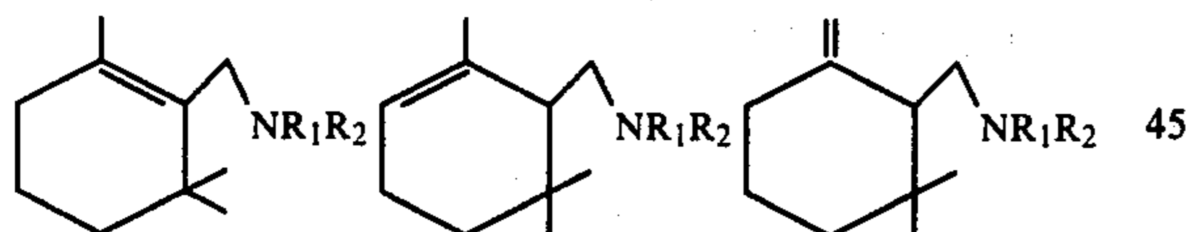
(I) Beta Isomer (II) Alpha Isomer (III) Gamma Isomer
