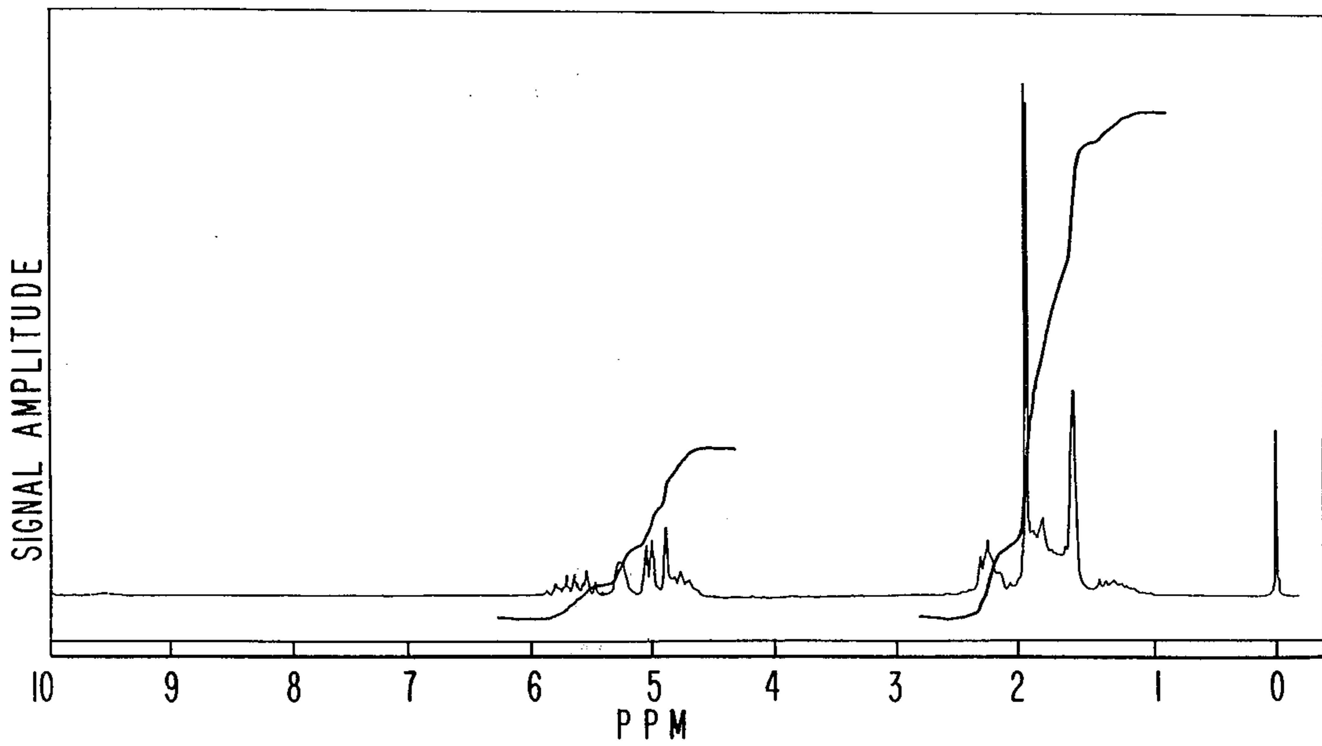
N M R SPECTRUM FOR EXAMPLE XXXIV .
