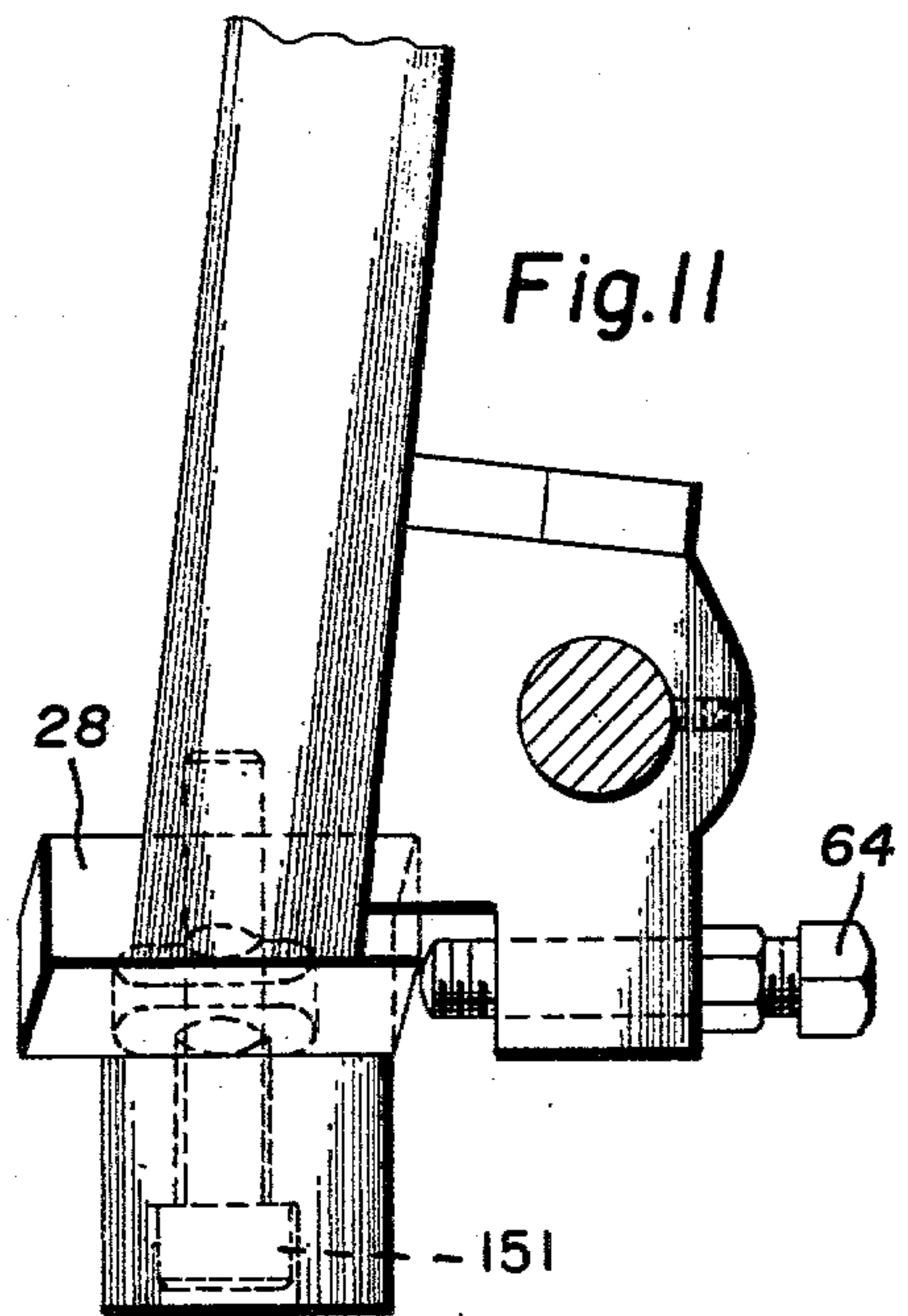
DETAIL 5 (FROM FIG. 5)
