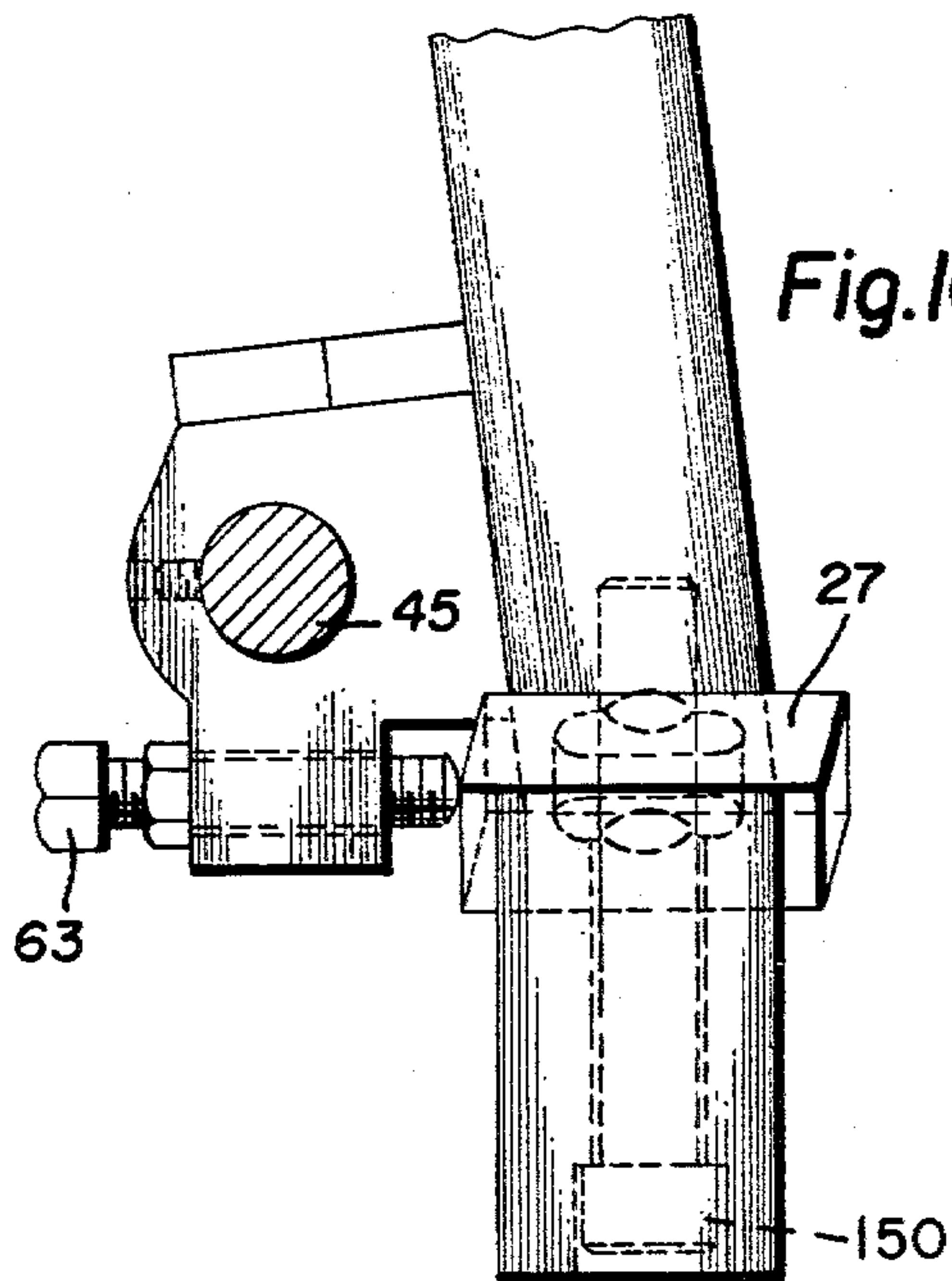
DETAIL 4 (FROM FIG. 5)
