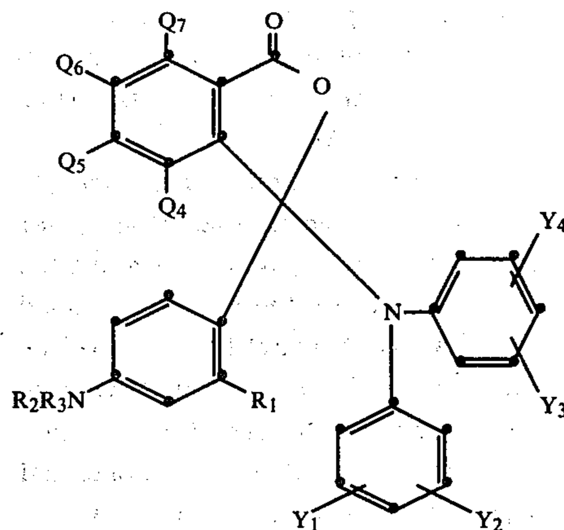
Formula II
