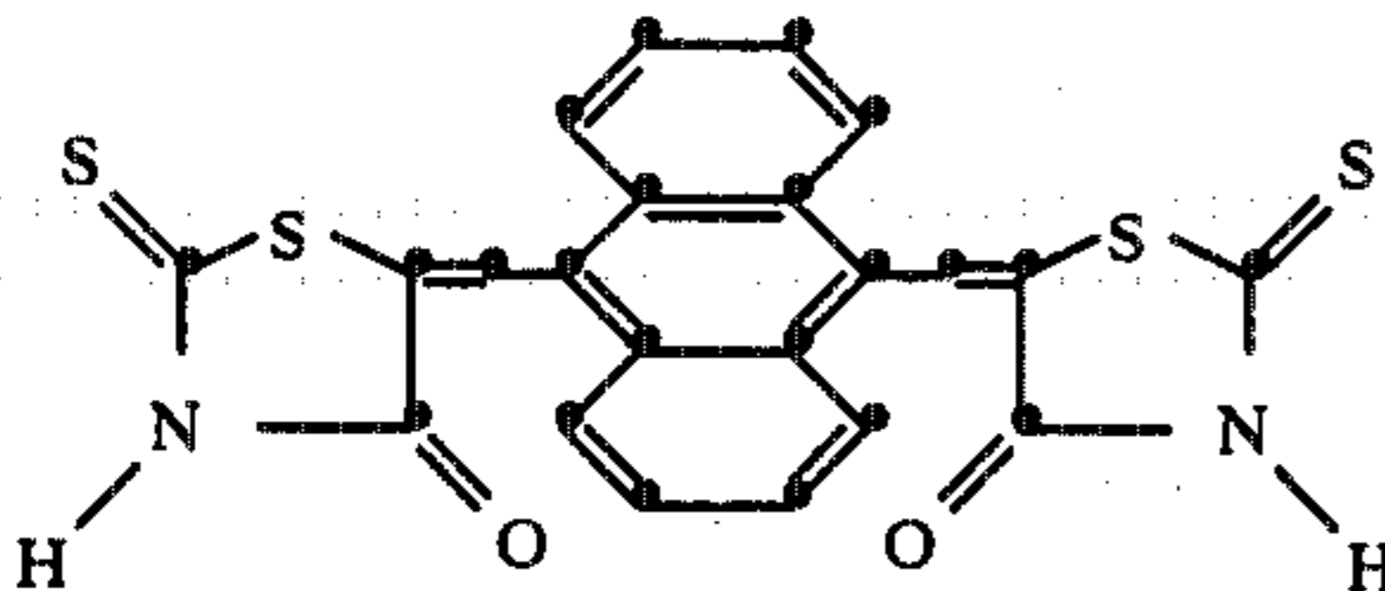
17. 4,4'-(1,4-phenylenedimethylidyne) bis(3-carbamoyl-1-phenyl pyrazolin-5-one)
