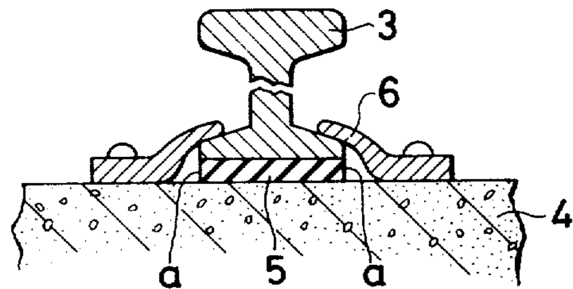
FIG. 3 PRIOR ART
