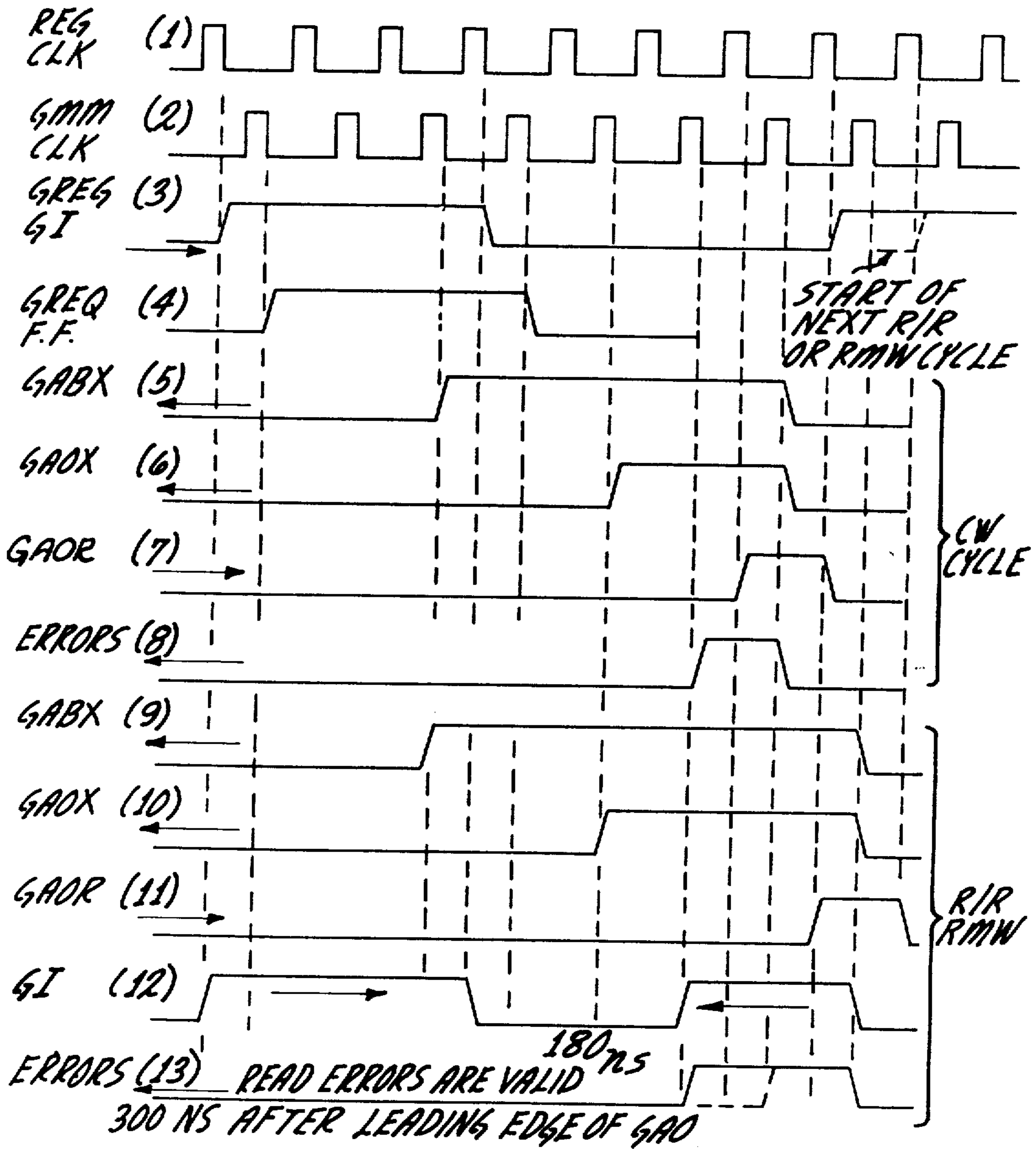
FIG. 20 TIMING RELATIONSHIPS
