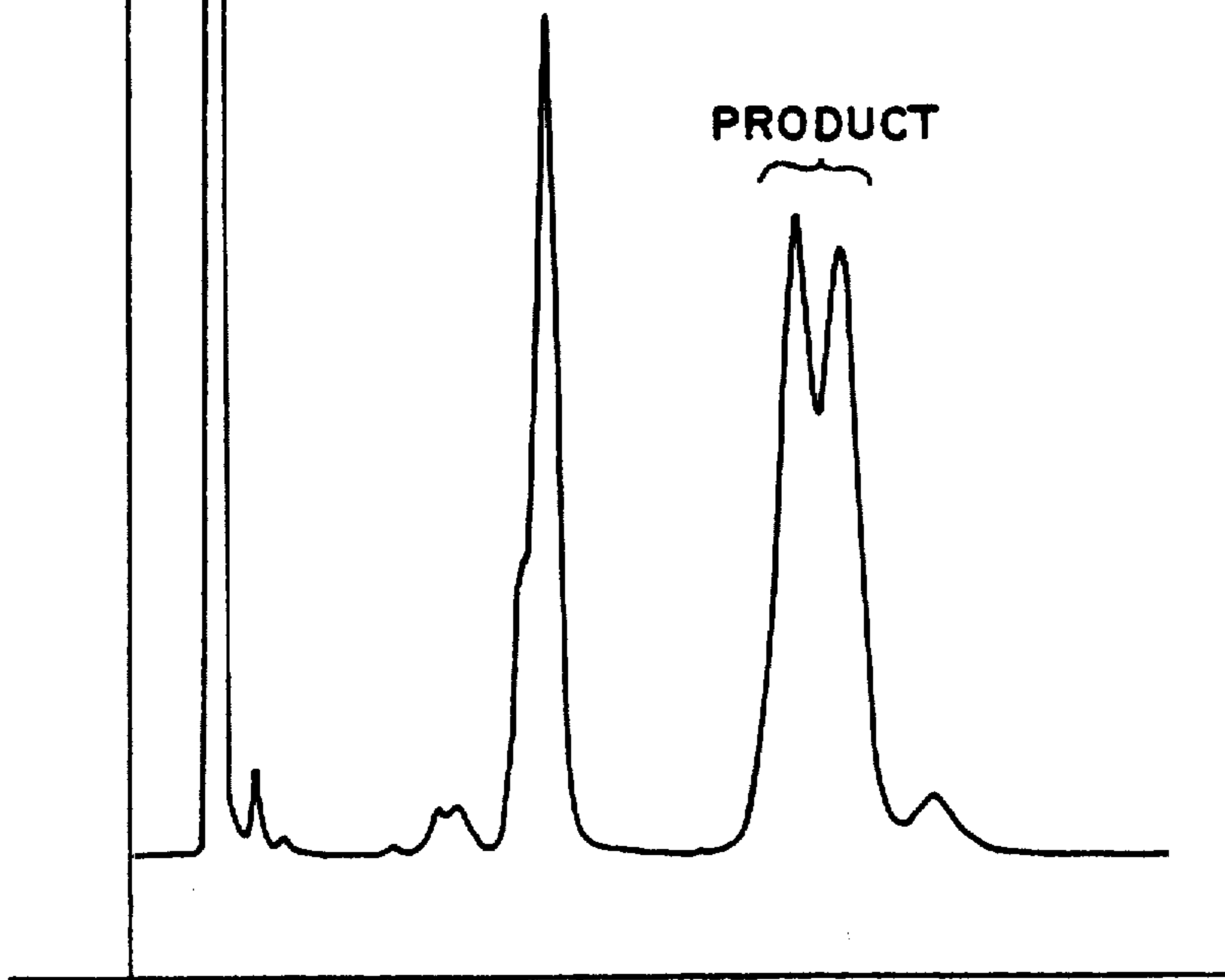
GLC PROFILE FOR EXAMPLE VII.
