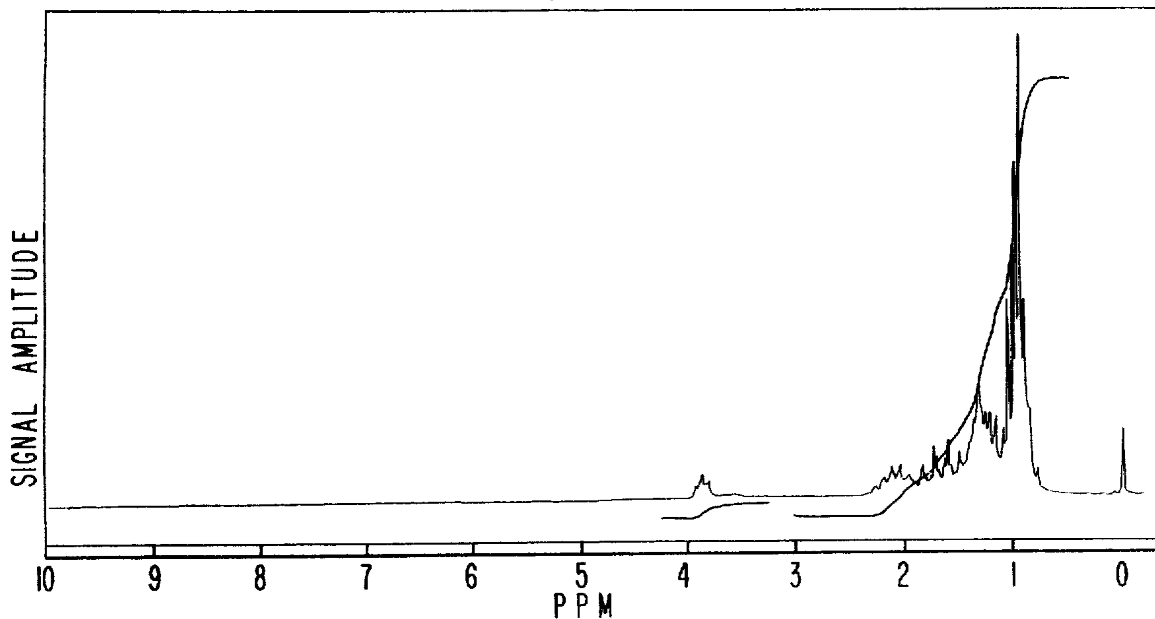
N M R SPECTRUM FOR EXAMPLE IV, FRACTION 10.
