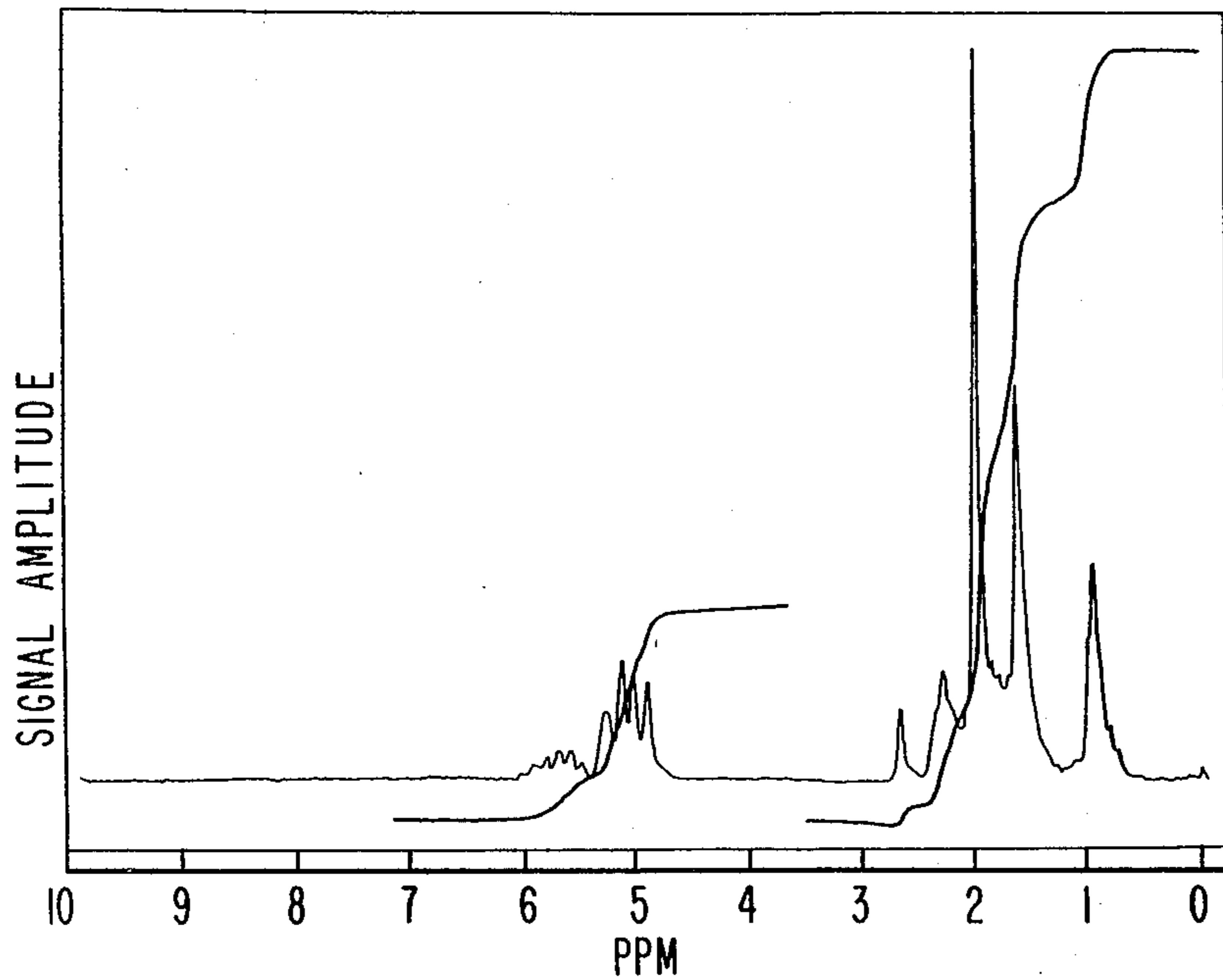
N M R SPECTRUM FOR EXAMPLE XXXII.
