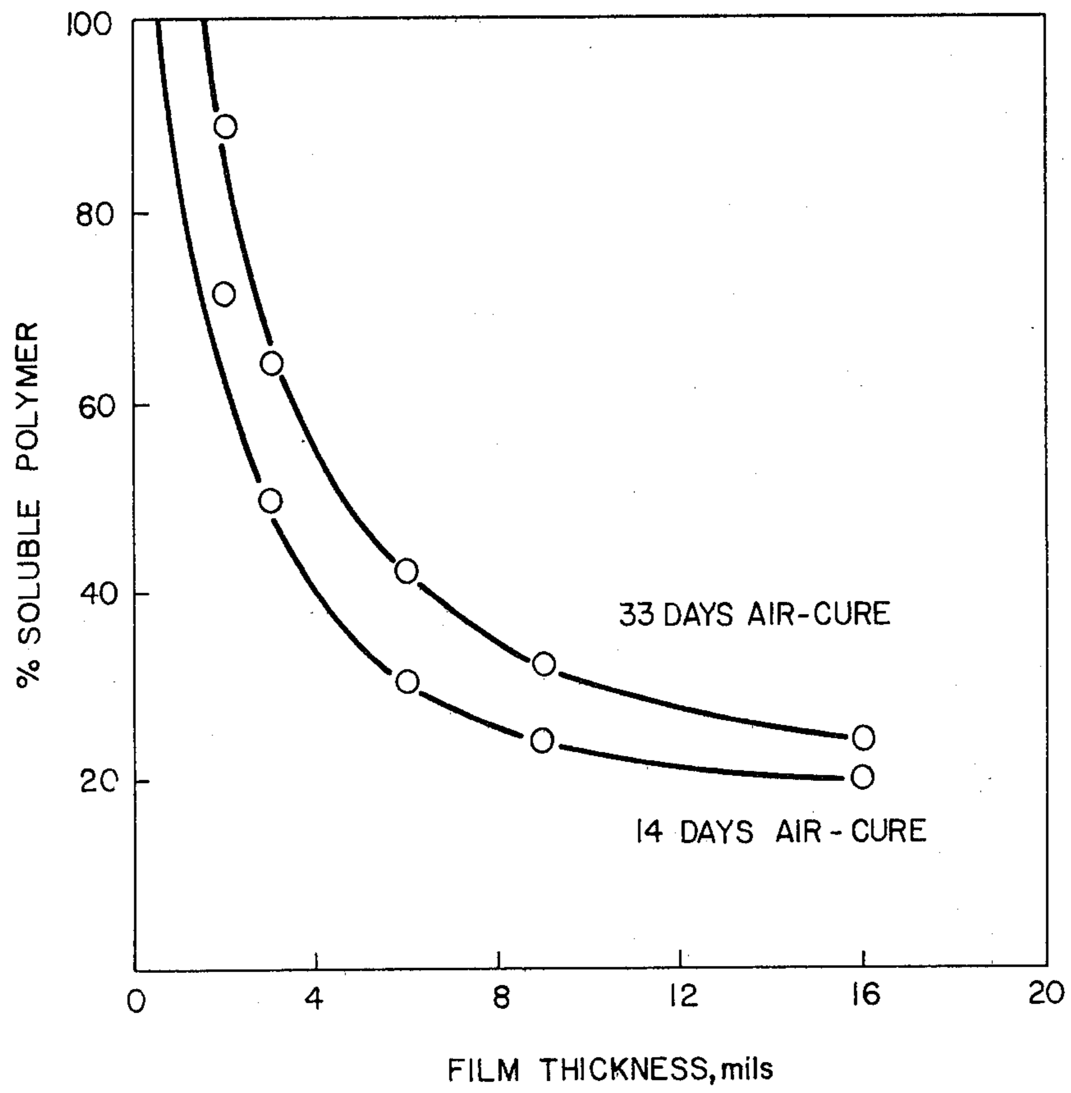
FIGURE 2 EFFECT OF FILM THICKNESS ON THROUGH-CURE
