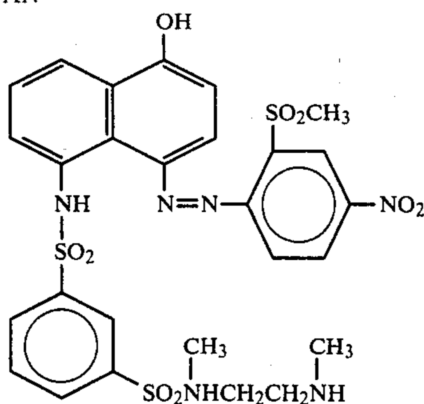
1-hydroxy-5-{m[2-(n-methyl amino)ethyl-n-methyl sulfamyl]-phenyl sulfamoylamido}-4-{[2-(methyl sulfonyl)-4-nitrophenyl]azo}-naphthalene.
