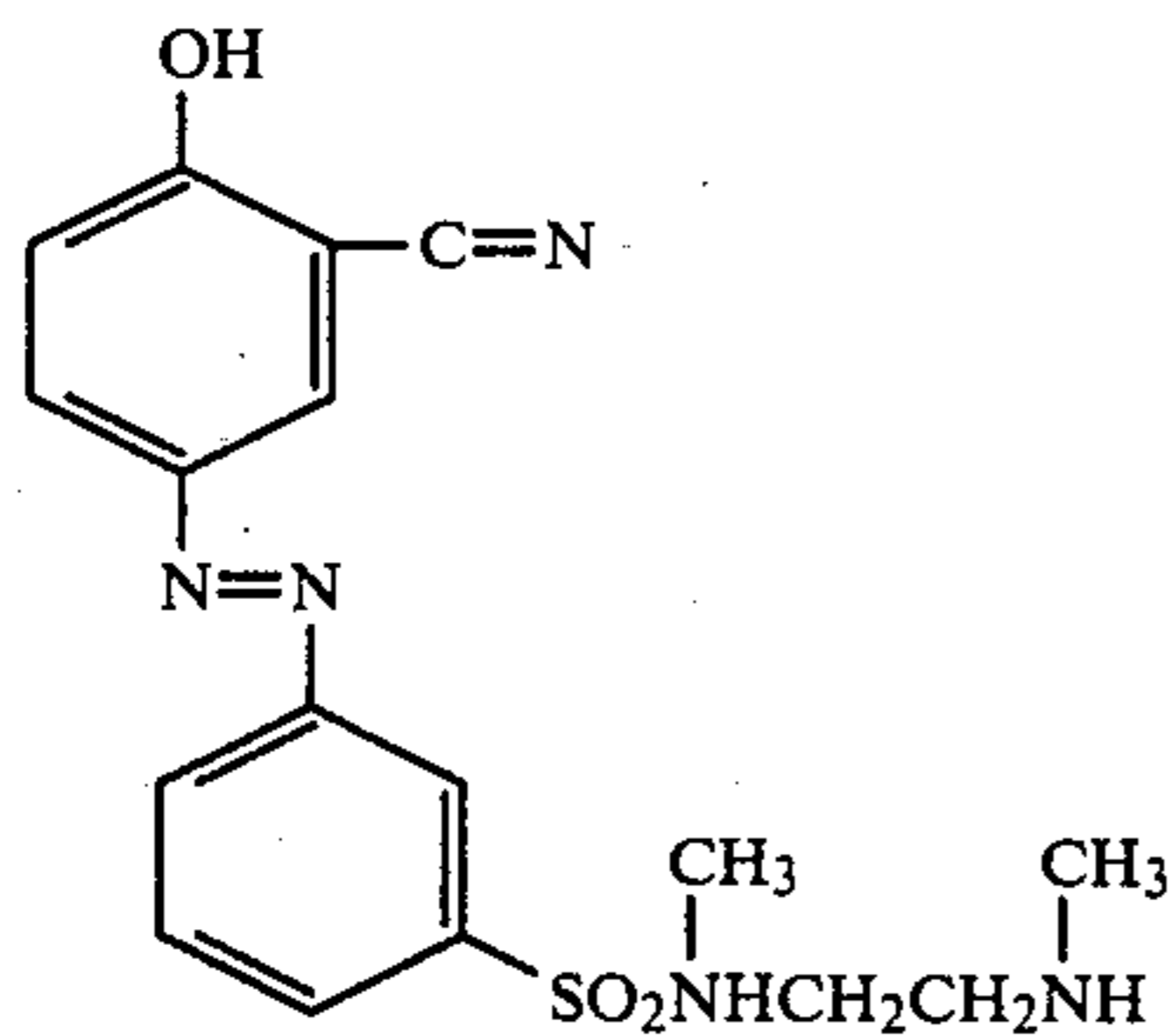
2-cyano-4-{m[2-(n-methyl amino)ethyl-n-methyl sulfamyl]-phenyl}azo phenol.
