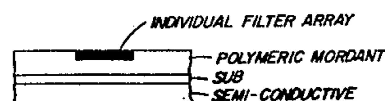
AFTER STRIPPING RESIST
