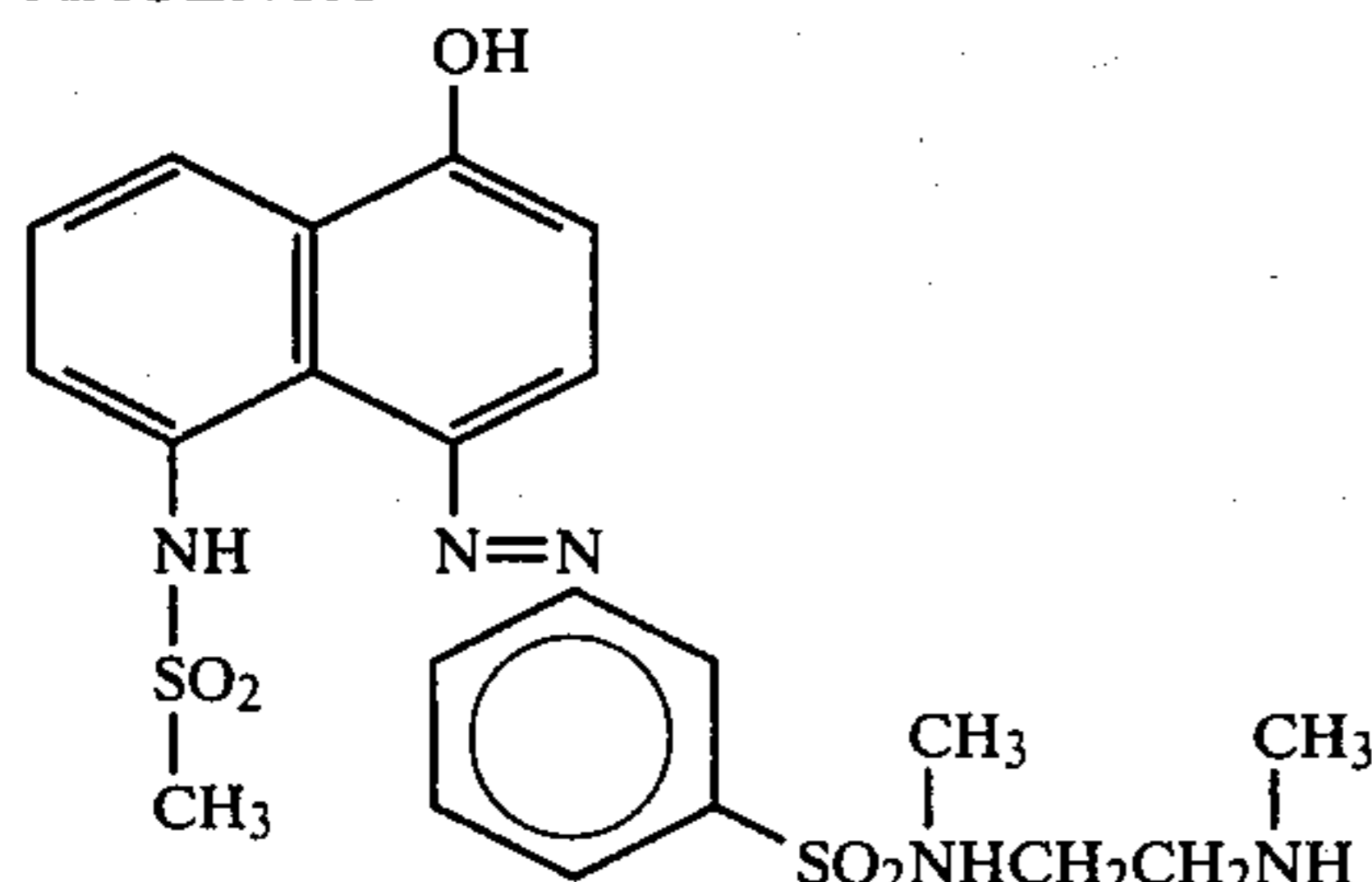
1-hydroxy-5-methylsulfamyl-4-{m[2-(n-methyl amino)ethyl-n-methyl sulfamyl phenyl]azo}-naphthalene.
