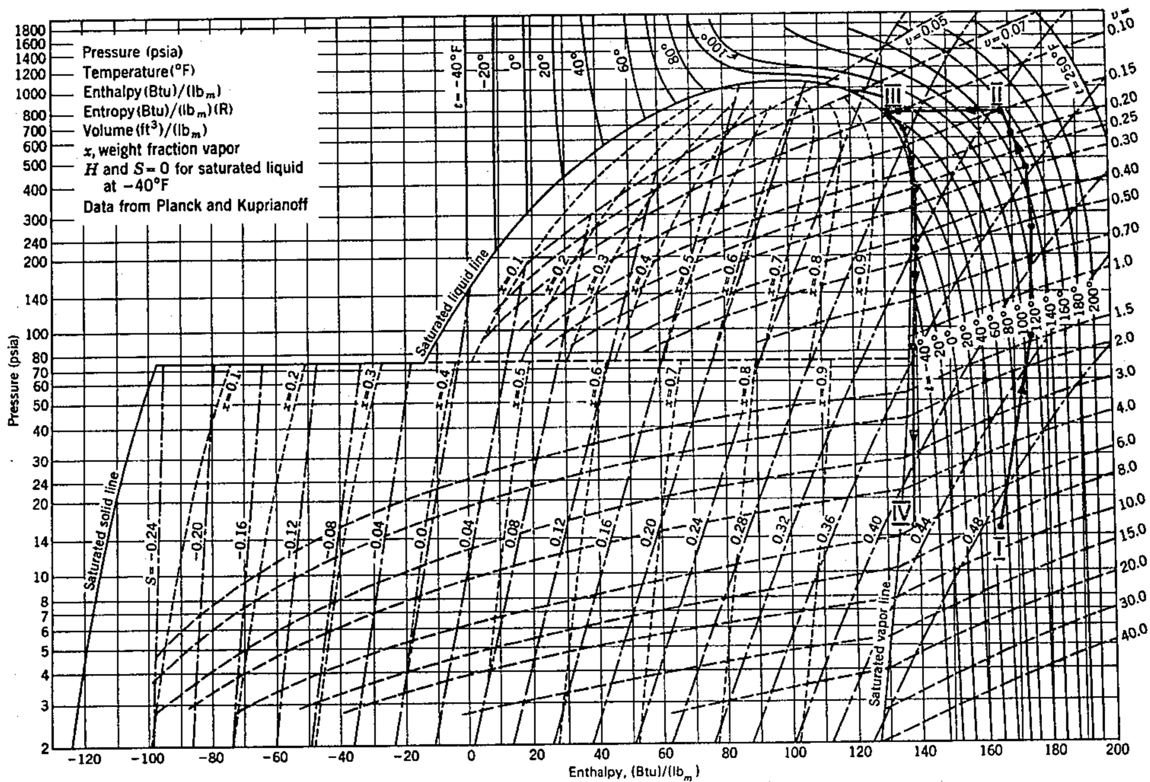
Pressure-enthalpy diagram for carbon dioxide.
