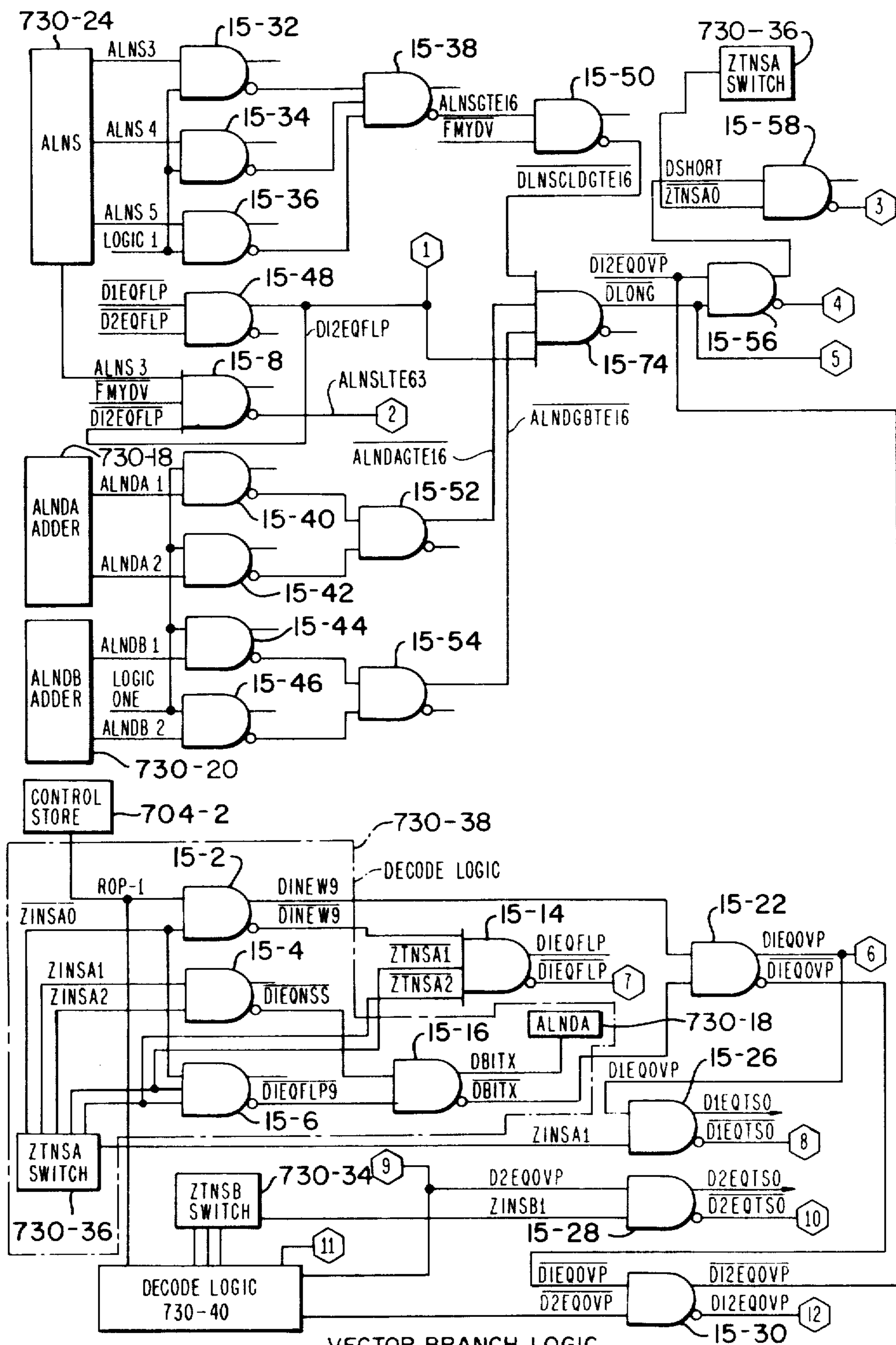
VECTOR BRANCH LOGIC FIG. 8 SHEET 1 OF 2
