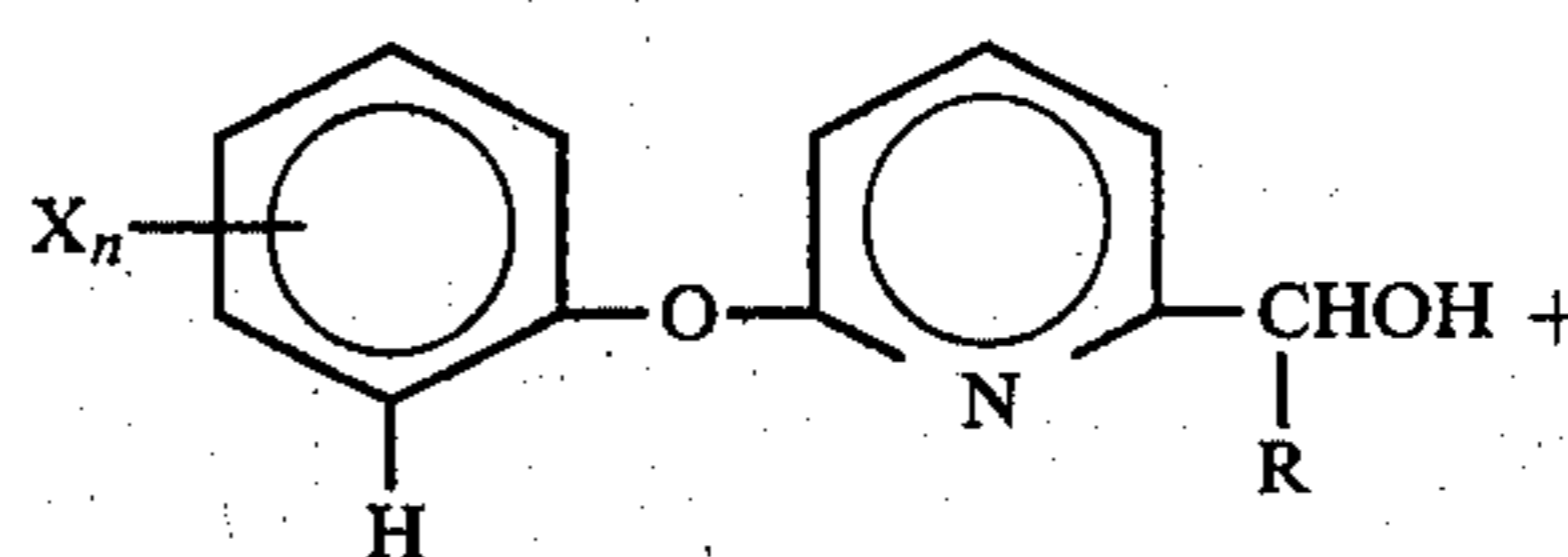
(Formula II)
