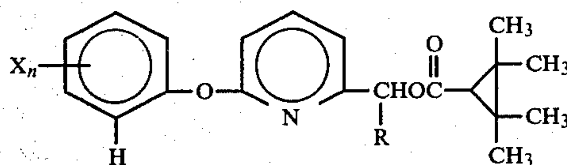
(Formula I)
