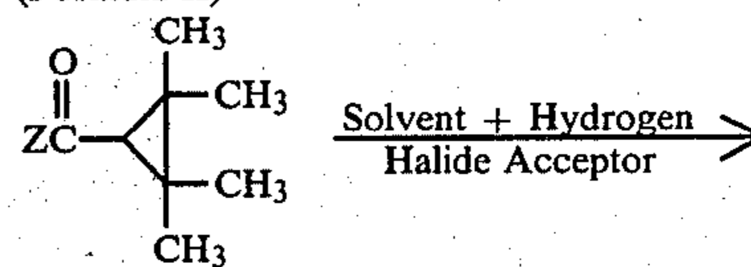
(Formula III)
