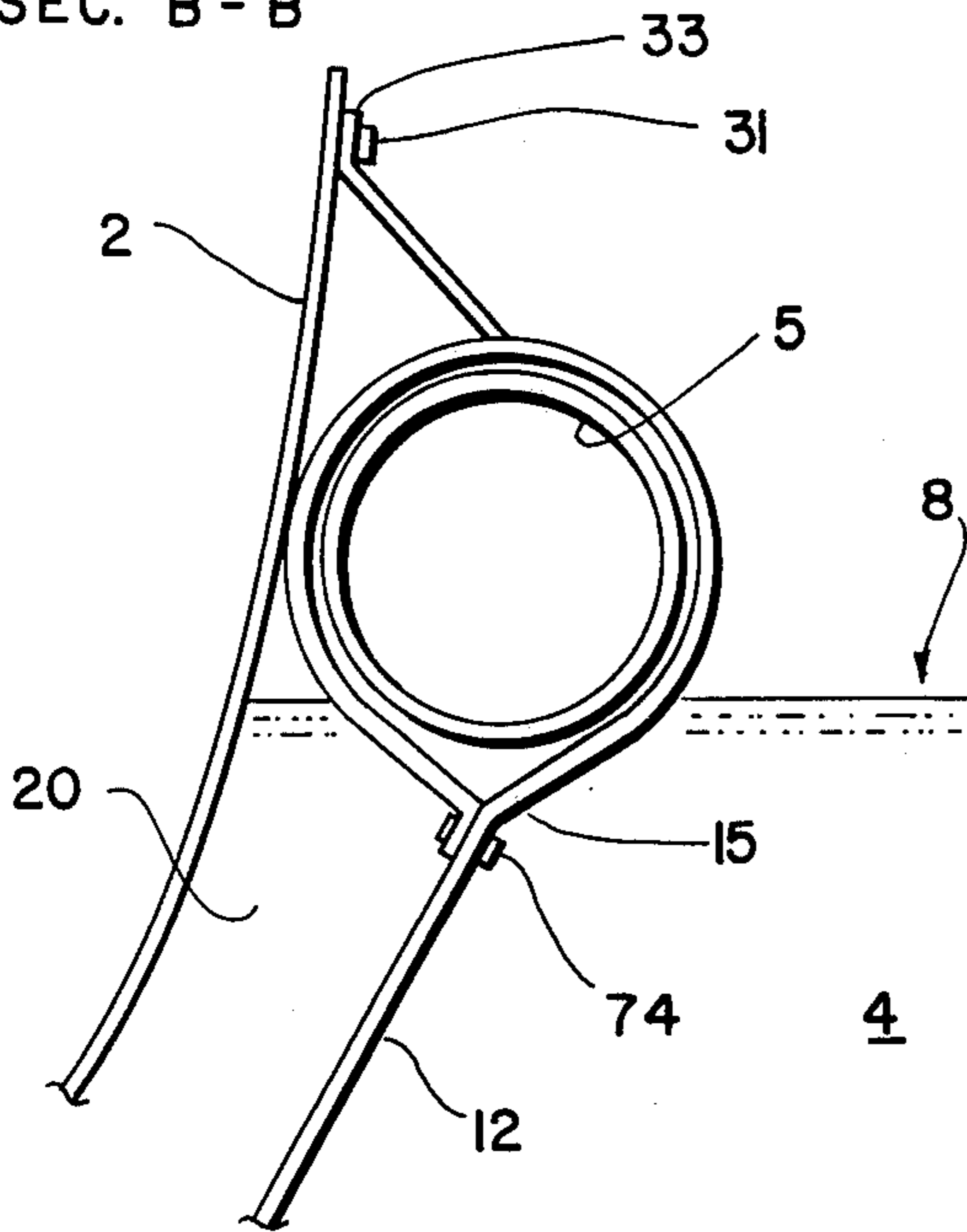
FIG. 6 SEC. B - B'
