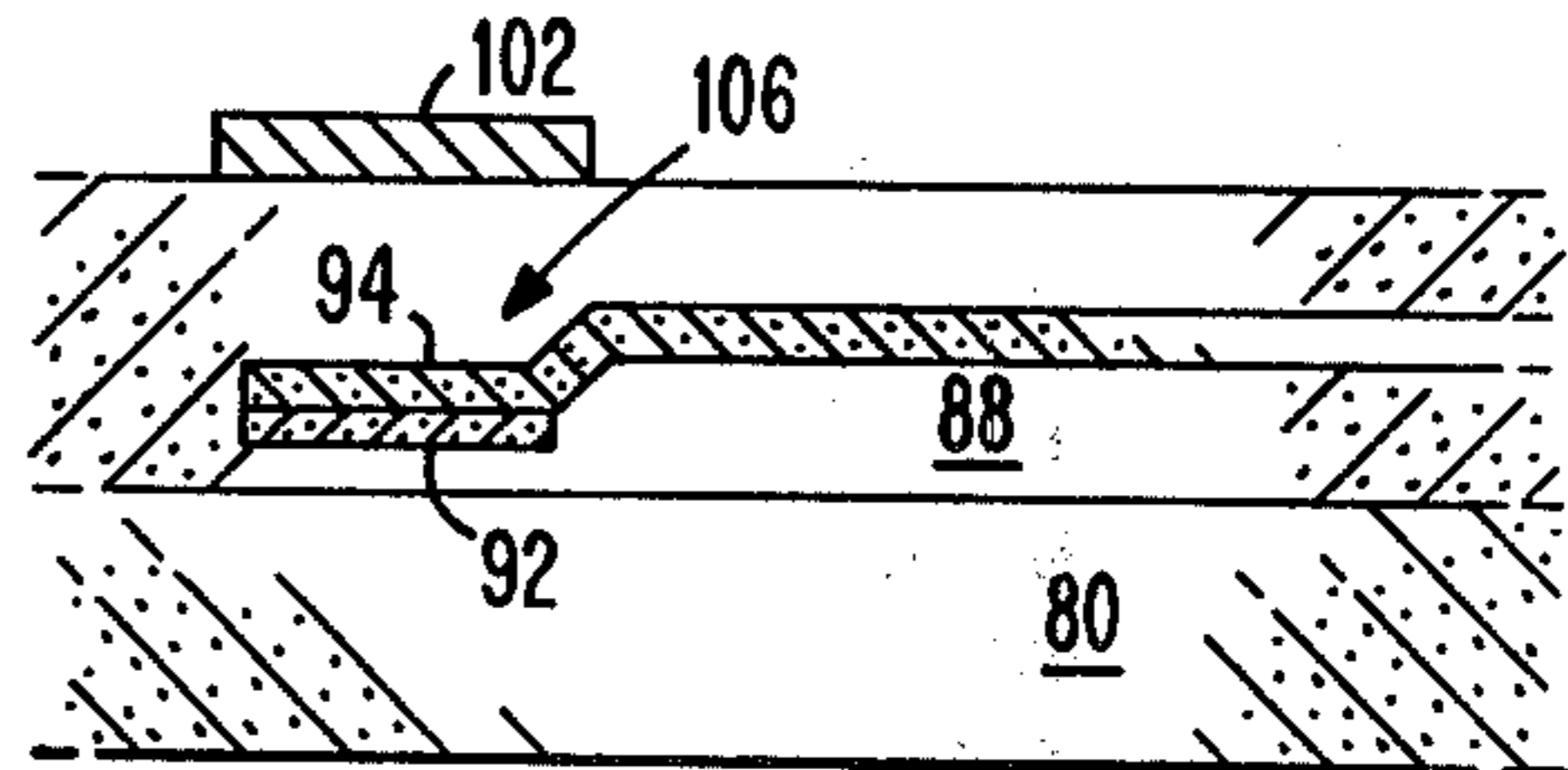
SECTION E-E'
