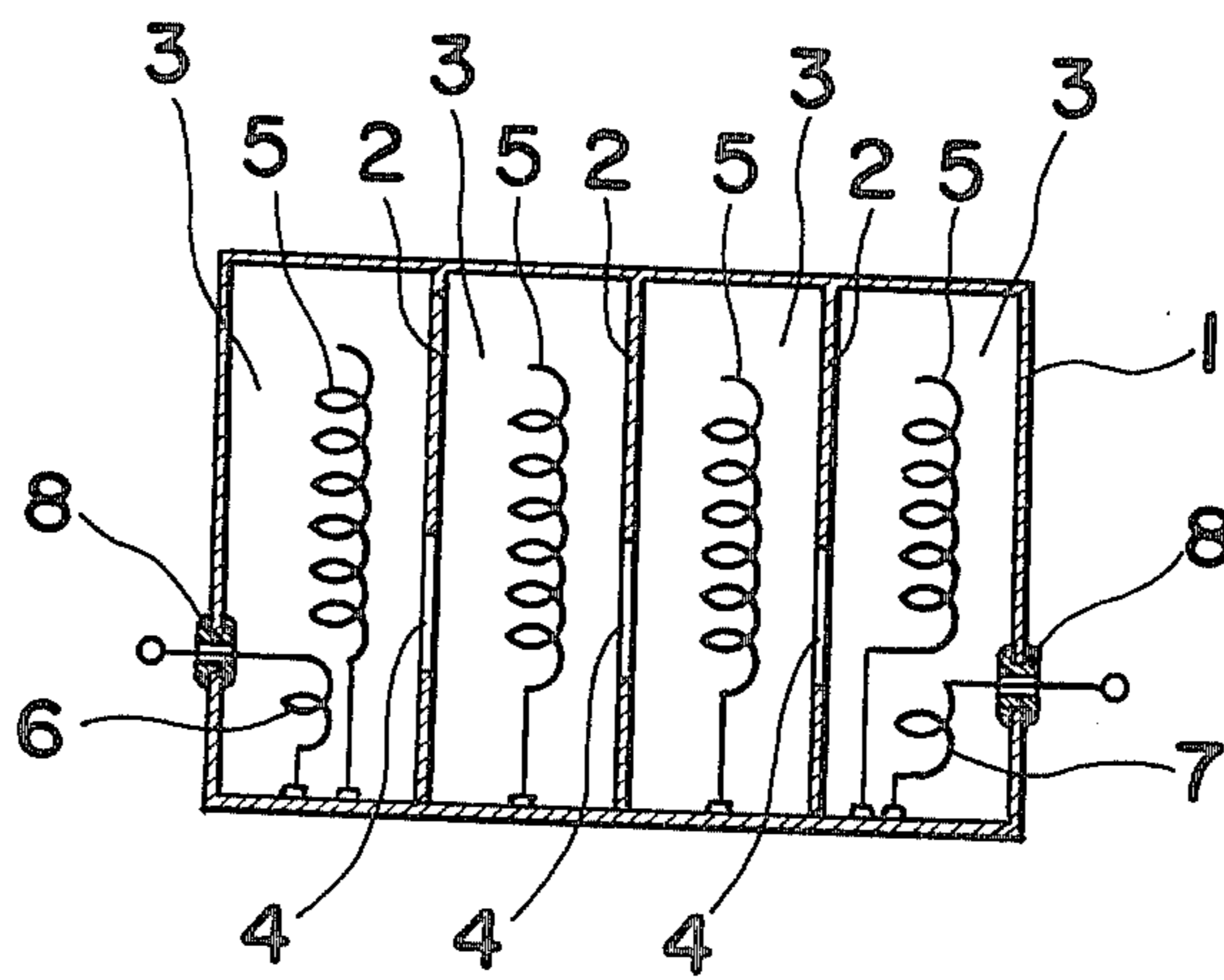
Fig. 3 PRIOR ART
