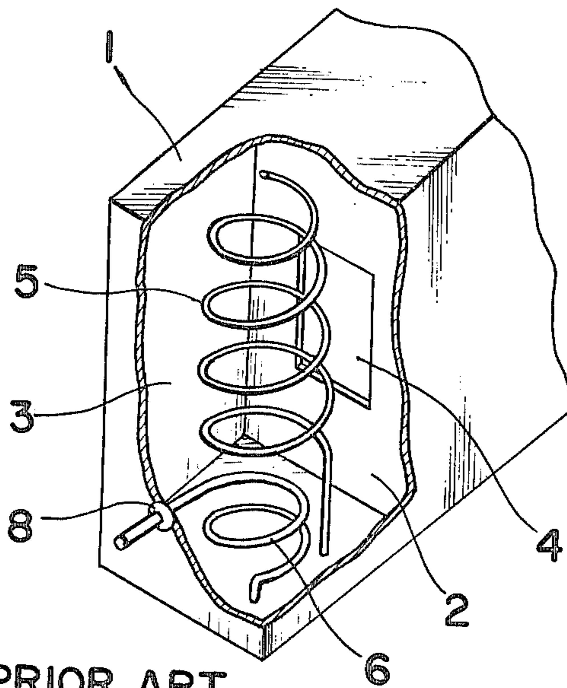
Fig. 1 PRIOR ART
