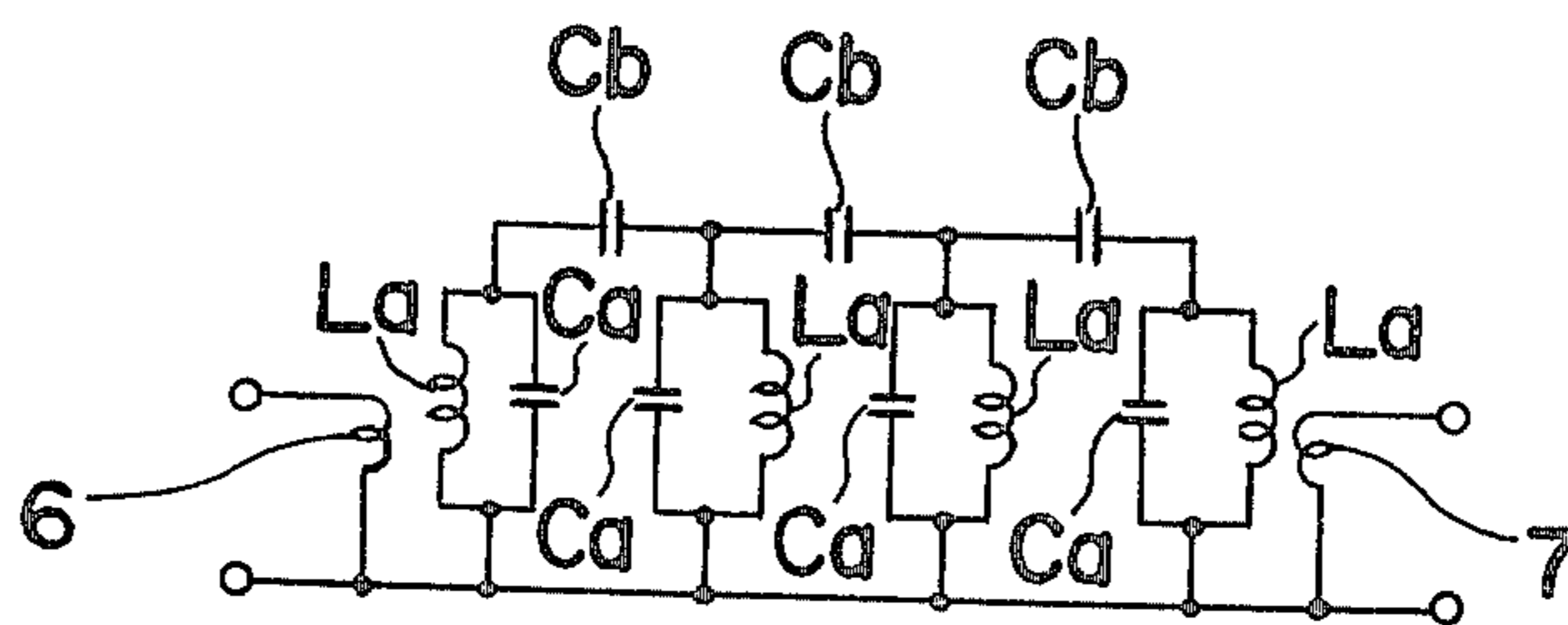
Fig. 3 PRIOR ART
