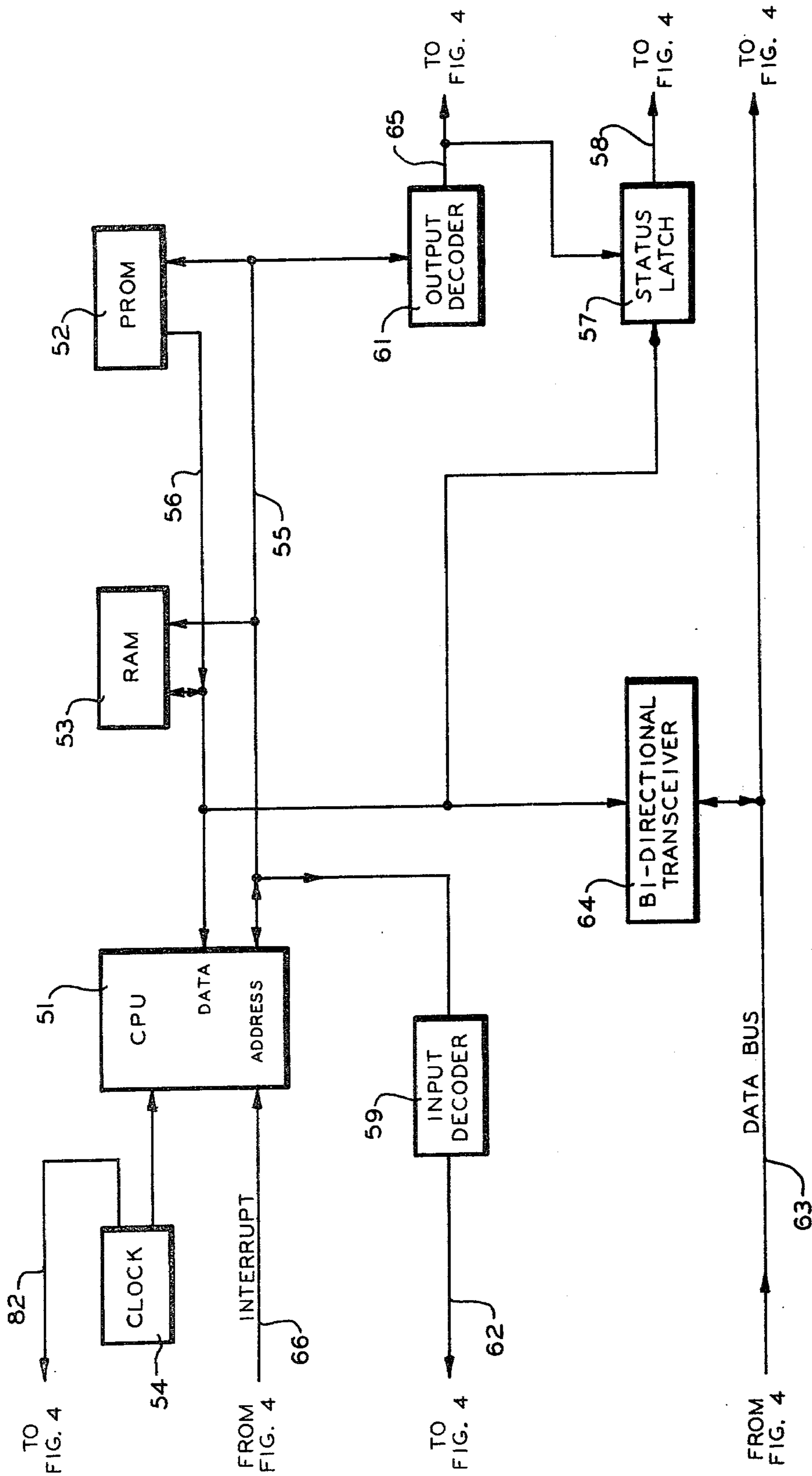
COMPUTER CIRCUIT 29
