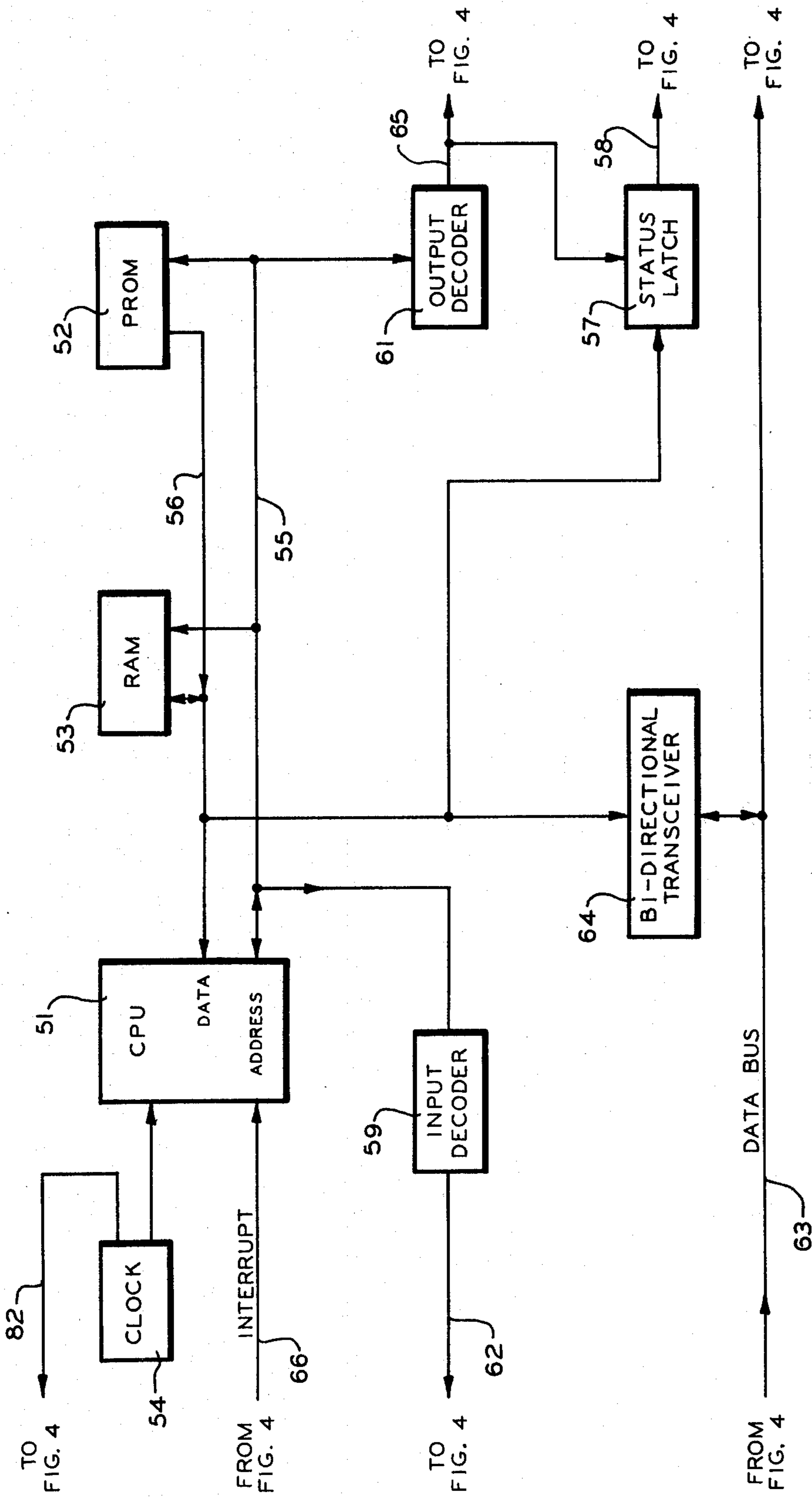
COMPUTER CIRCUIT 29
