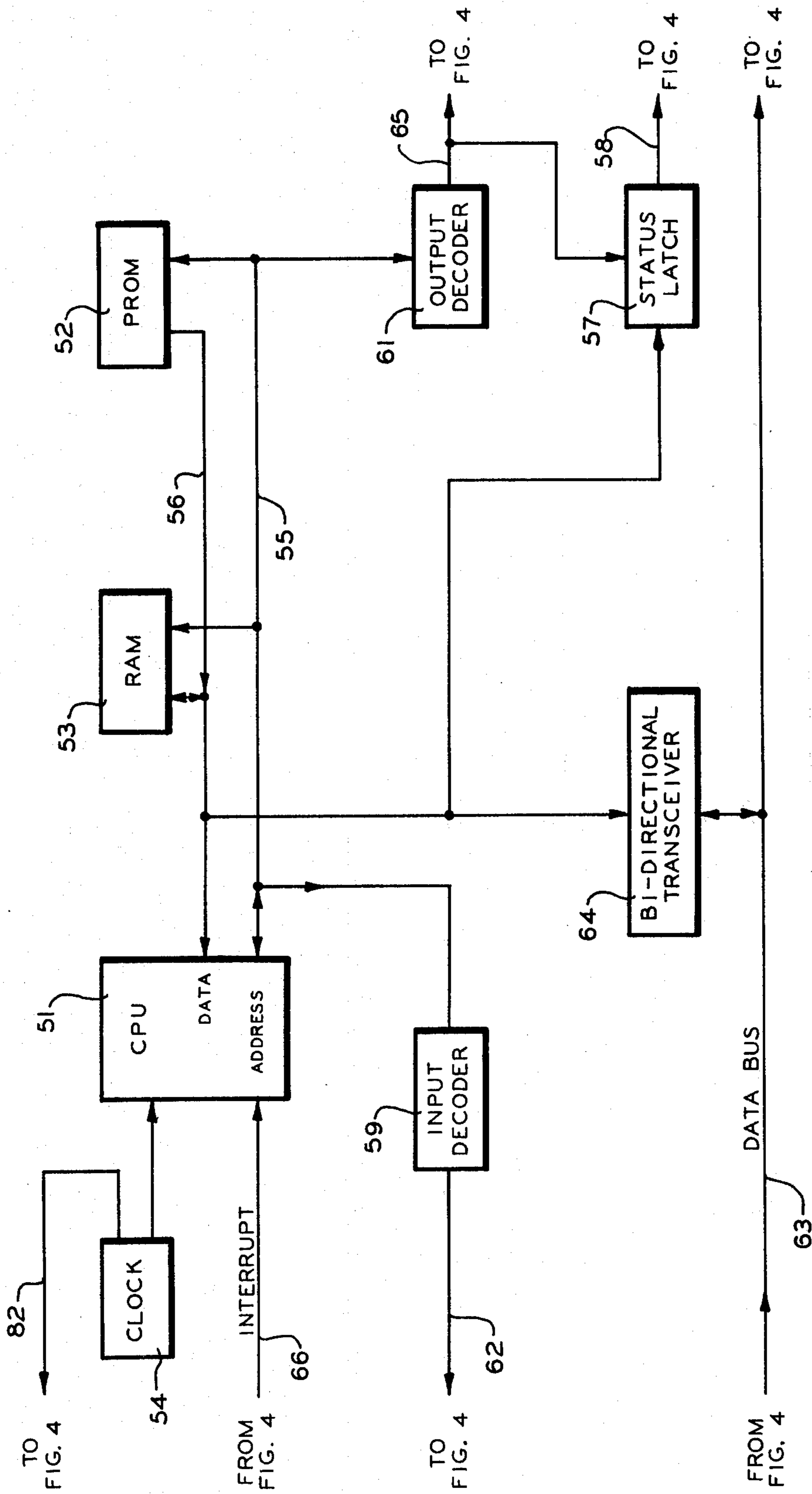
COMPUTER CIRCUIT 29
