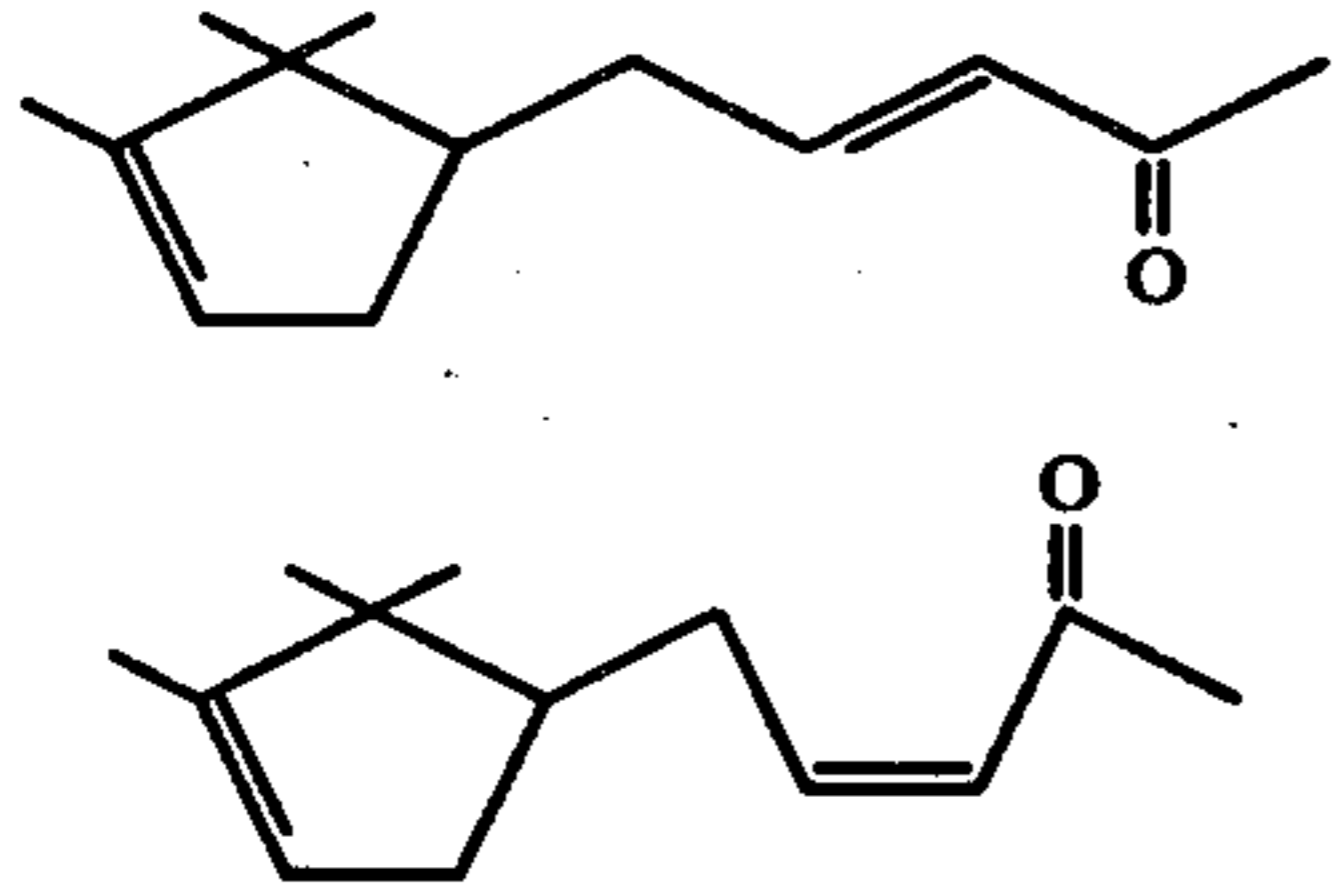
FIG. 32 is the NMR spectrum for peak "A" of the reaction product produced according to Example IIIB containing compounds having the structures:
