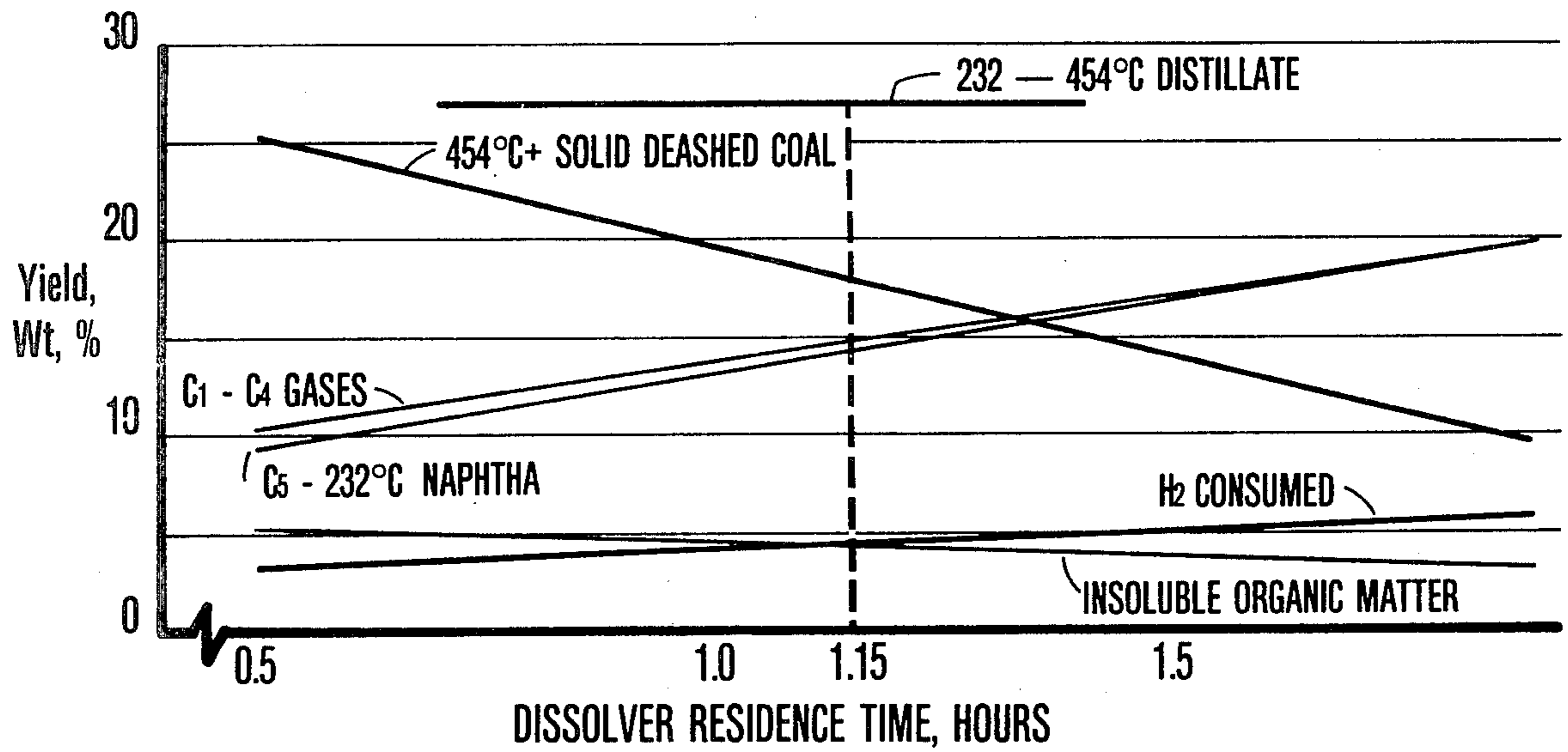
FIGURE 2 COUPLED COAL LIQUEFACTION- GASIFICATION PROCESS
