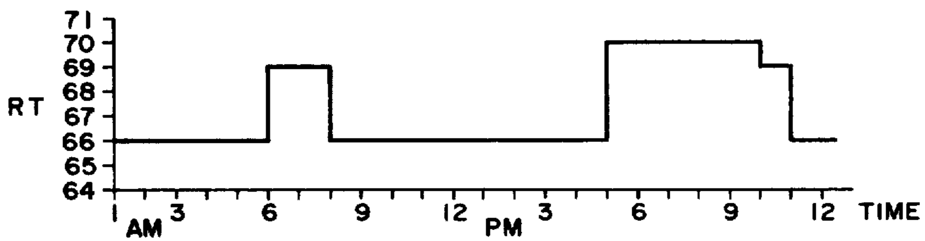
FIGURE 2C HEATING (OCCUPANTS NOT HOME DURING DAY)
