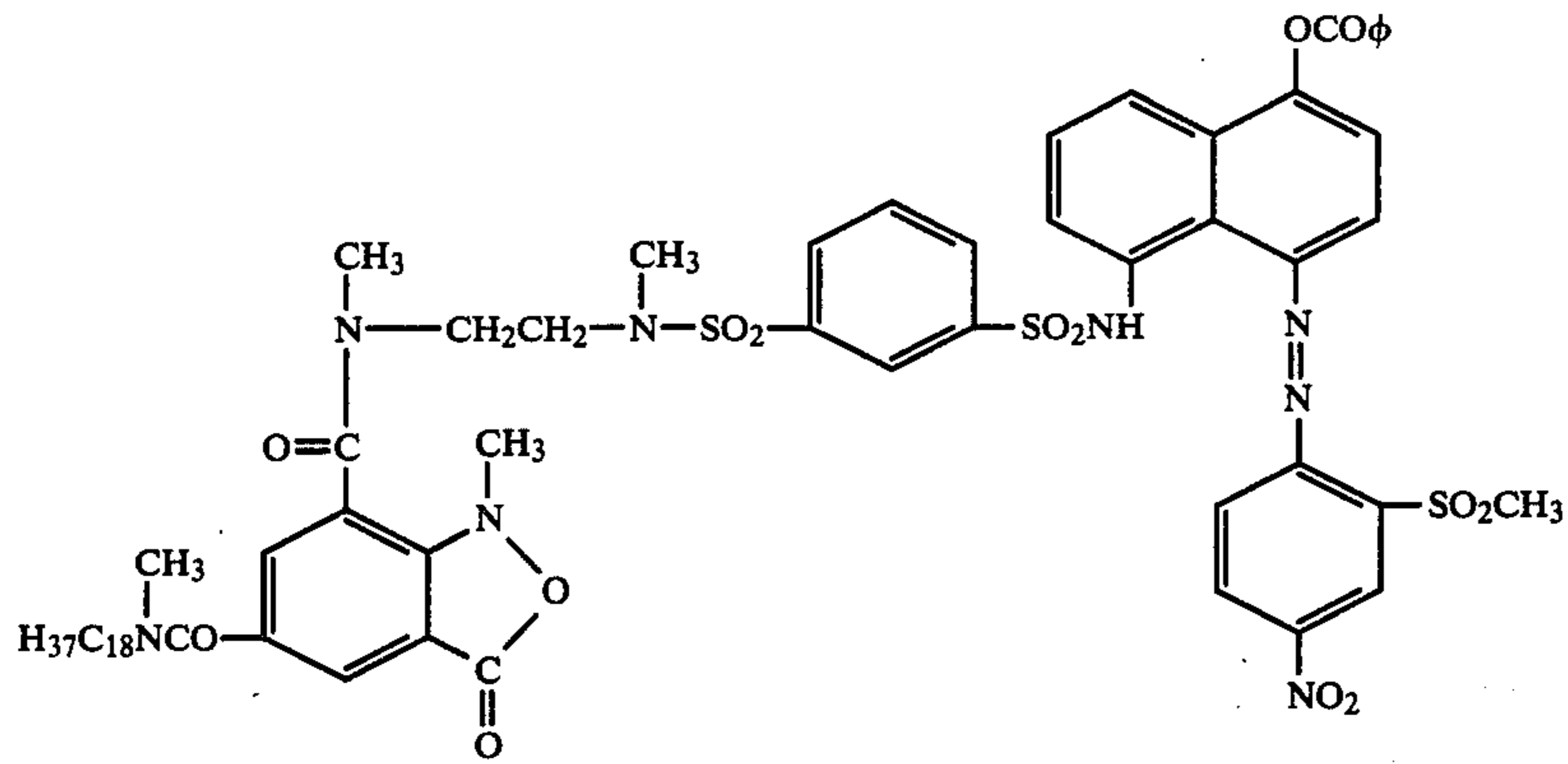
Compound VI
