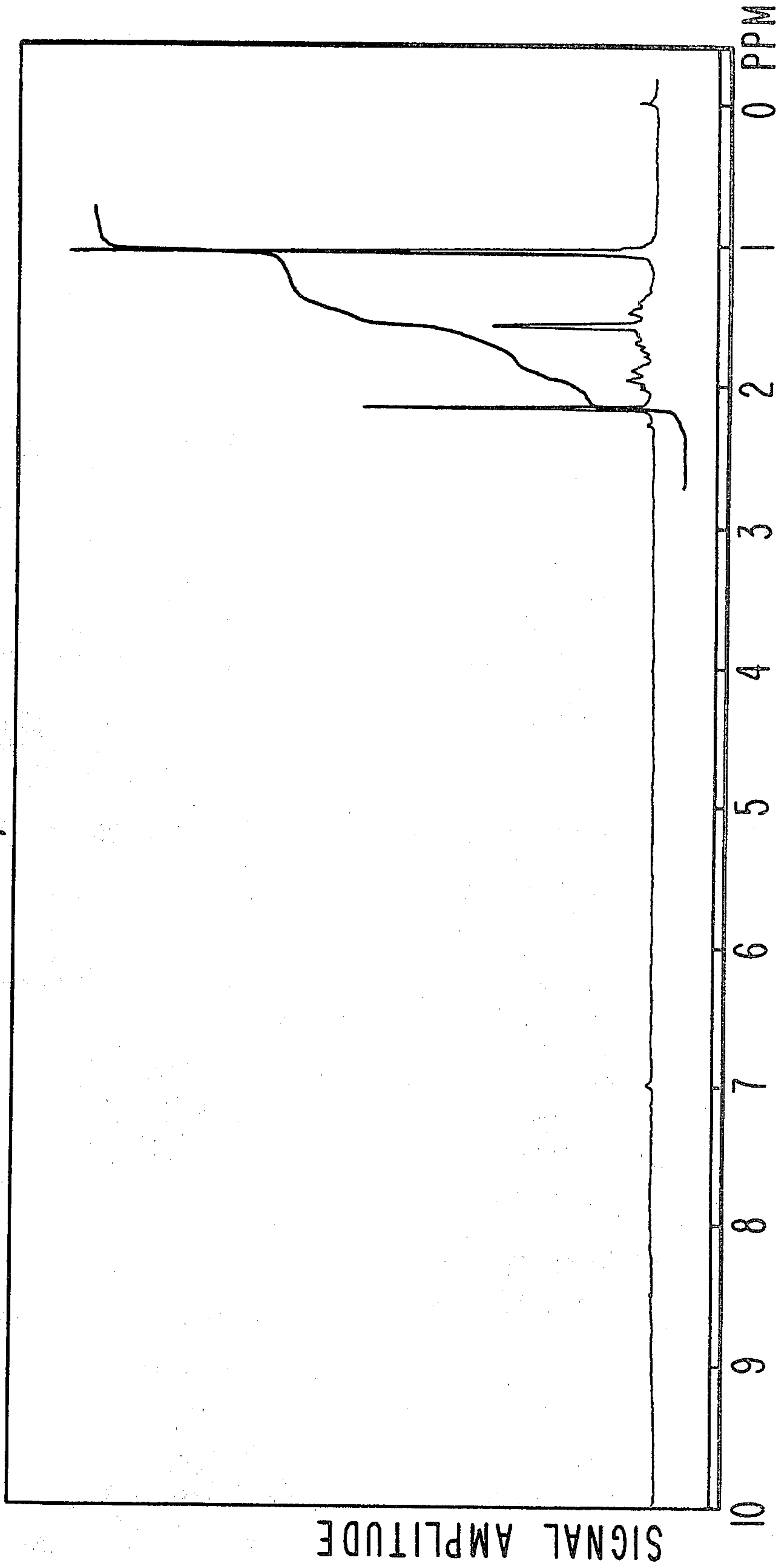
N M R SPECTRUM FOR EXAMPLE I , PEAK 3.
