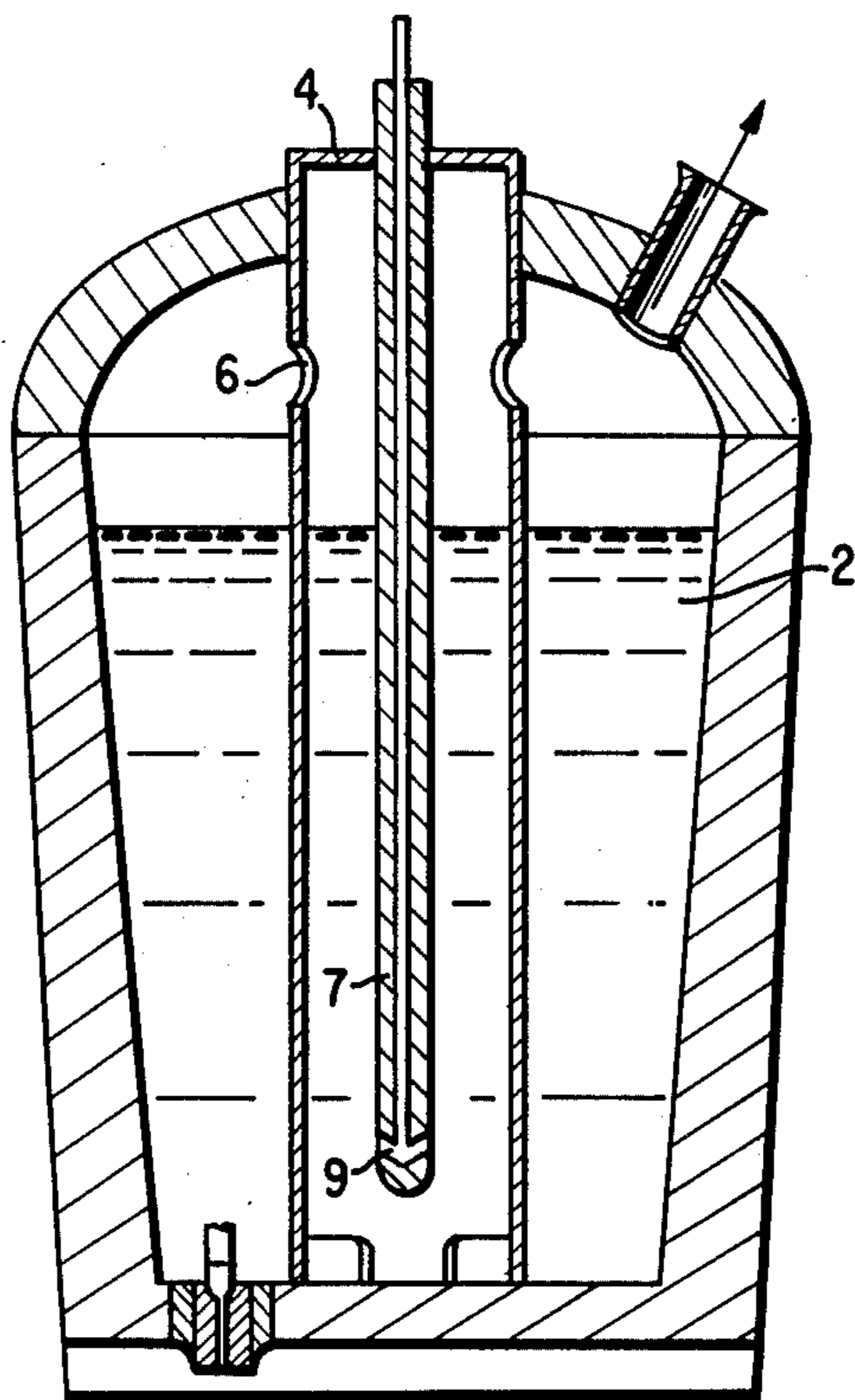
FIG. 1 (PRIOR ART)
