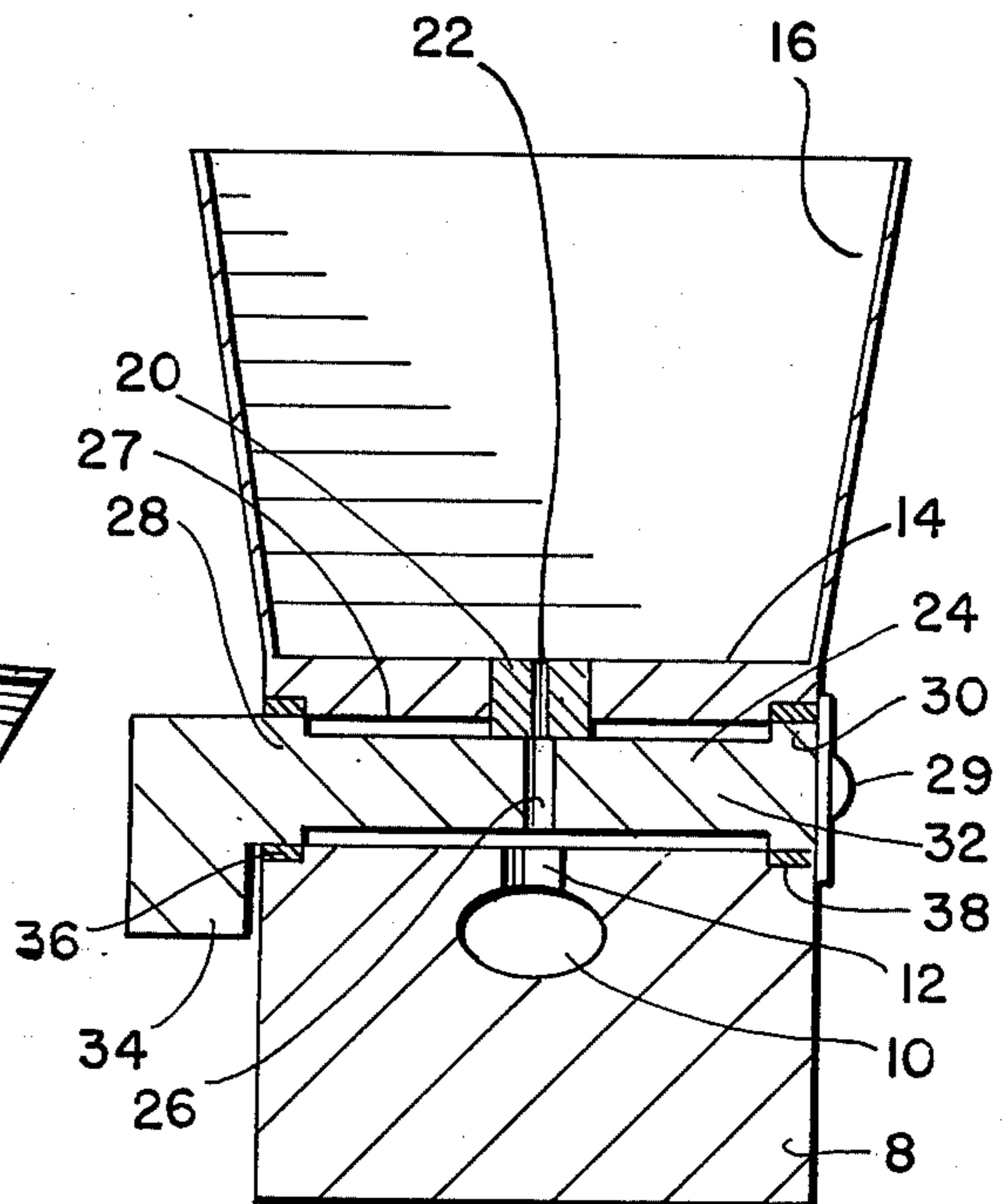
FIG. 3 SEC. B-B'
