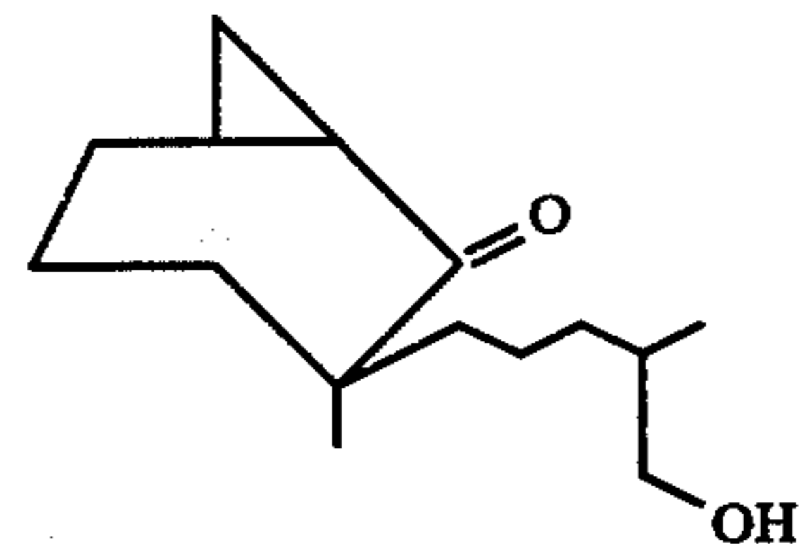
dihydro- \beta -santalol
