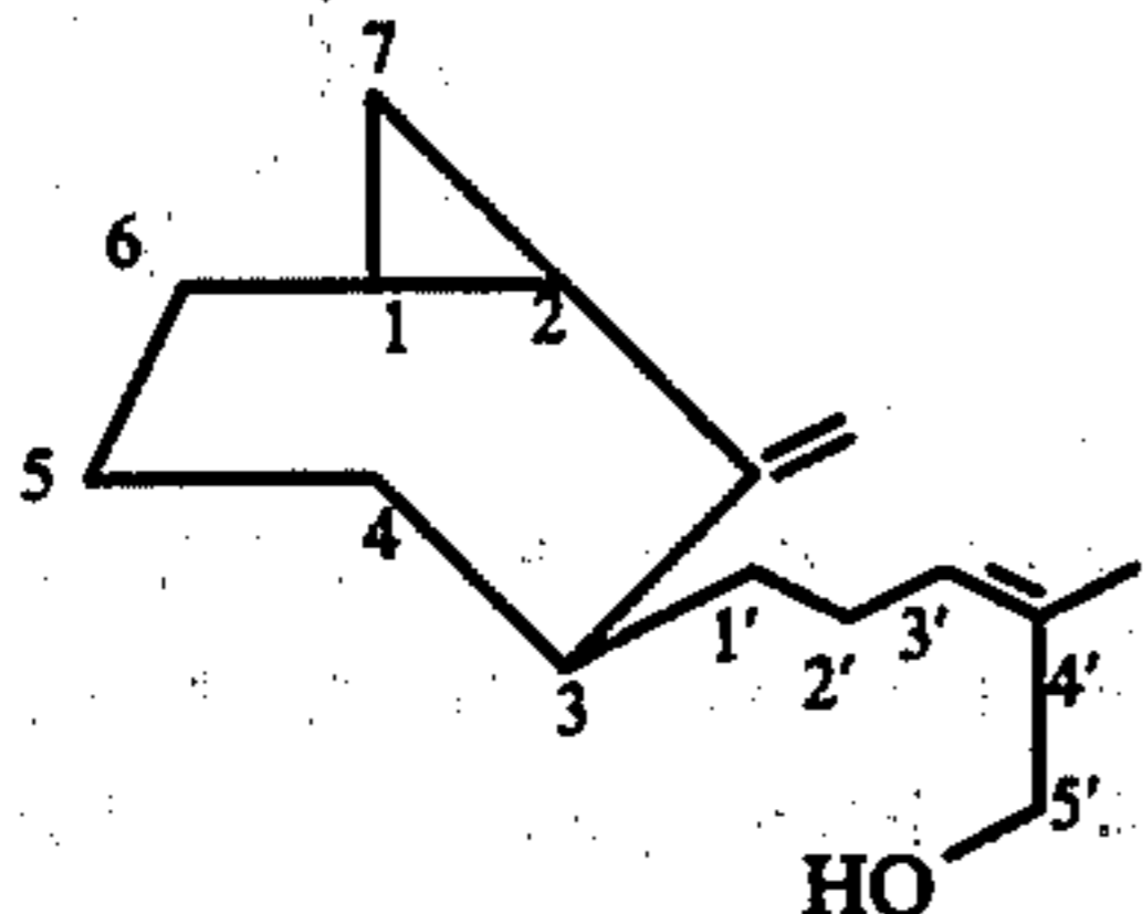
2-methylene-3-exo(cis-4'-methyl-5'-hydroxypent-3'-enyl)bicyclo[2.2.1]-heptane cis-3-normethyl- \beta -santalol
