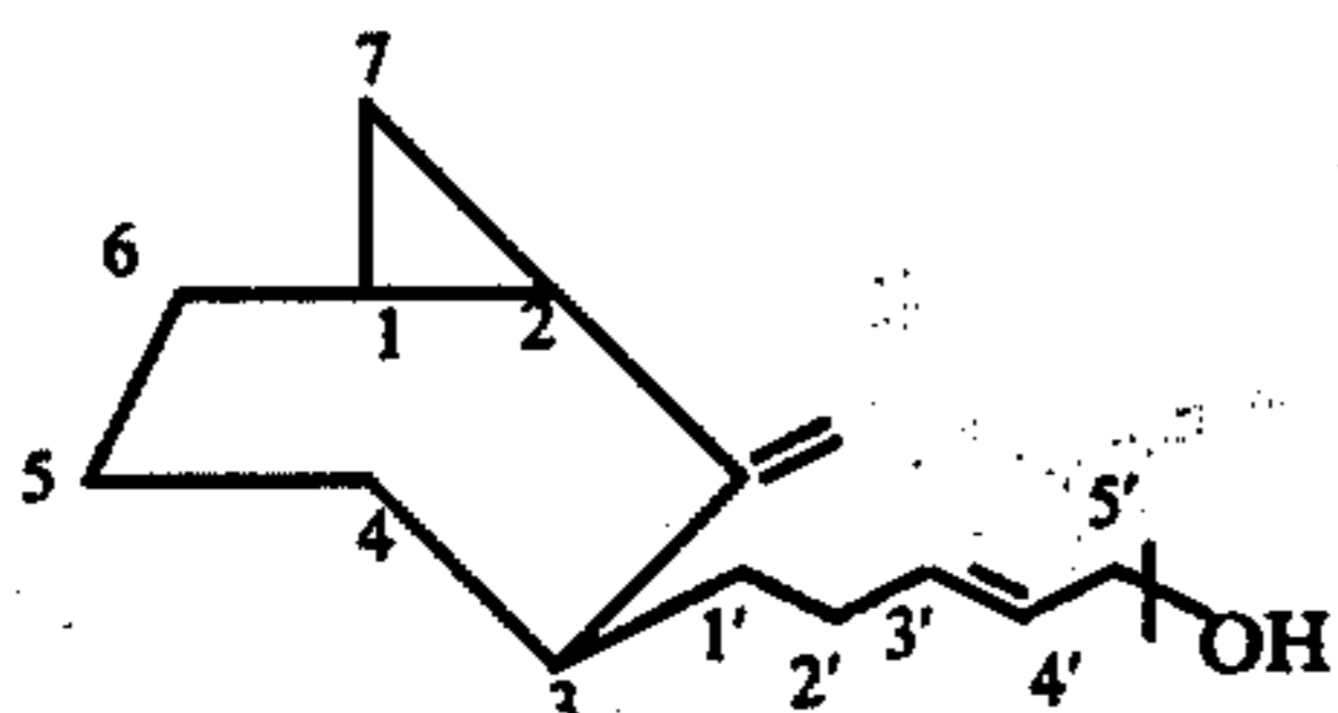
2-methylene-3-exo(trans-4'-methyl-5'-hydroxypent-3'-enyl)bicyclo[2.2.1]-heptane trans-3-Normethyl- \beta -santalol
