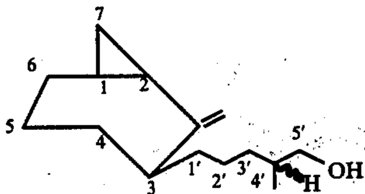
2-methylene-3-exo(4'-methyl-5'-hydroxypentyl)-bicyclo[2.2.1]-heptane
