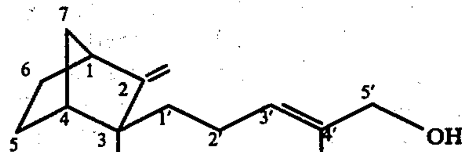
endo-3-methyl-exo-3(trans-5'-hydroxy-4'-methylpent-3'-enyl)-2-methylenebicyclo[2.2.1]heptane
