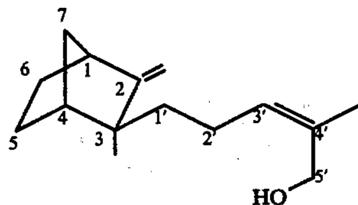
endo-3-methyl-exo-3(cis-5'-hydroxy-4'-methylpent-3'-enyl)-2-methylenebicyclo[2.2.1]heptane
