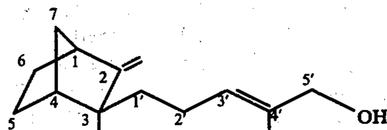
endo-3-methyl-exo-3(trans-5'-hydroxy-4'-methylpent-3'-enyl)-2-methylenebicyclo[2.2.1]heptane
