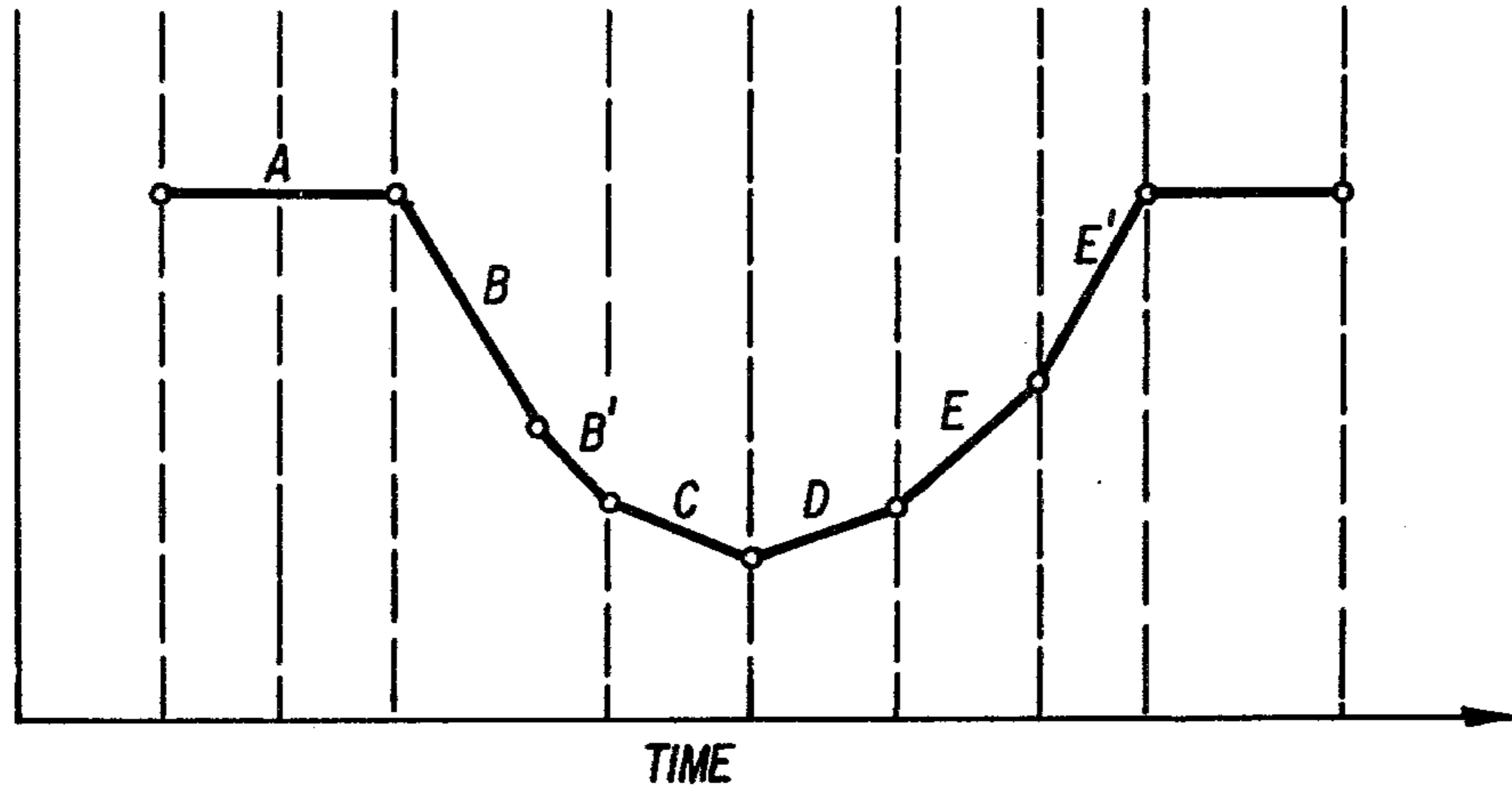
FIG. 2(a) UPPER PLATEN DISPLACEMENT
