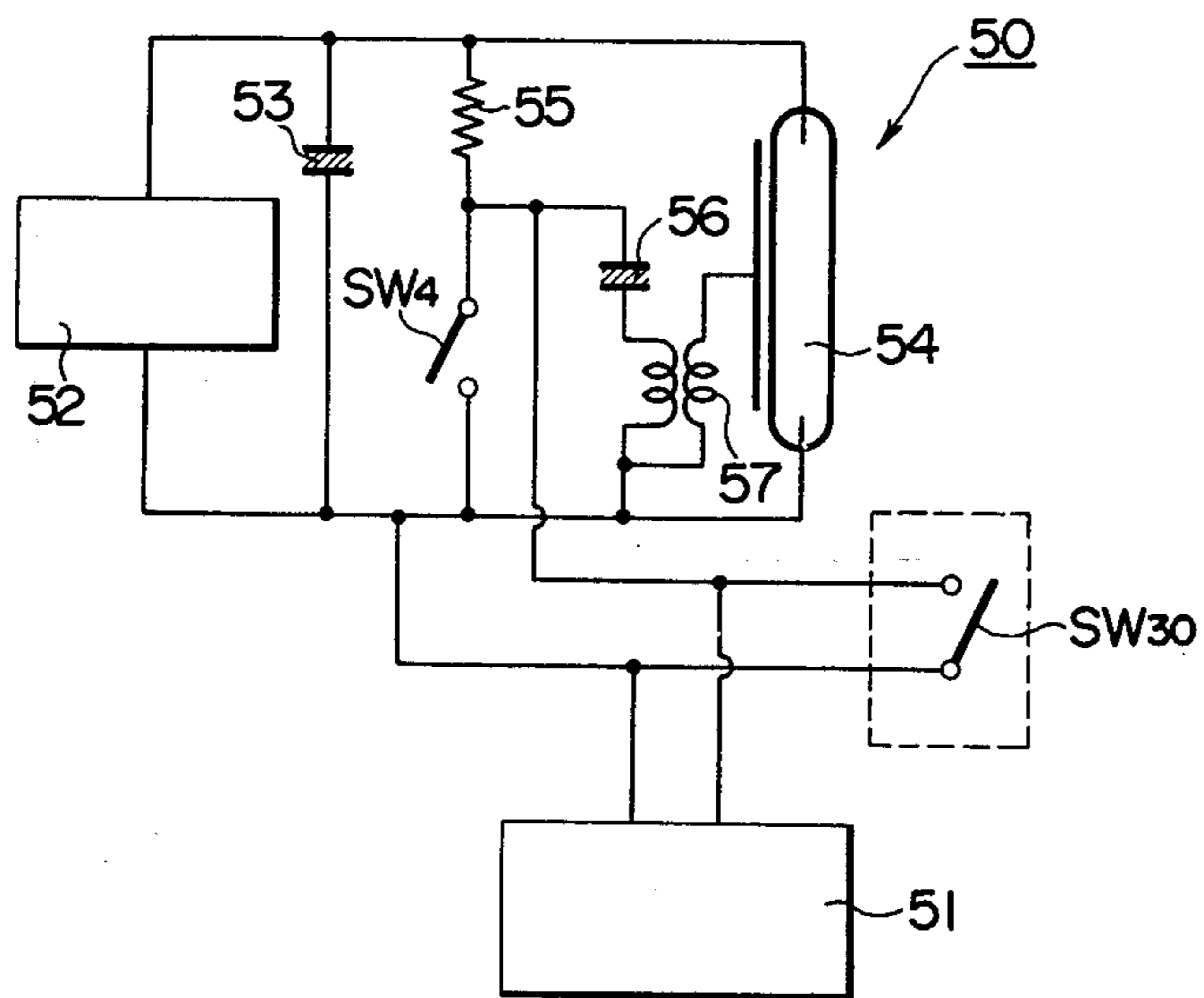
FIG. 2 (PRIOR ART)
