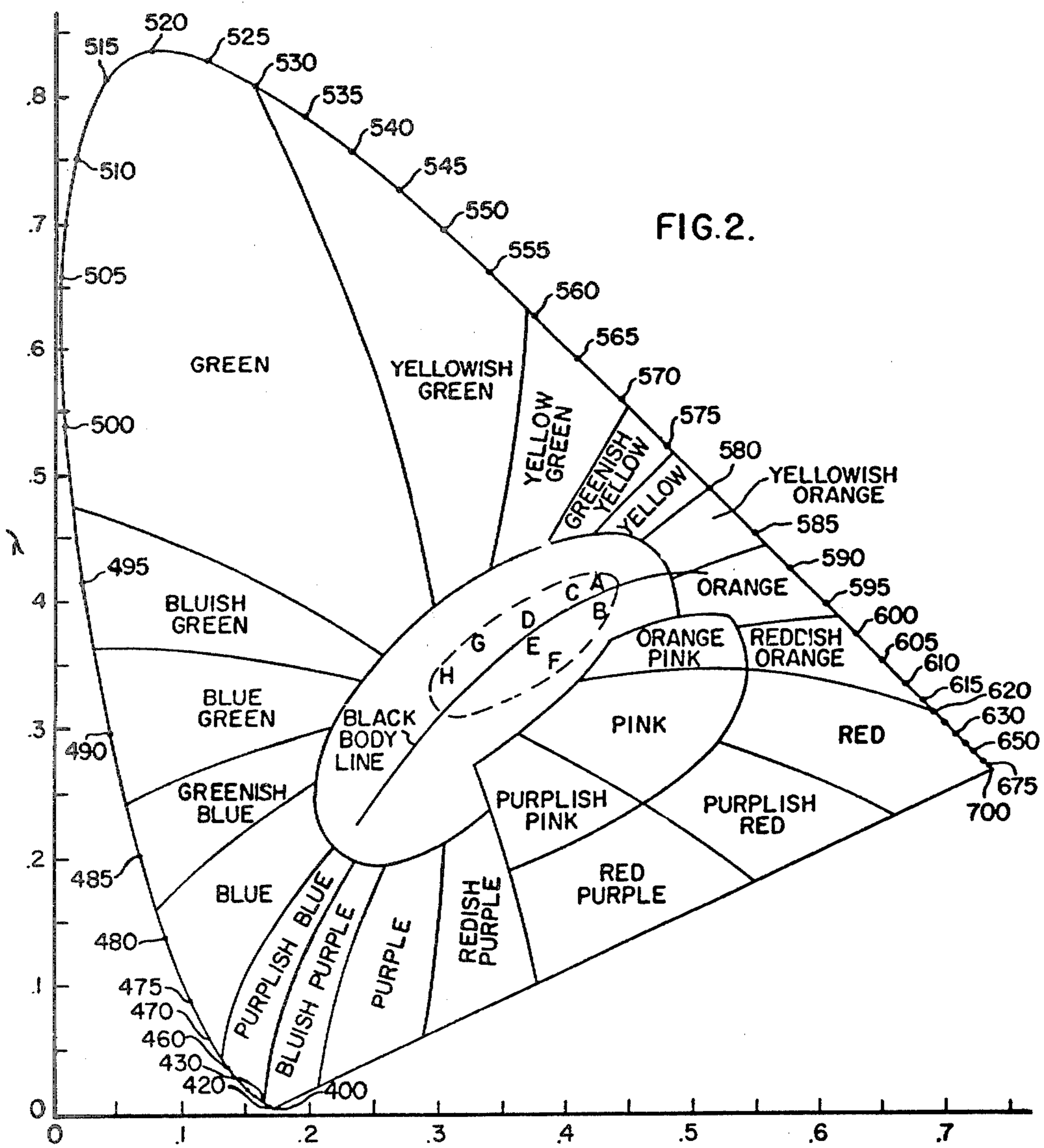
THE (x,y)-CHROMATICITY DIAGRAM OF THE ICI SYSTEM
