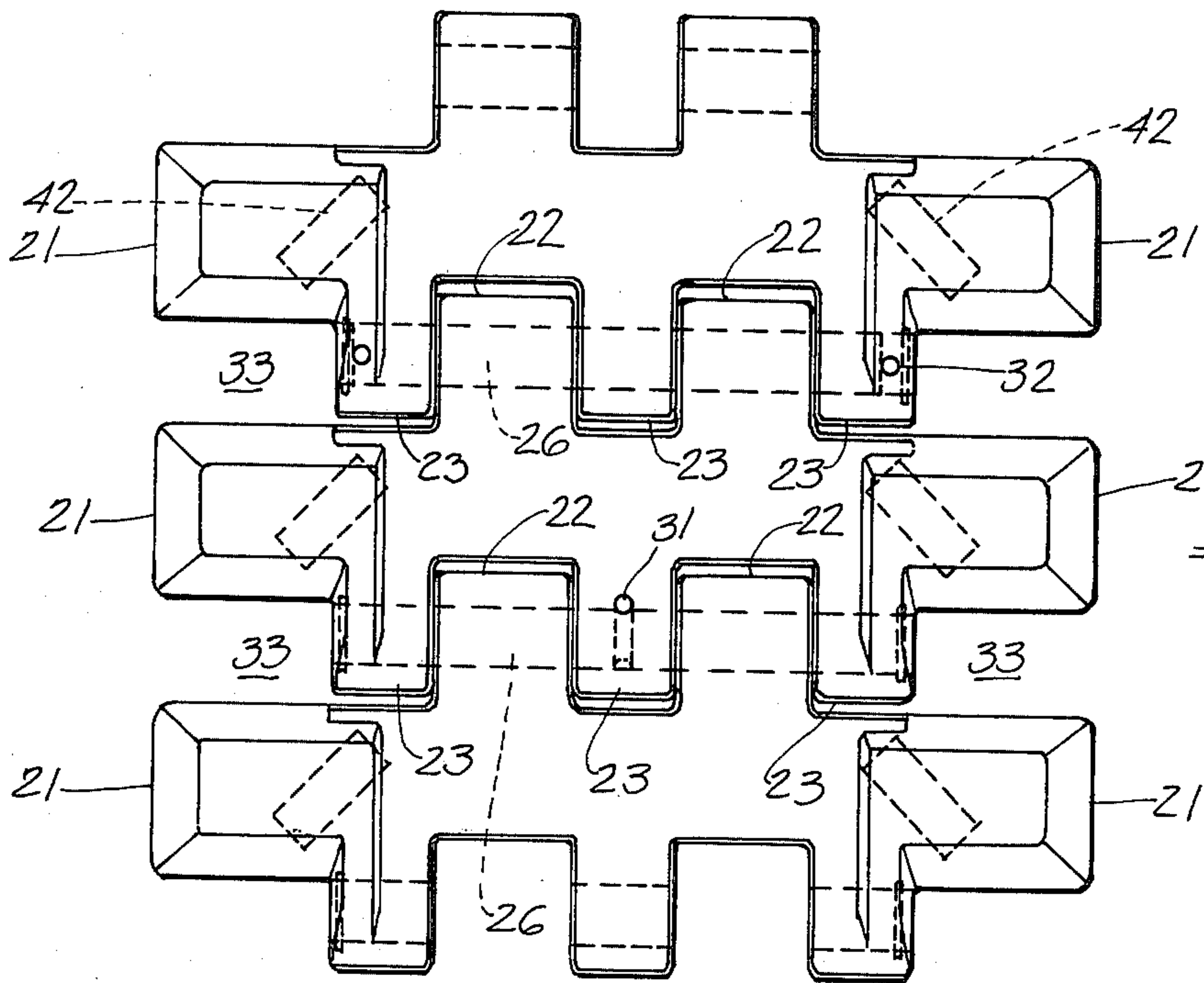
Fig. 6 PRIOR ART
