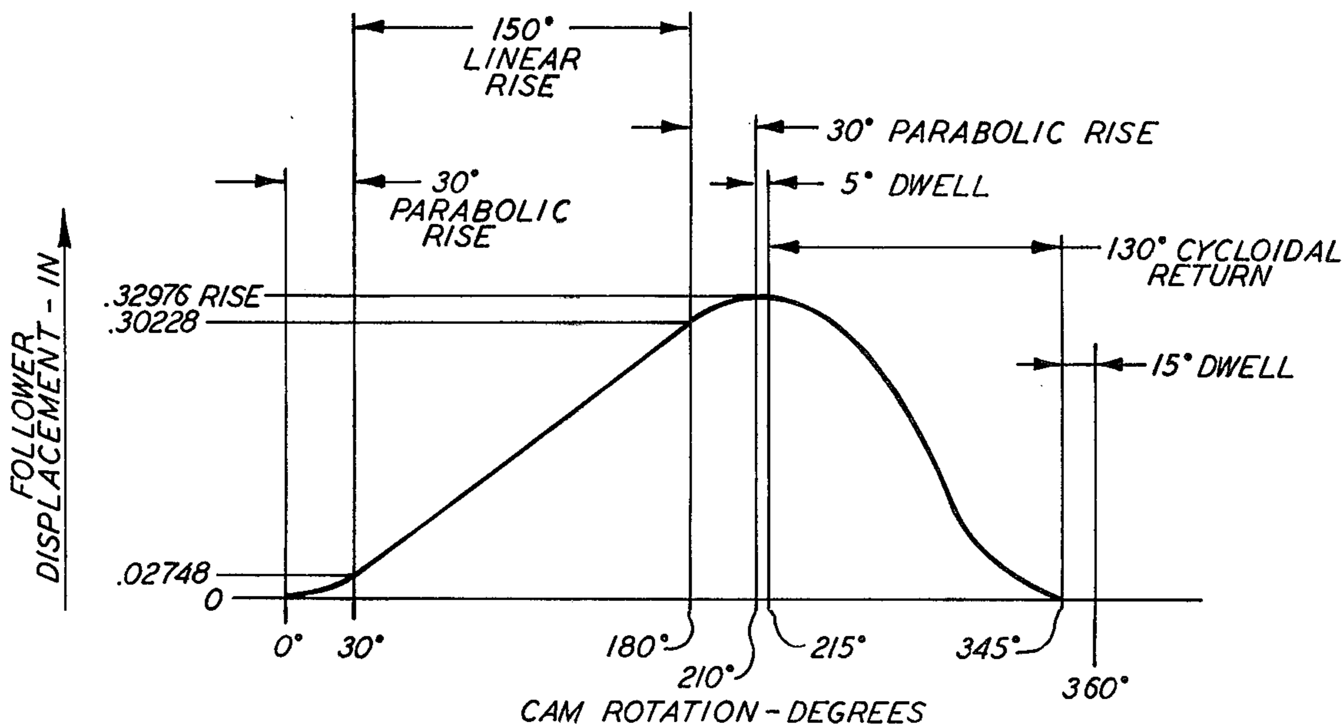
CAM FOLLOWER DISPLACEMENT DIAGRAM
