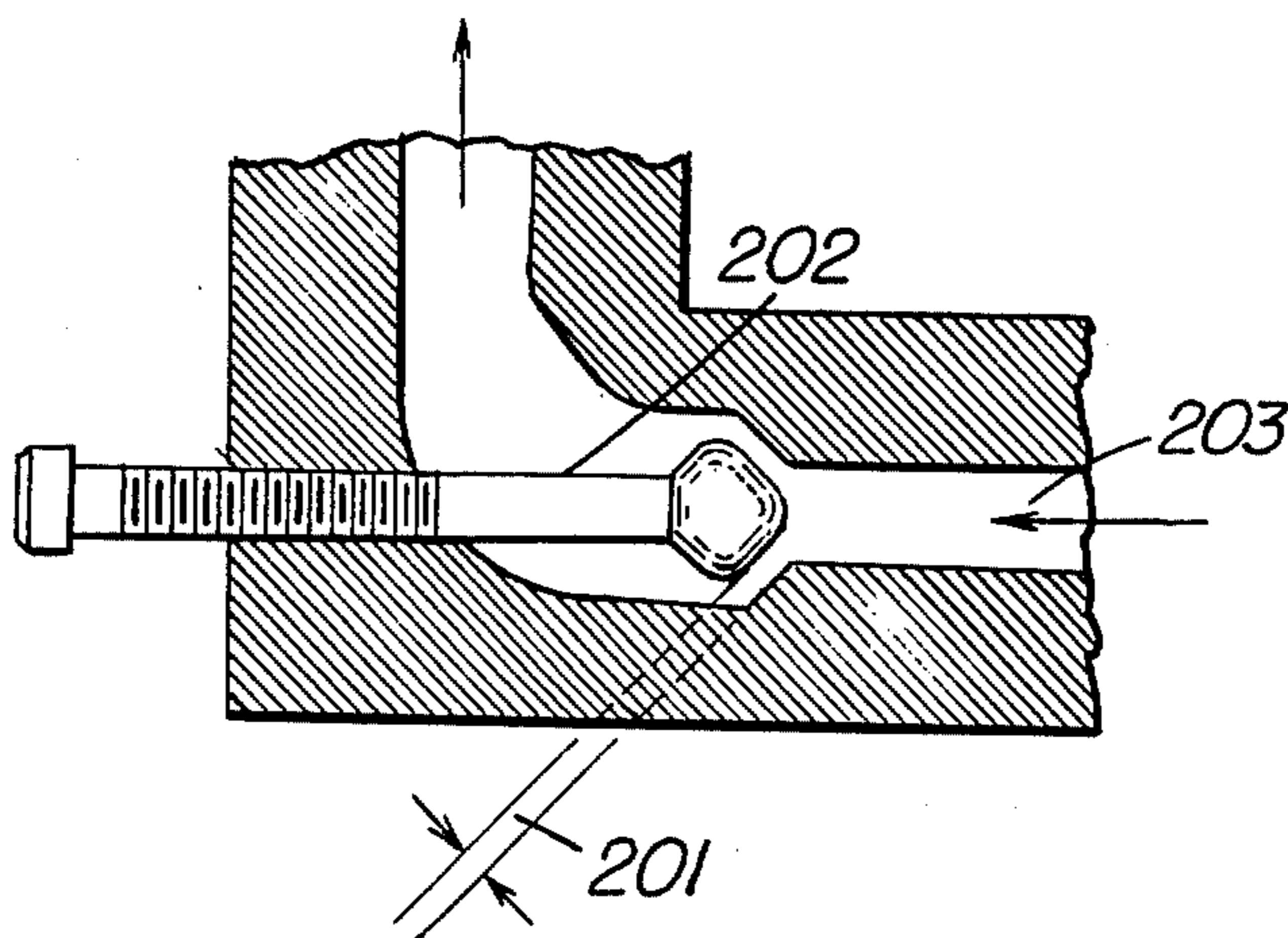
Fig. 6 PRIOR ART
