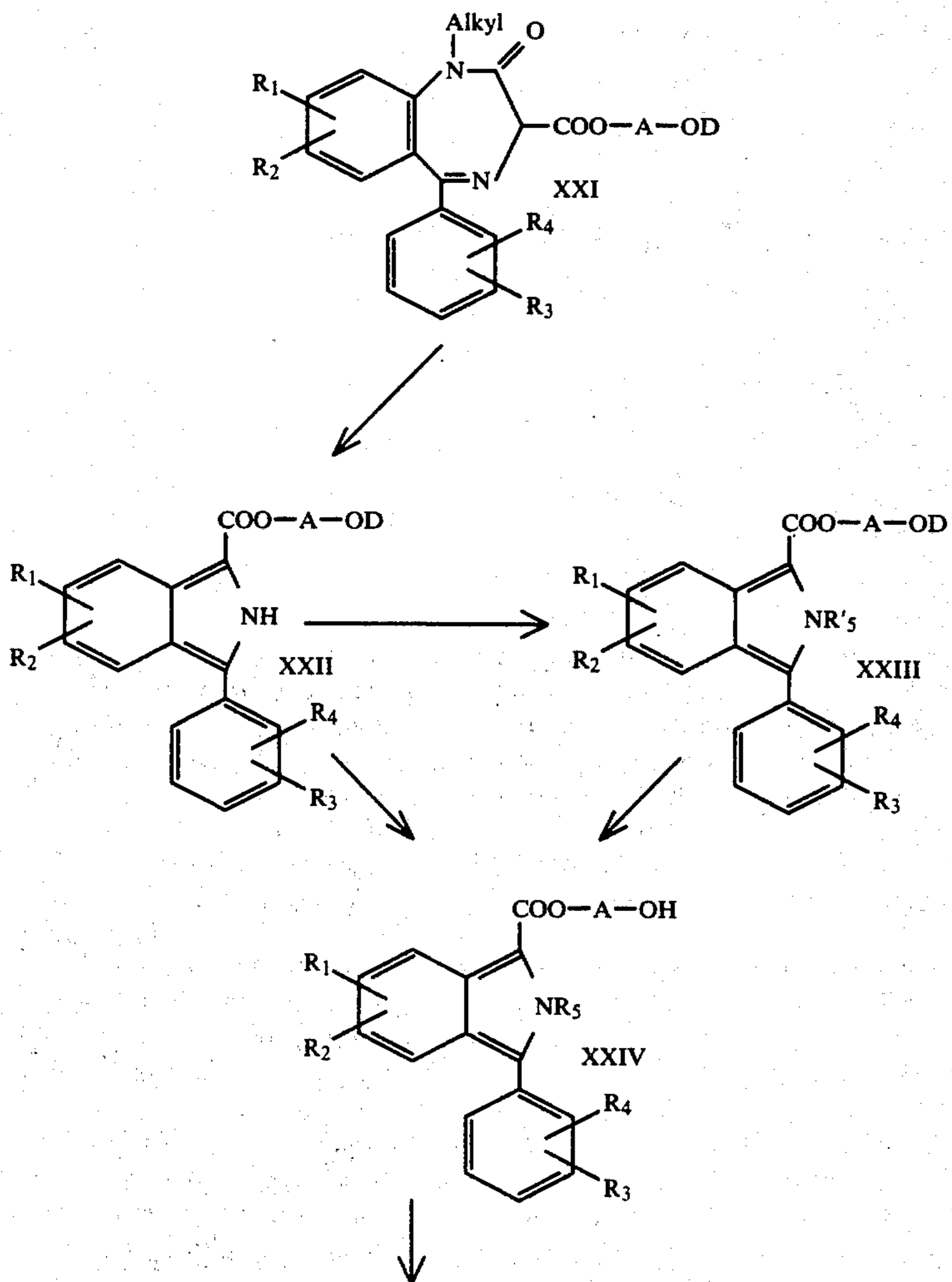
Formula Scheme II
