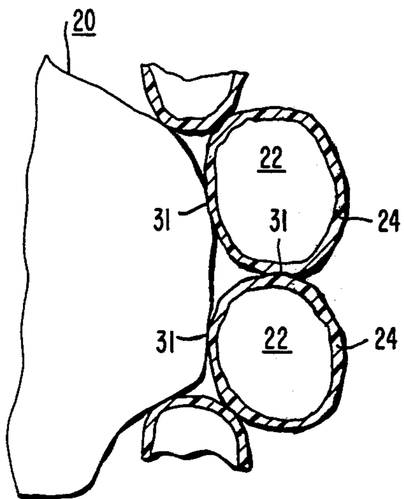
FIG. 3 PRIOR ART
