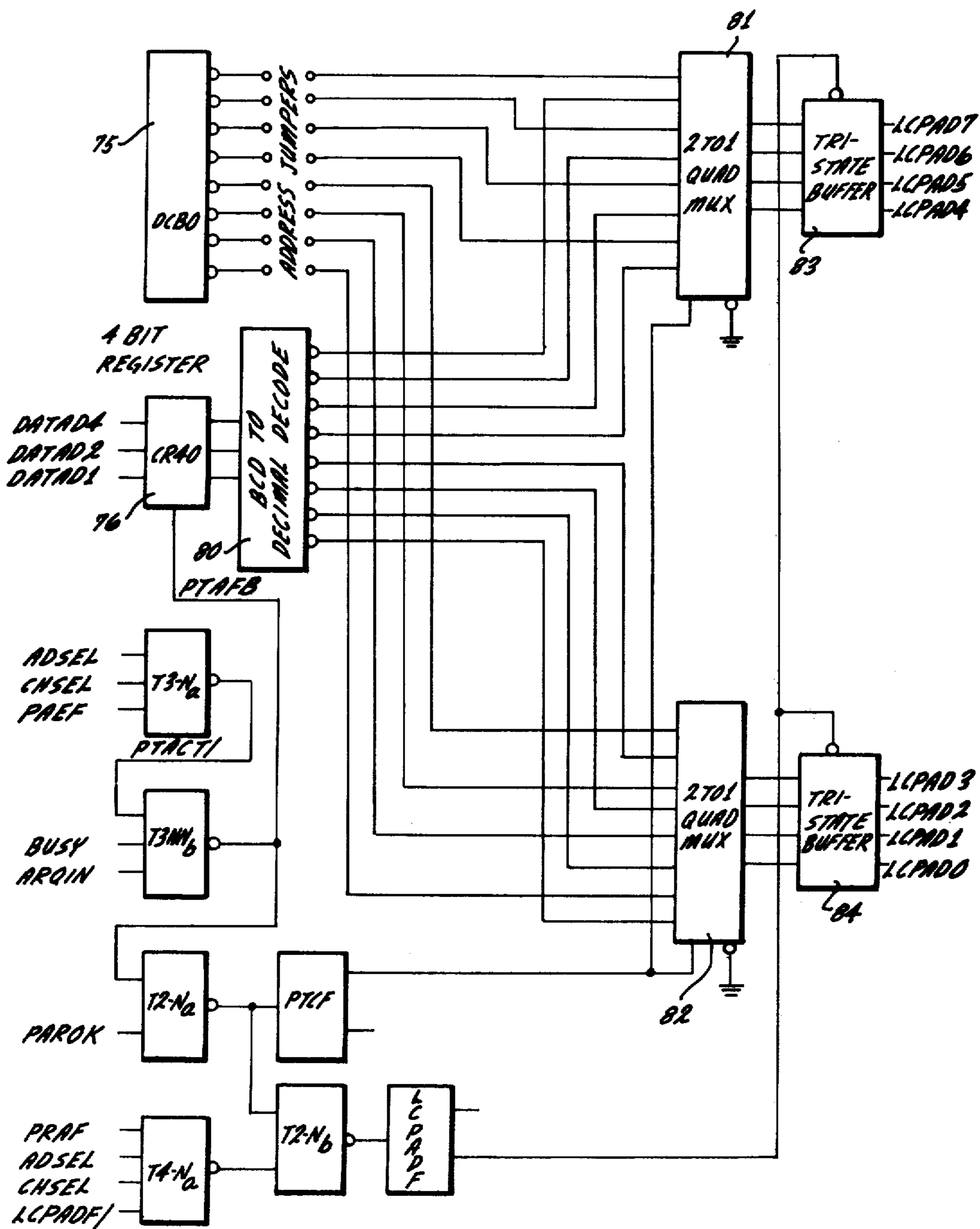
FIG. 5C-200 DISTRIBUTION CARD (LCP ADDRESS DECODING)
