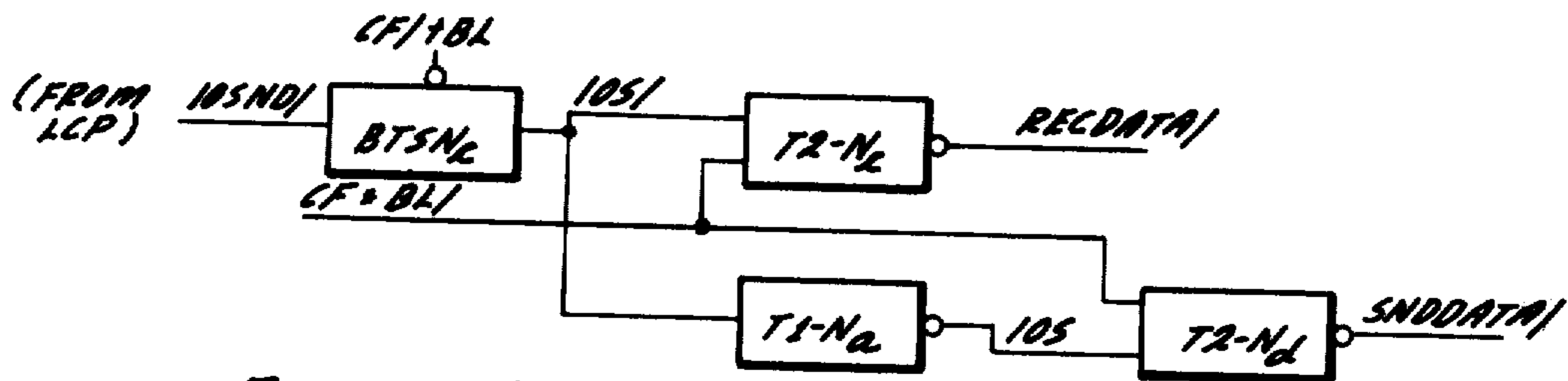
FIG. 5C-22 WRITE CYCLE DATA TRANSFERS
