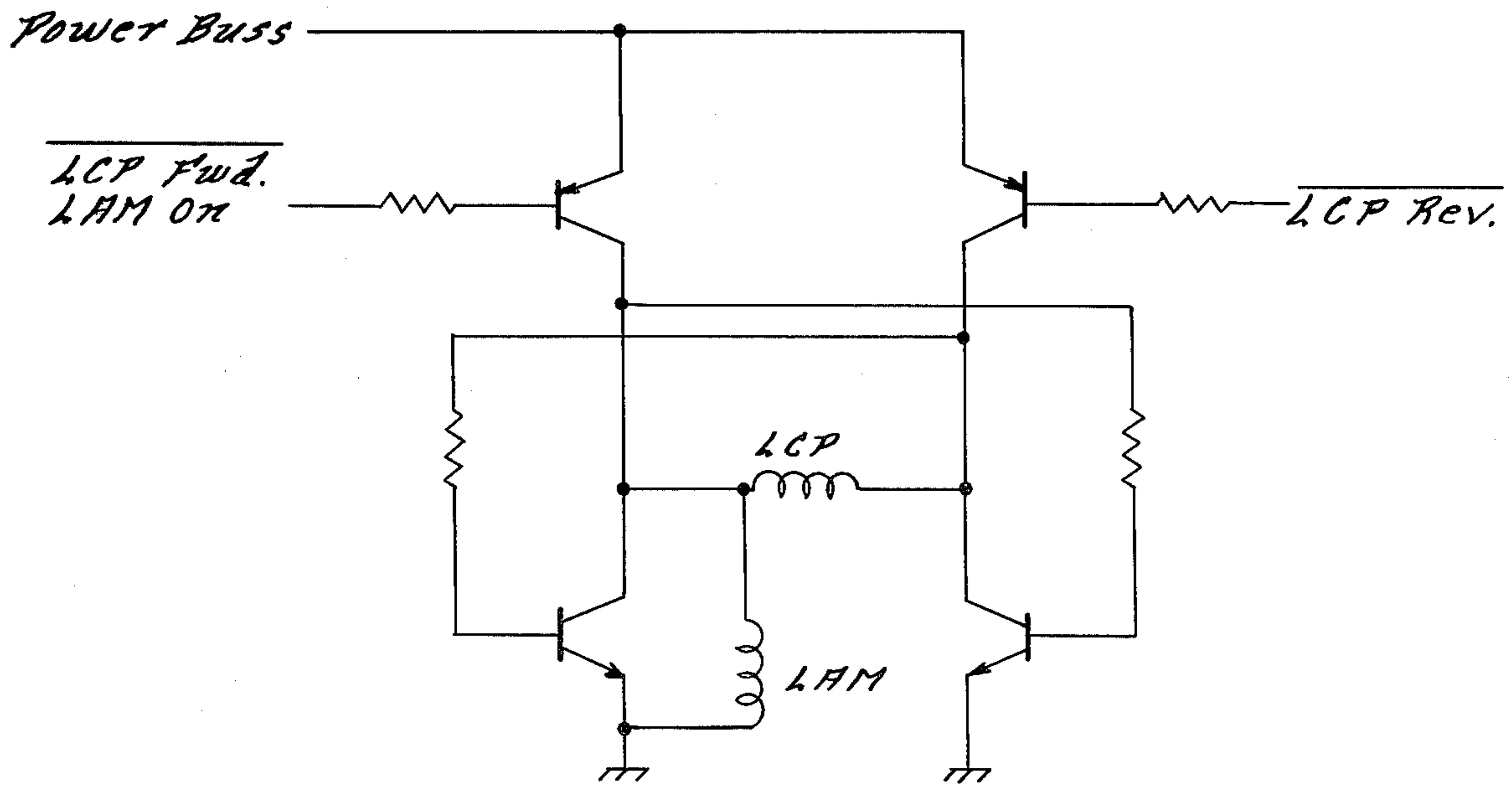
LCP & LAM Power Switch
