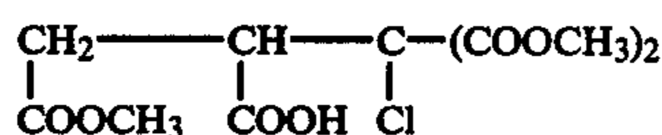
2—Ethyl hydrogen \alpha -(diethyl chloromalonyl)succinate
