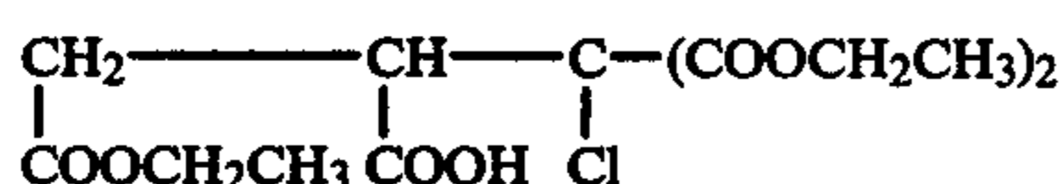
3—Methyl hydrogen \alpha -(diethyl-2-chloromalonyl)succinate
