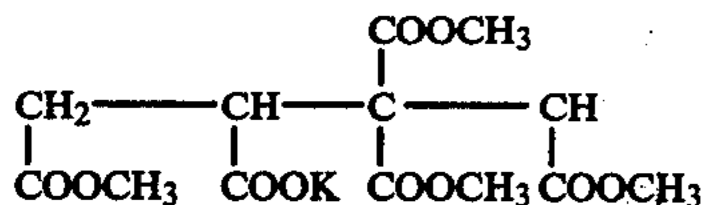
10—Potassium butane-1,2,2,4-tetracarboxylic methyl ester-3-carboxylate
