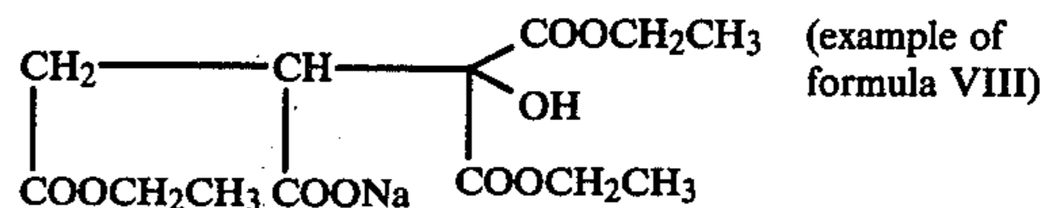
5—Dicalcium 1-hydroxy propane-1,1,2,3-tetracarboxylate
