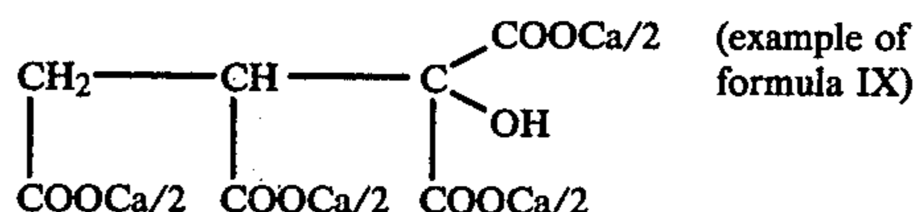
6—Tetrasodium propane-1-hydroxy-1,1,2,3-tetracarboxylate
