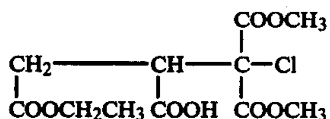
5—Methyl hydrogen \alpha -(dimethyl bromomalonyl)succinate
