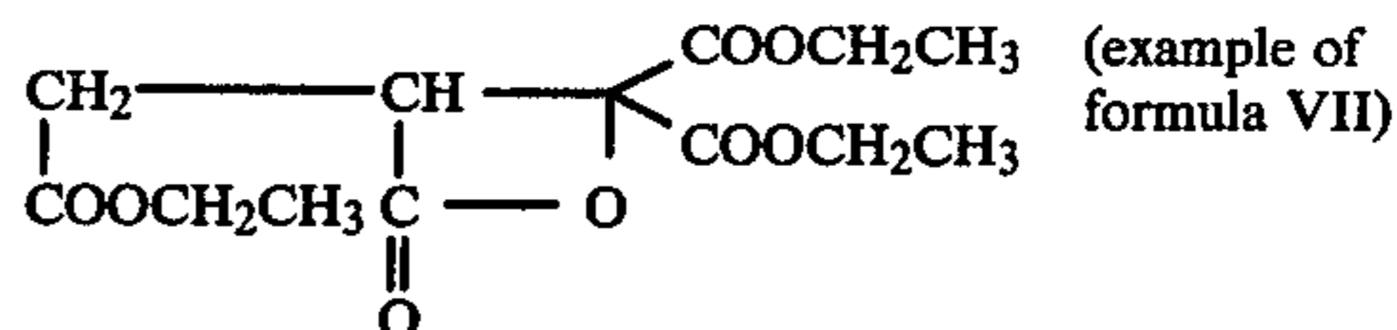
4—Ethyl hydrogen \alpha -(diethyl hydroxymalonyl)succinate
