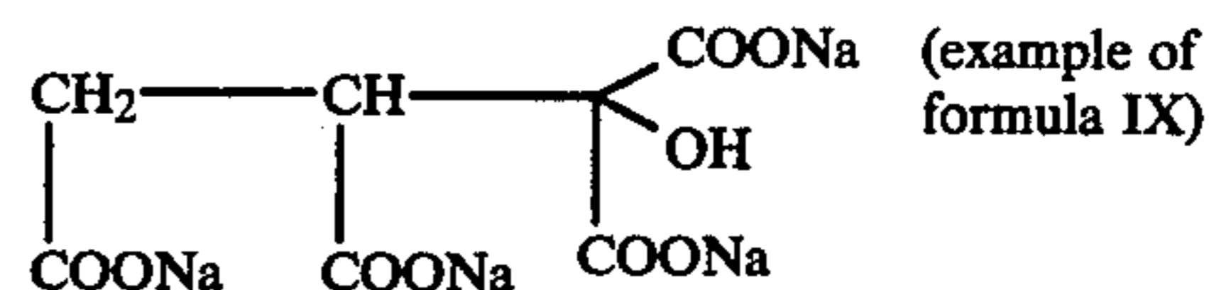
6—Tetrasodium propane-1-hydroxy-1,1,2,3-tetracarboxylate
