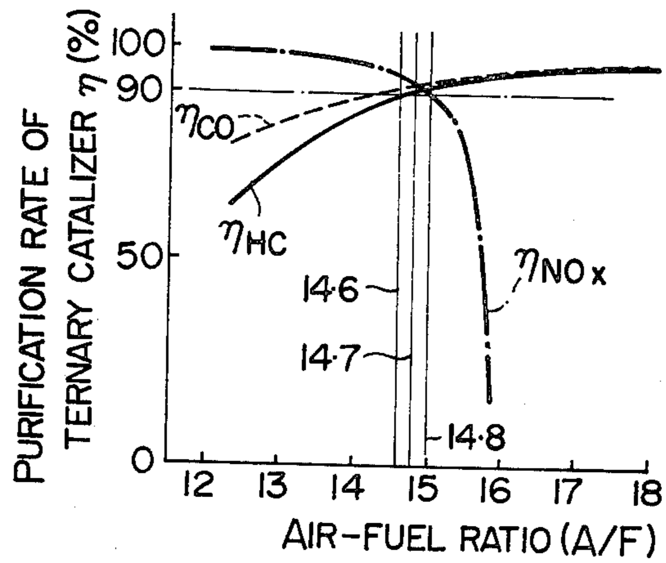
FIG. 2 PRIOR ART
