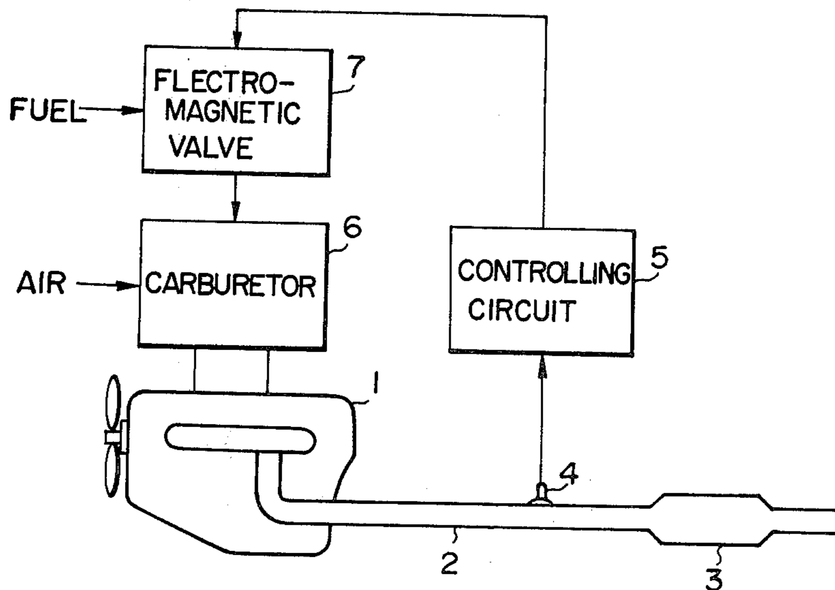
FIG. 2 PRIOR ART
