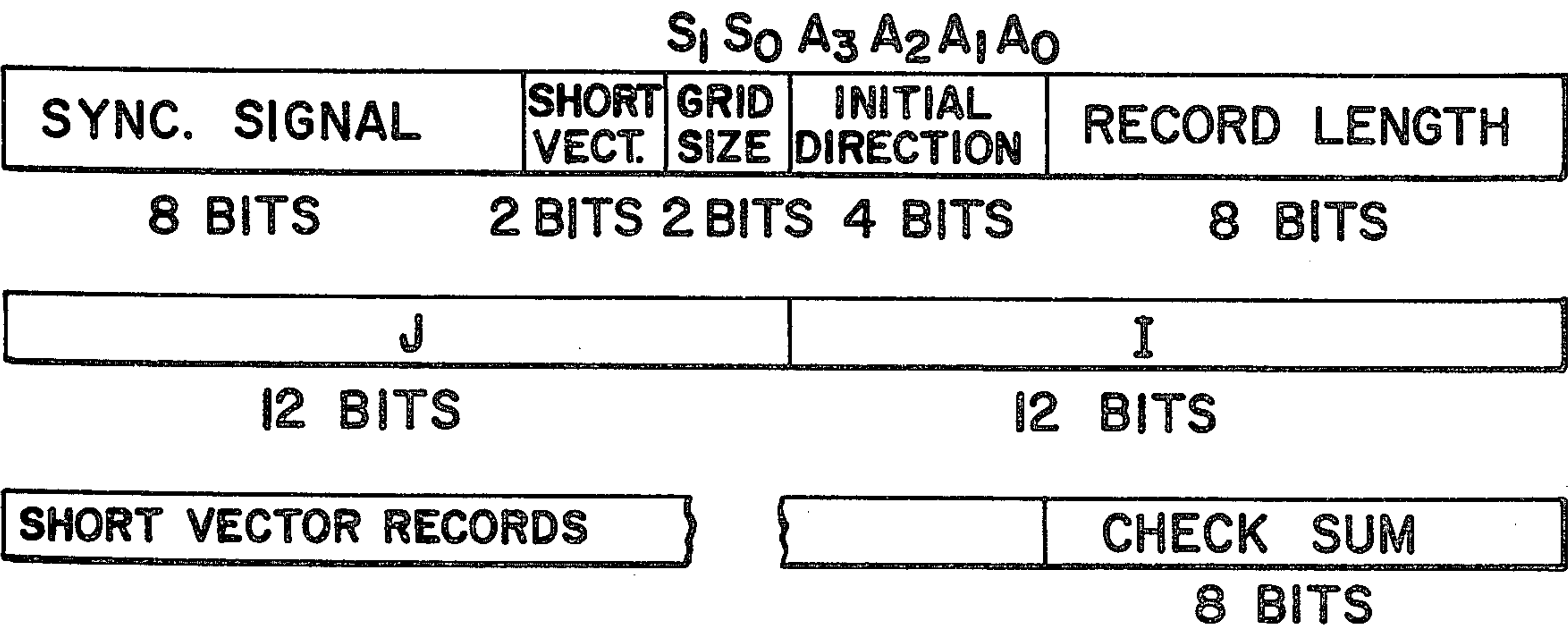
SHORT VECTOR MESSAGE
