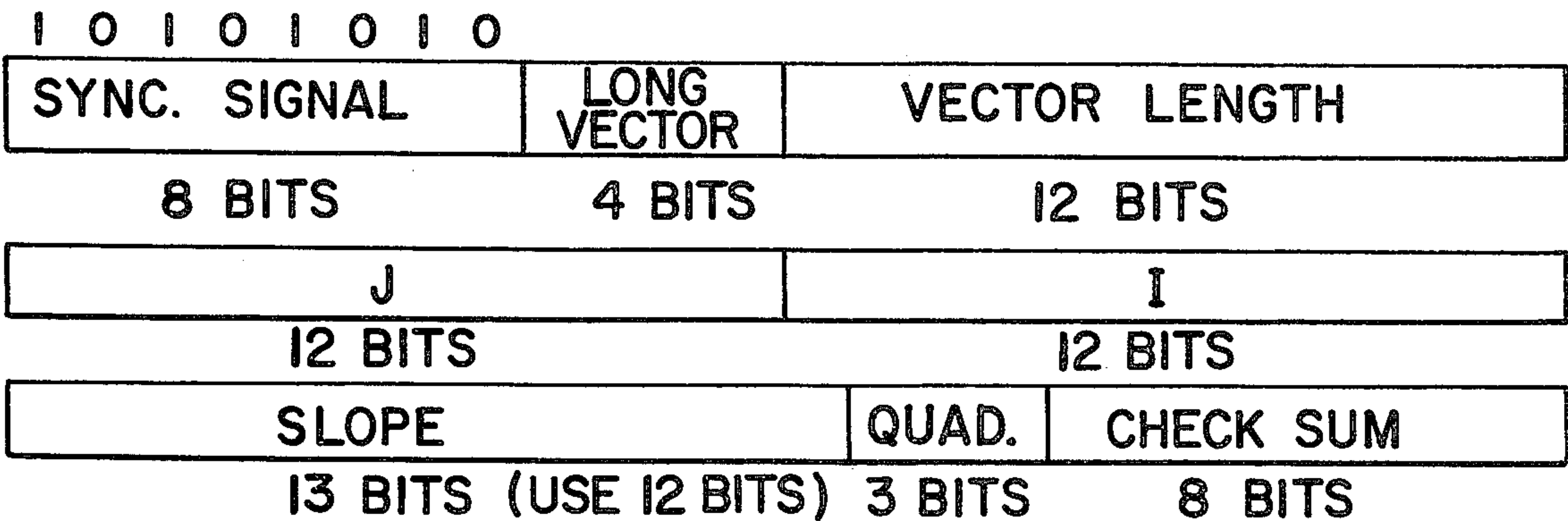
FIG _ 4 LONG VECTOR MESSAGE
