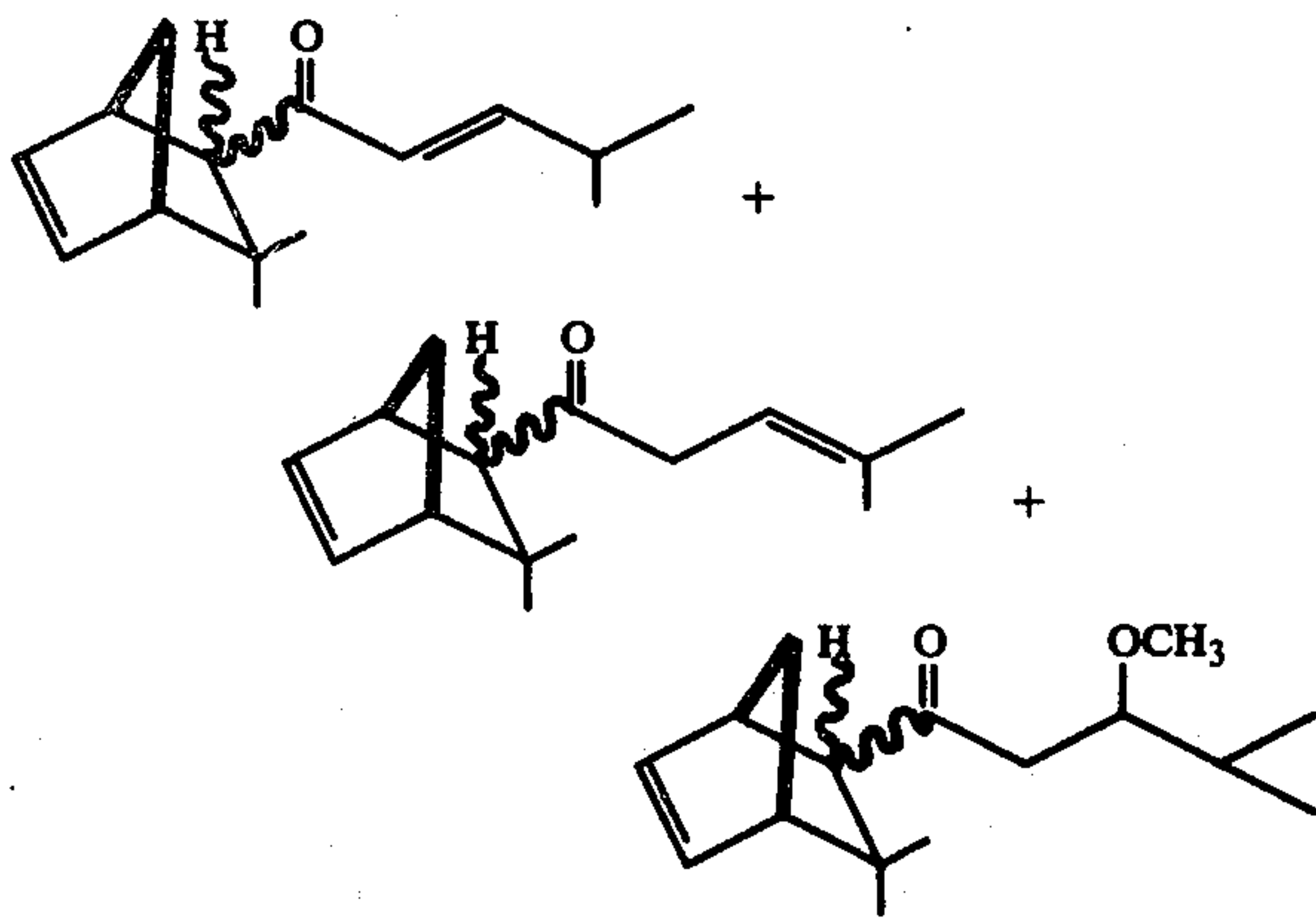
Spectral Data for Total Mixture
