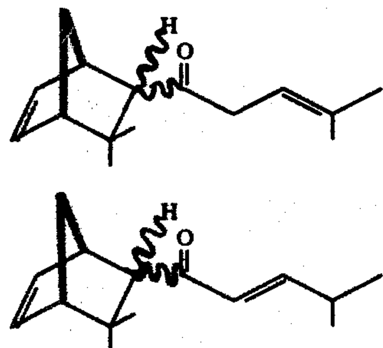
FIG. 22 illustrates the GLC profile for the mixture of ketones and keto ethers produced according to Example XXI, having the structures:
