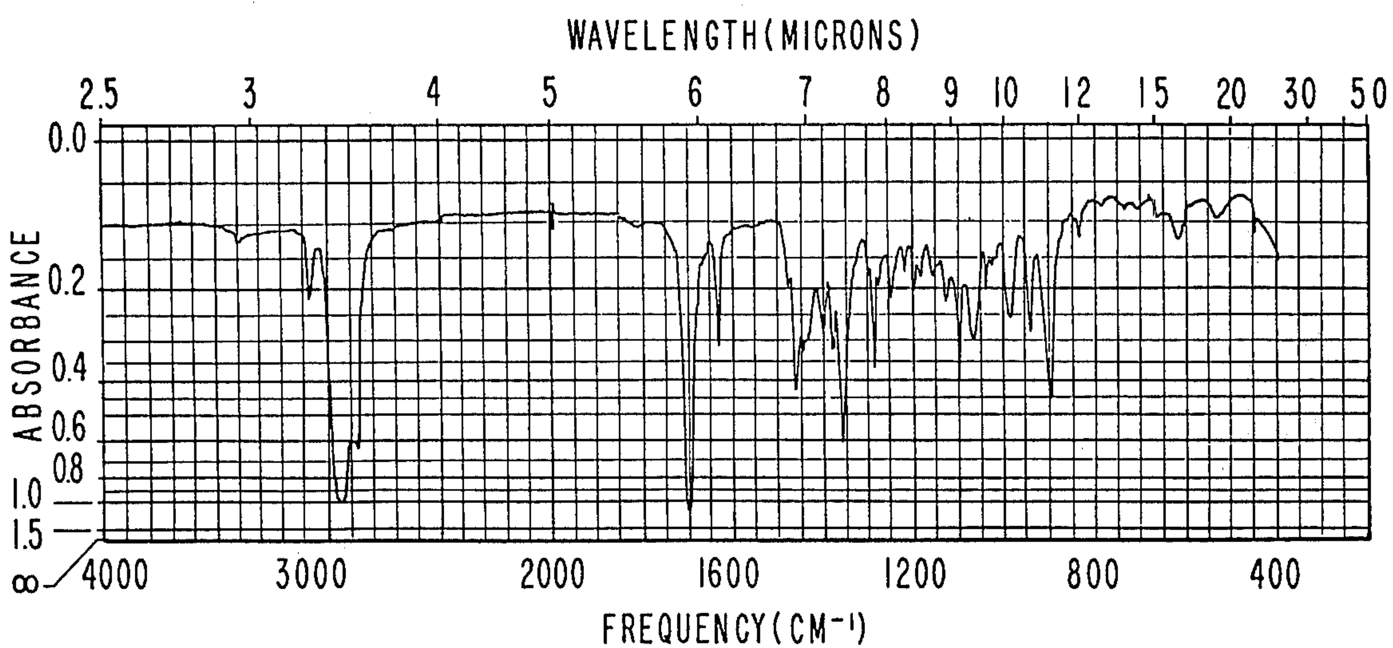
I R SPECTRUM FOR EXAMPLE XXV, PART B.
