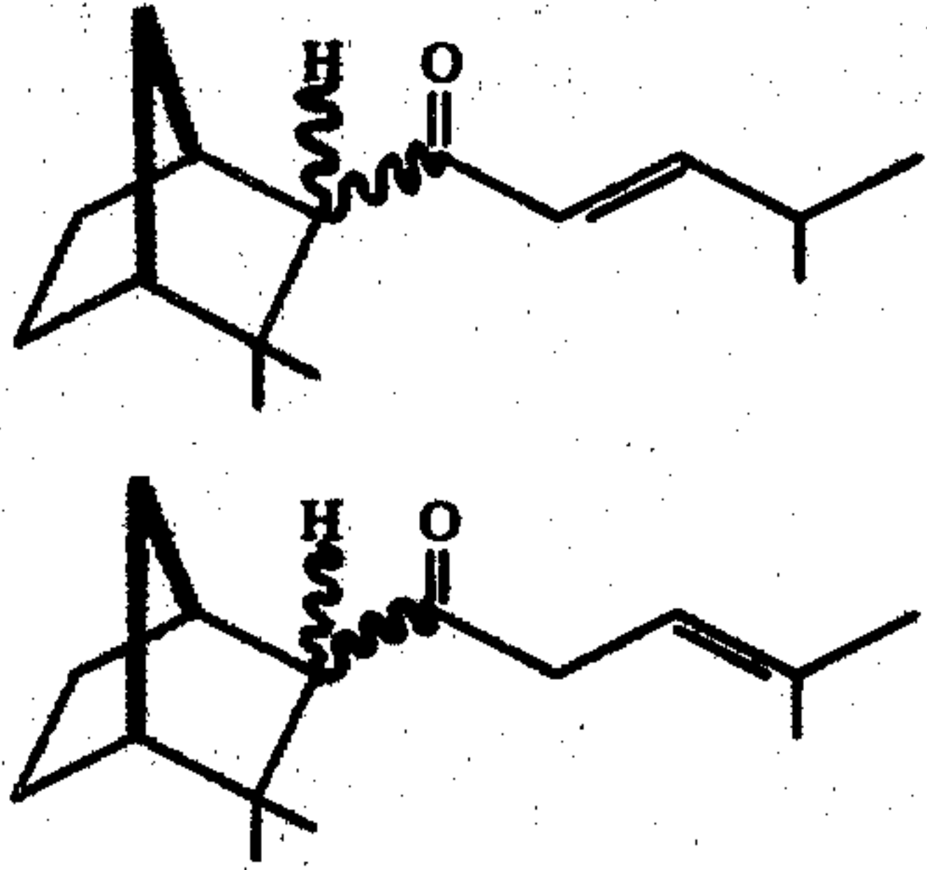
FIG. 19 illustrates the Infrared spectrum of peak 1, fraction 18 of Example XX, which is a mixture of the two ketones having the structures:
