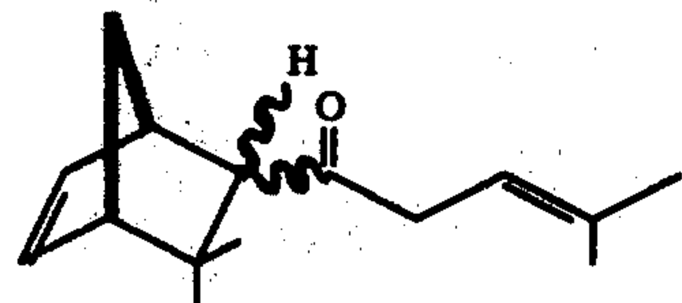
FIG. 24 is the Infrared spectrum for the mixture of ketones and keto ethers produced according to Example XXI, having the structures:
