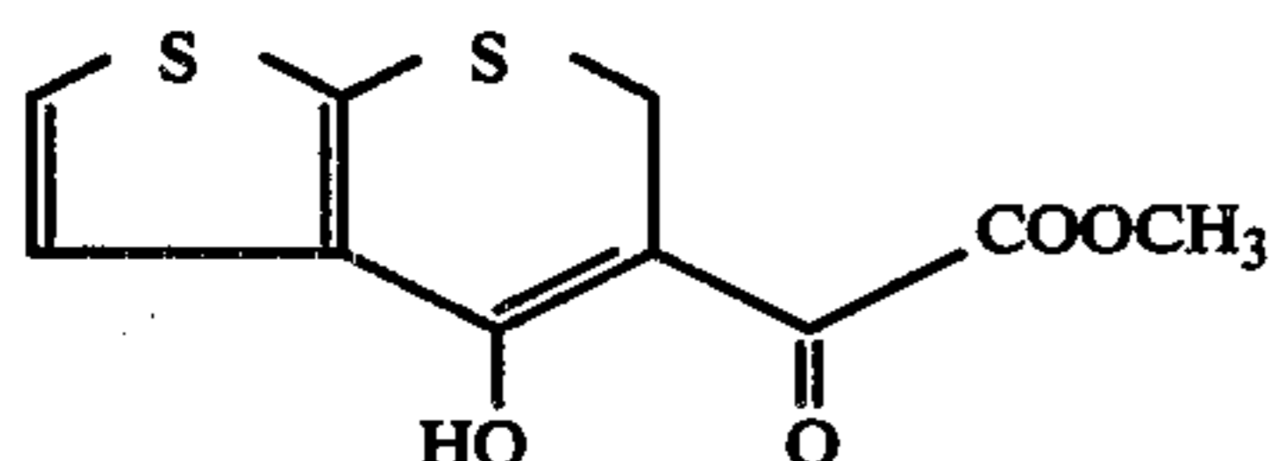
Methyl 4-hydroxy- \alpha -oxo-6H-thieno[2,3-b]-thiopyran-5-acetate.
