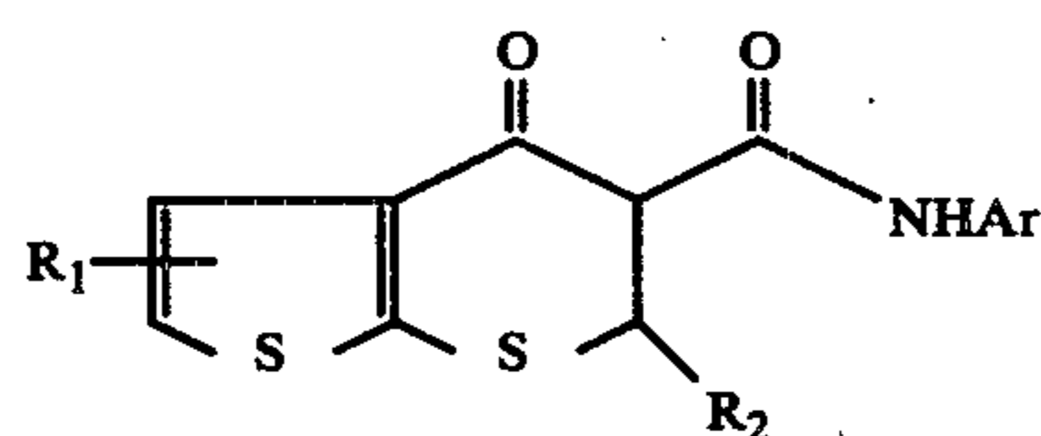
Amides of 5,6-dihydro-4-oxo-4H-thieno[2,3-b]thiopyran-5-carboxylic acid
