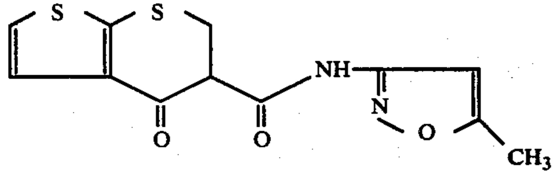
5,6-Dihydro-N-(5-methyl-3-isoxazolyl)-4-oxo-4H-thieno[2,3-b]-thiopyran-5-carboxamide
