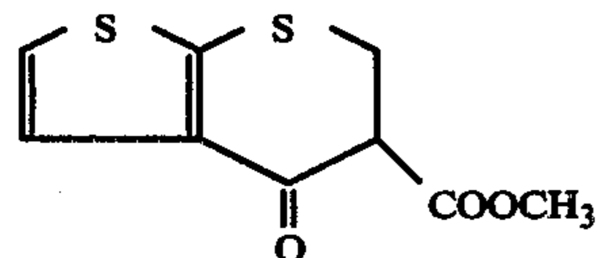
Methyl 5,6-dihydro-4-oxo-4H-thieno[2,3-b]thiopyran-5-carboxylate
