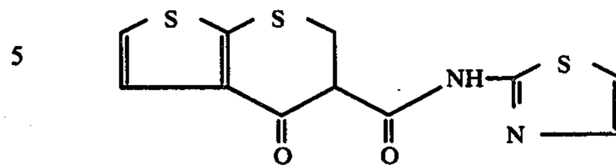
5,6-Dihydro-4-oxo-N-(2-thiazolyl)-4H-thieno[2,3-b]-thiopyran-5-carboxamide
