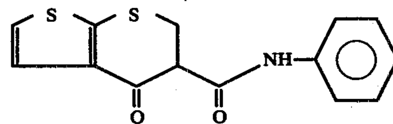
5,6-Dihydro-4-oxo-N-phenyl-4H-thieno[2,3-b]-thiopyran-5-carboxamide
