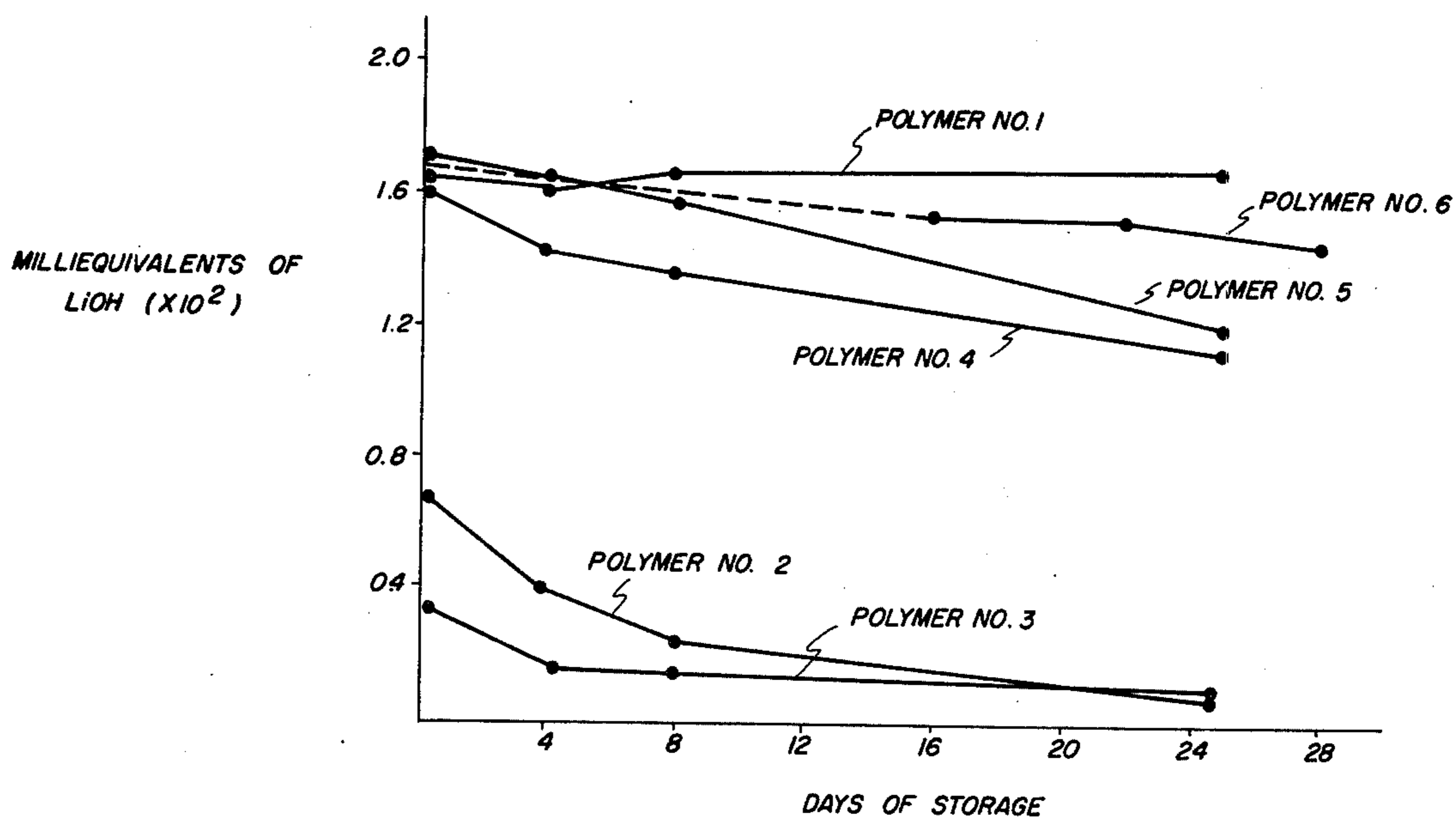
STABILITY OF LIOH HAND COATINGS
