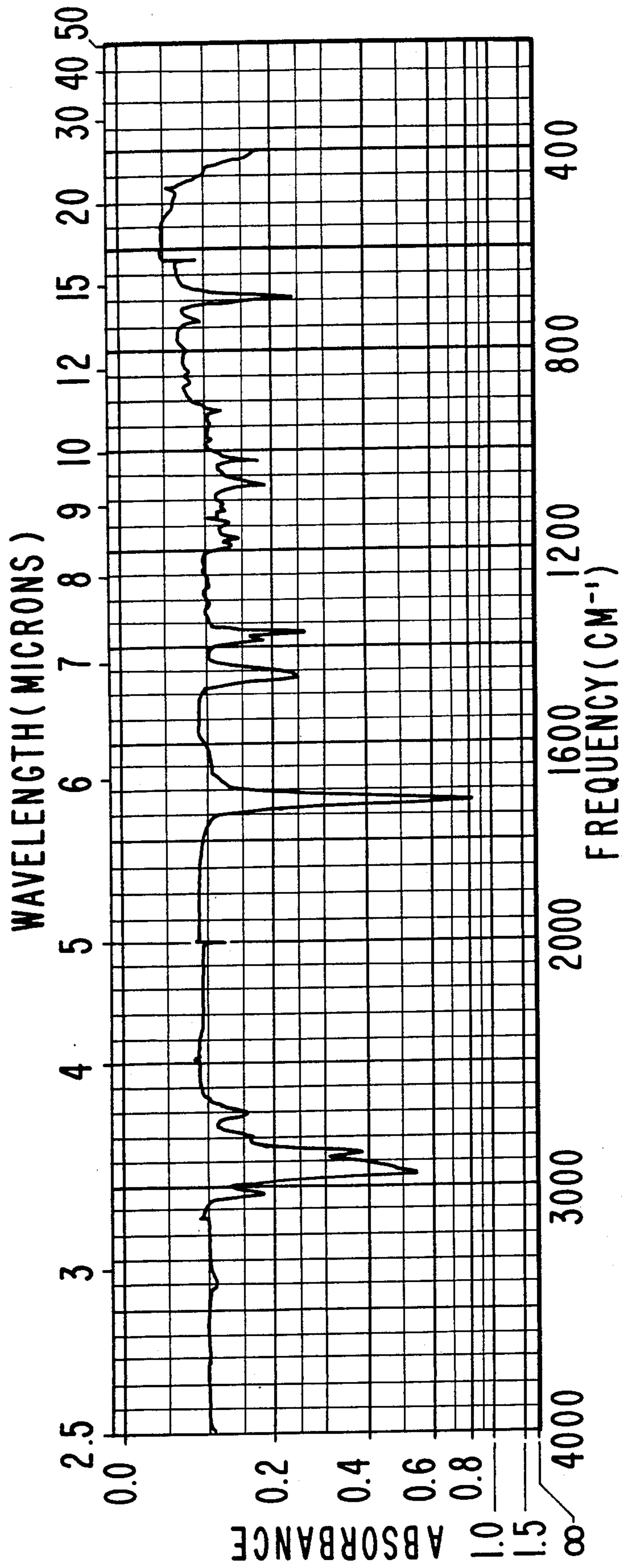
IR SPECTRUM FROM EXAMPLE II
