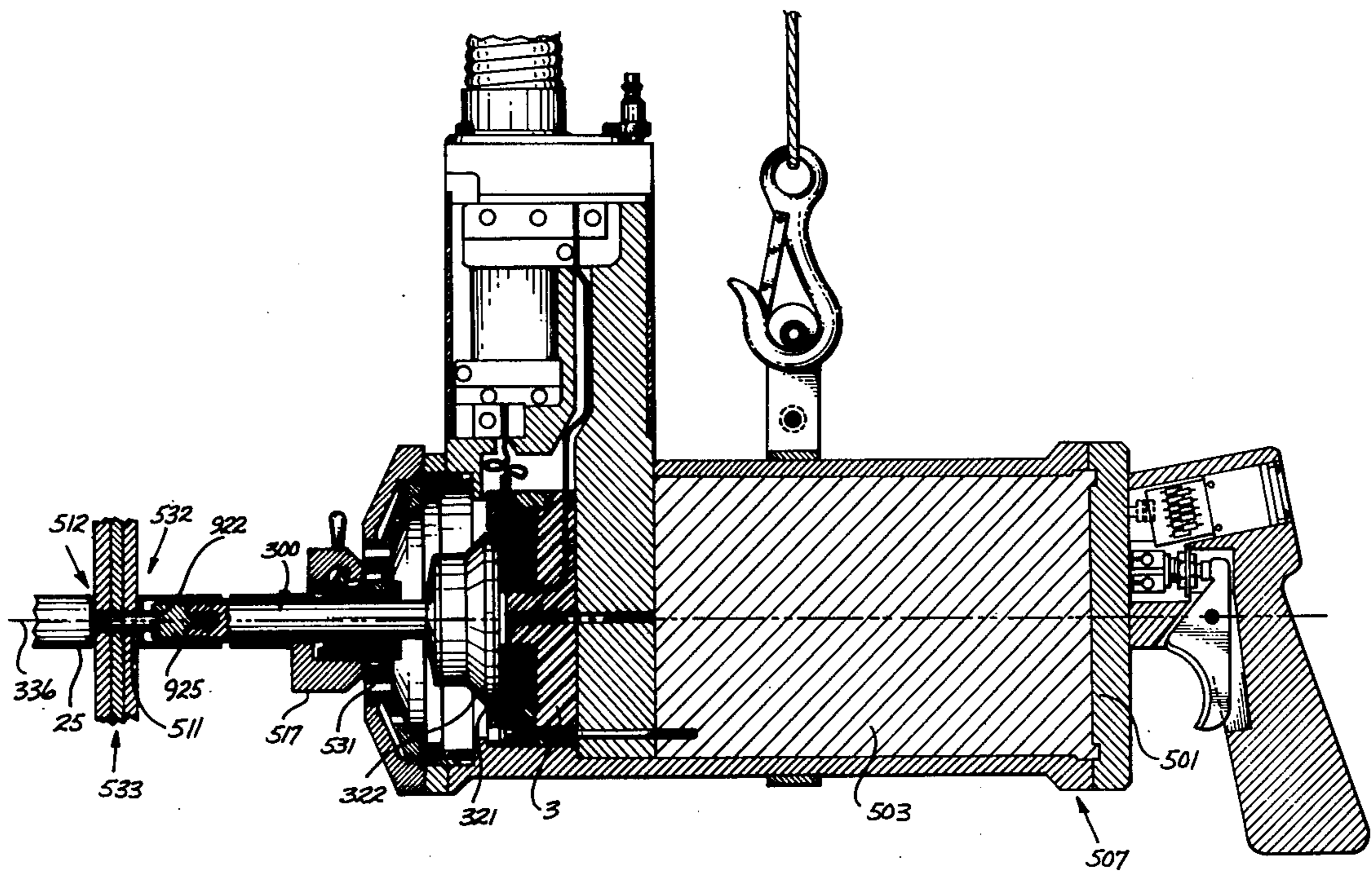
SOLID MASS RECOIL EMR GUN ASSEMBLY
