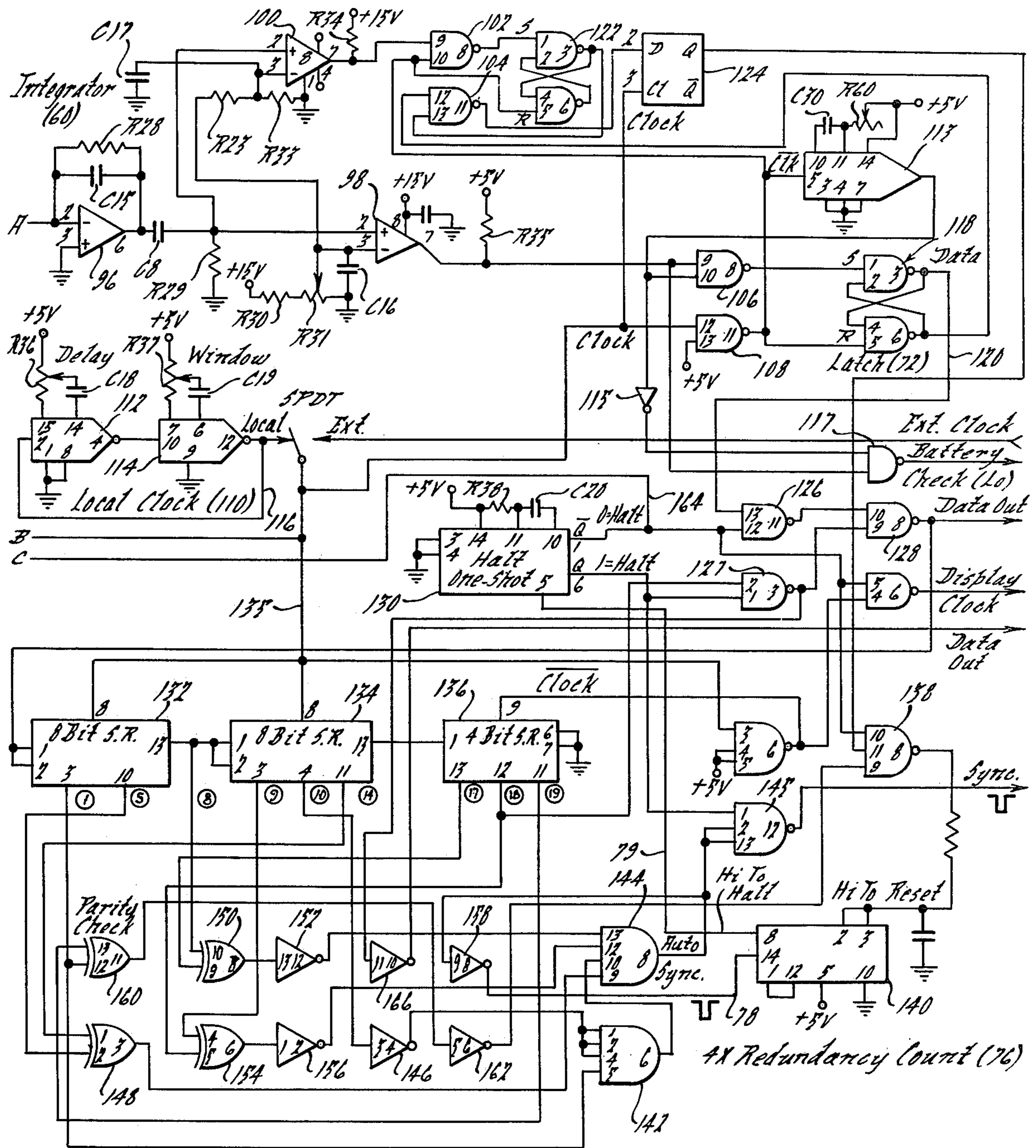
Auto Synchronous Decoder (74)
