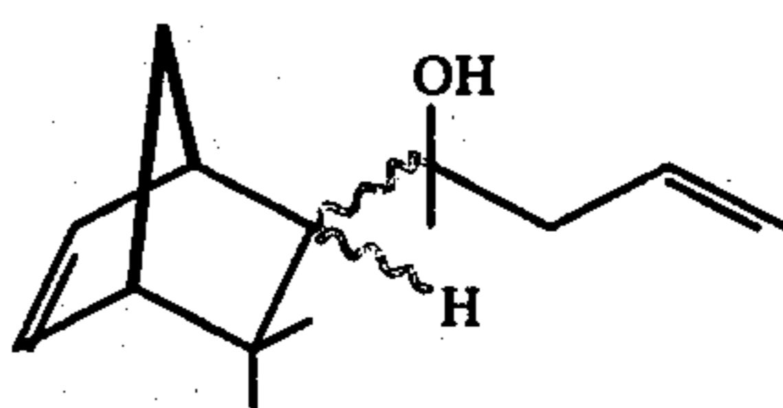
FIG. 48 is the NMR spectrum for the compound having the structure:
