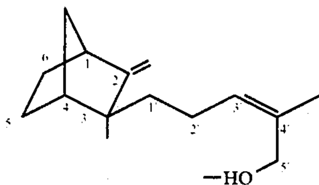
endo-3-methyl-exo-3-(cis-5'-hydroxy-4'-methylpent-3'-enyl)-2-methylenebicyclo[2.2.1]heptane
