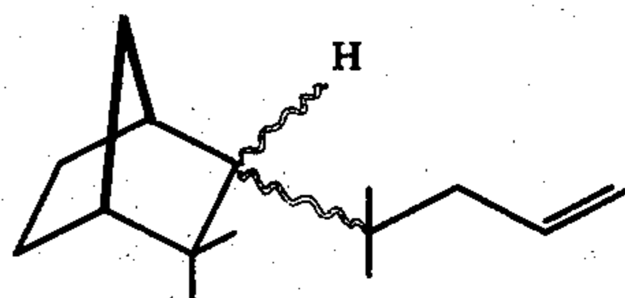
FIG. 45 illustrates the Infrared spectrum for the compound having the structure:
