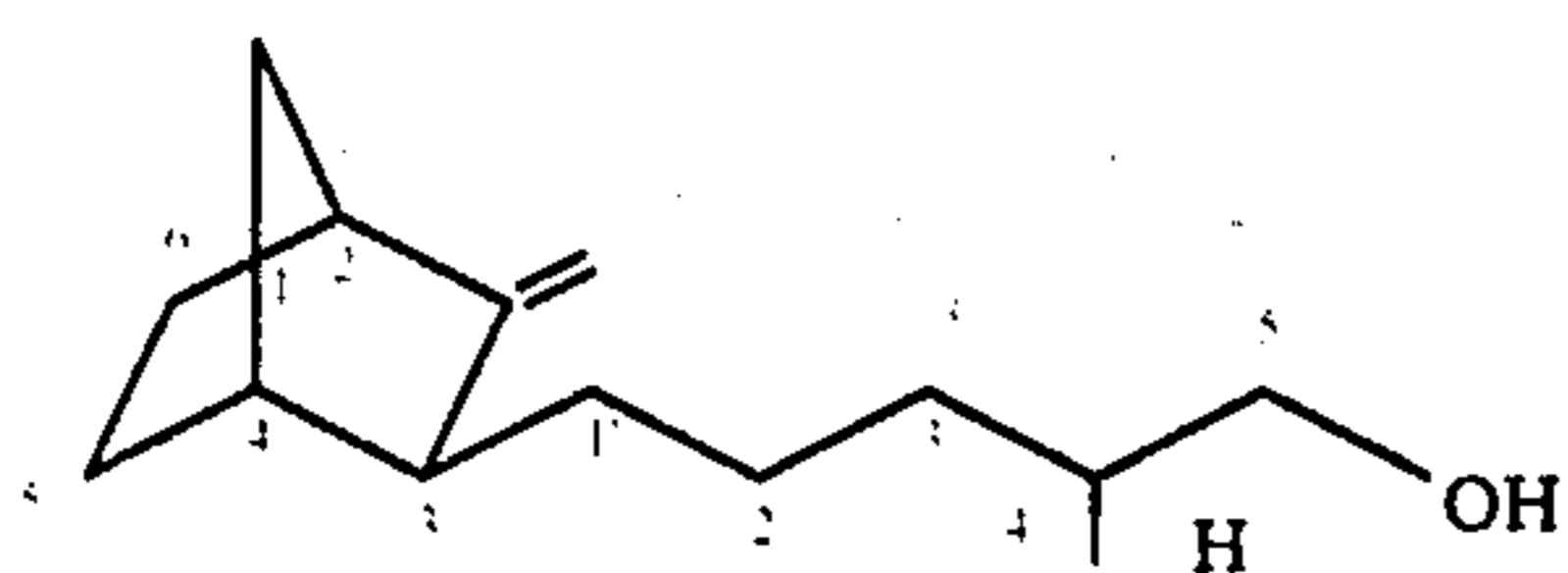
2-methylene-3-exo-(4'-methyl-5'-hydroxypentyl)-bicyclo[2.2.1]heptane; 3-normethyldihydro-beta-santalol
