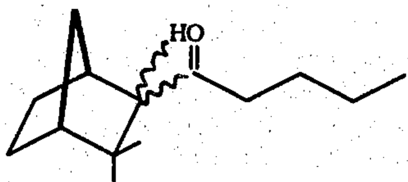
FIG. 41 is the Infrared spectrum for the compound having the structure:
