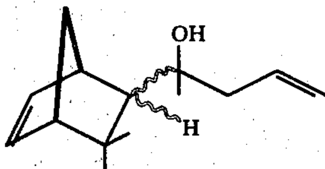
FIG. 46 illustrates the NMR spectrum for the compound having the structure:
