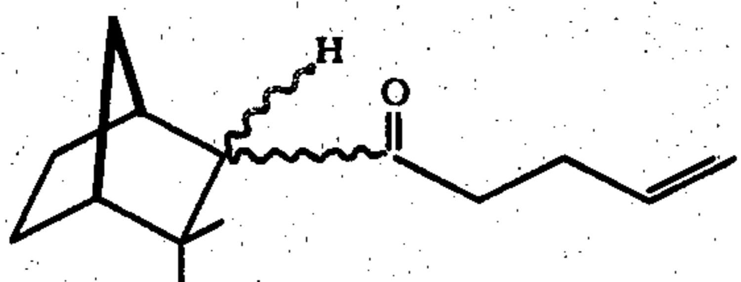
FIG. 40 is the NMR spectrum for the compound having the structure:
