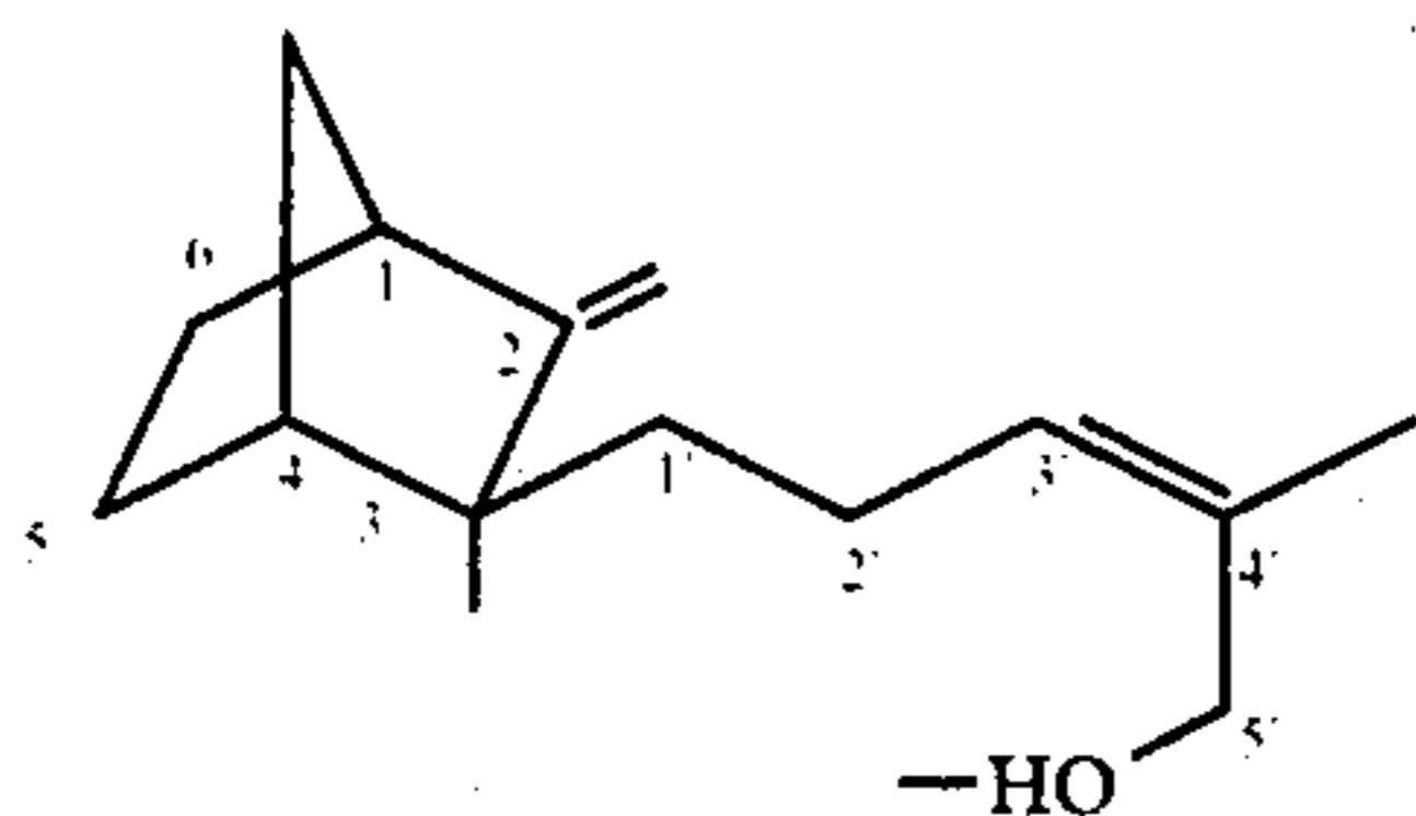
endo-3-methyl-exo-3-(cis-5'-hydroxy-4'-methylpent-3'-enyl)-2-methylenebicyclo[2.2.1]heptane
