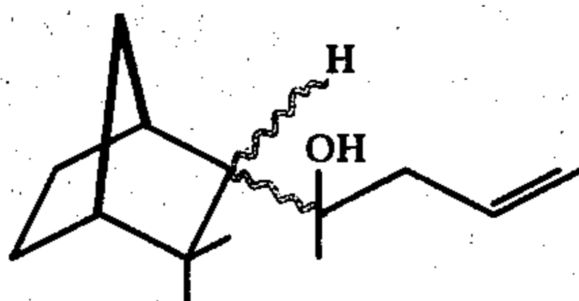
FIG. 44 illustrates the NMR spectrum for the compound having the structure:
