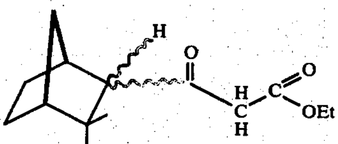
FIG. 38 is the NMR spectrum for the compound produced in Part B of Example XXV having the structure:
