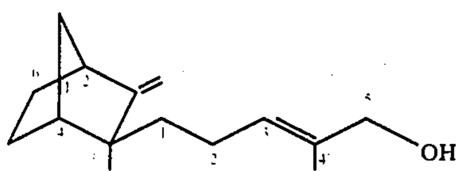
endo-3-methyl-exo-3-(trans-5'-hydroxy-4'-methylpent-3'-enyl)-2-methylenebicyclo[2.2.1]heptane
