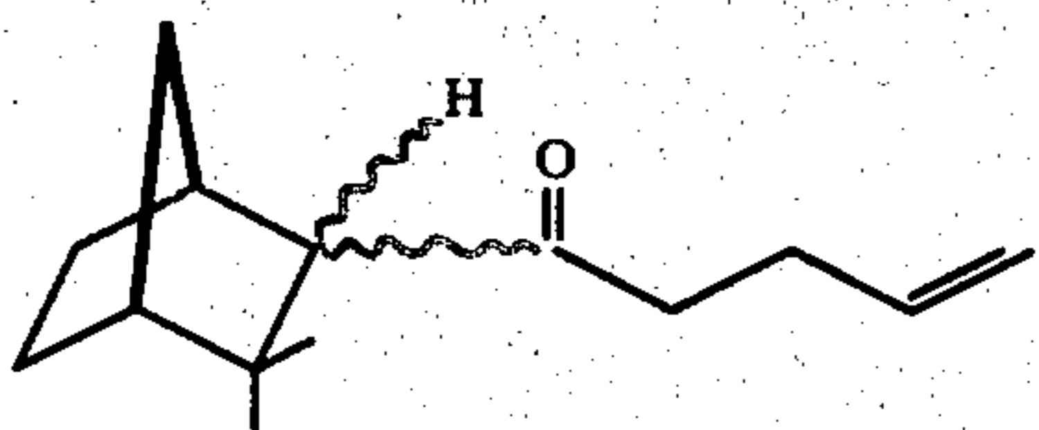
FIG. 39 is the Infrared spectrum for the compound produced in Part B of Example XXV having the structure:
