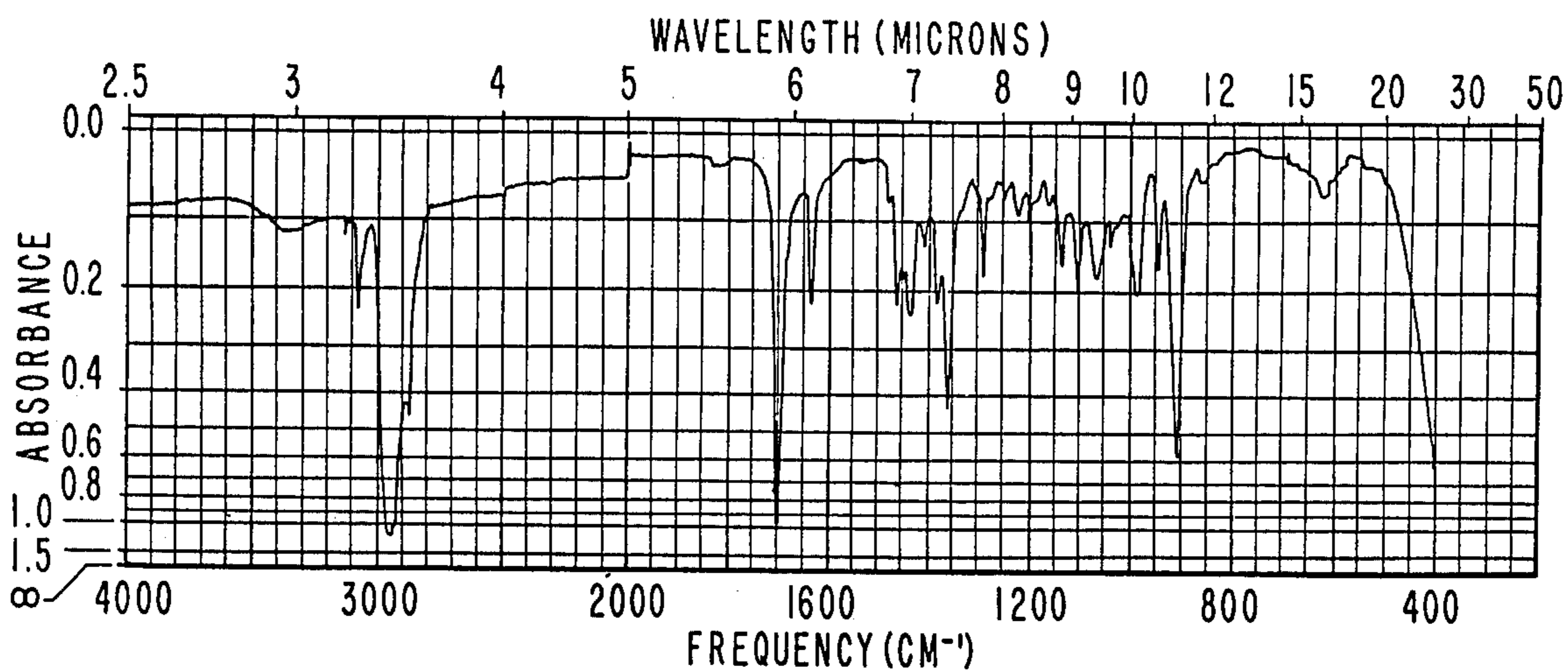
I R SPECTRUM FOR EXAMPLE XXIV
