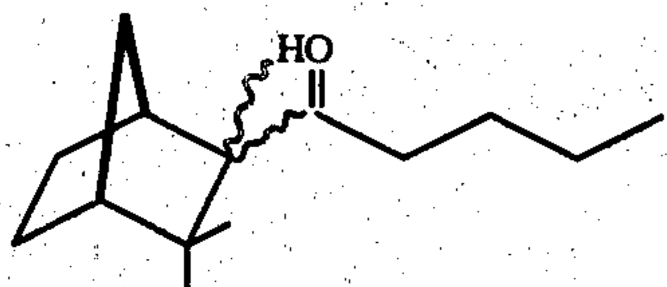
FIG. 41 is the Infrared spectrum for the compound having the structure:
