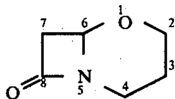
O-Cephem
