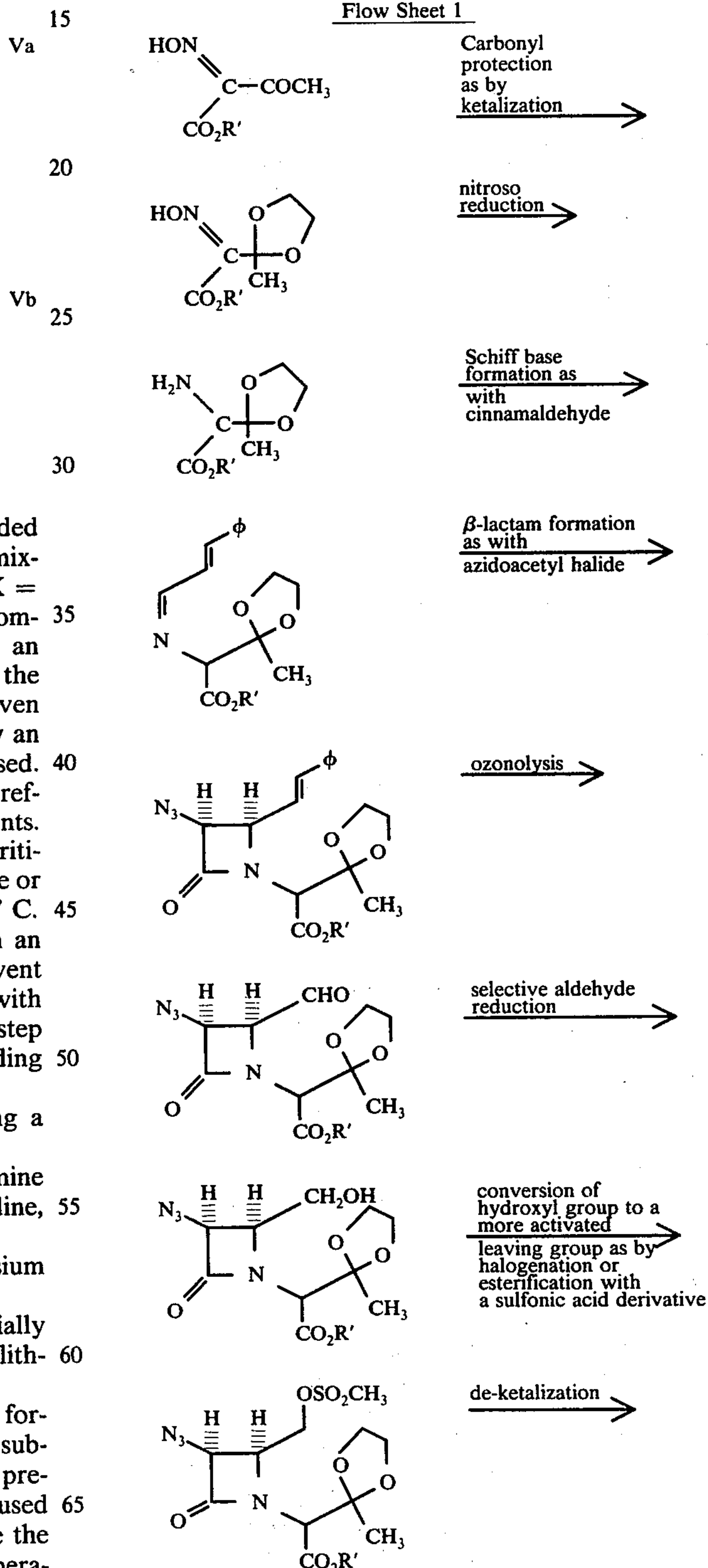
Flow Sheet 1
