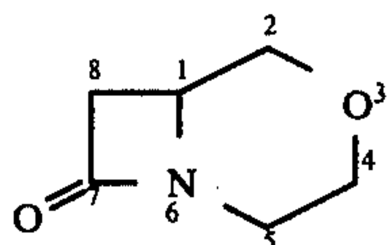
3-oxa-6-aza-bicyclo-[4,2,0]octan-7-one.
