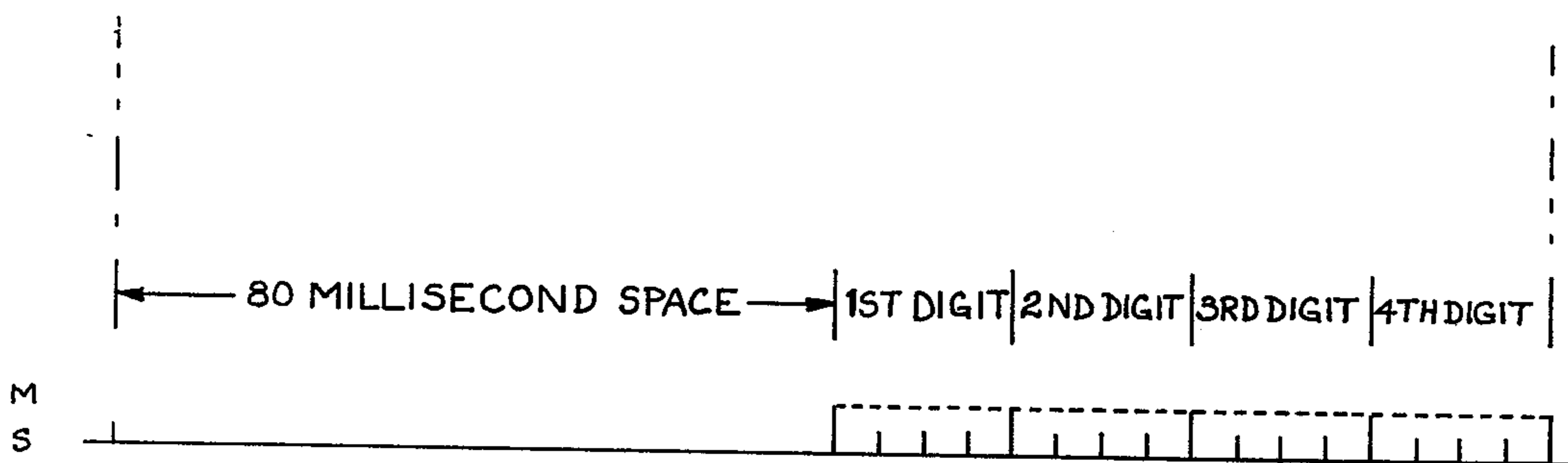
FIG. 2C. ID SIGNALLING FROM MOBILE-TO-BASE
