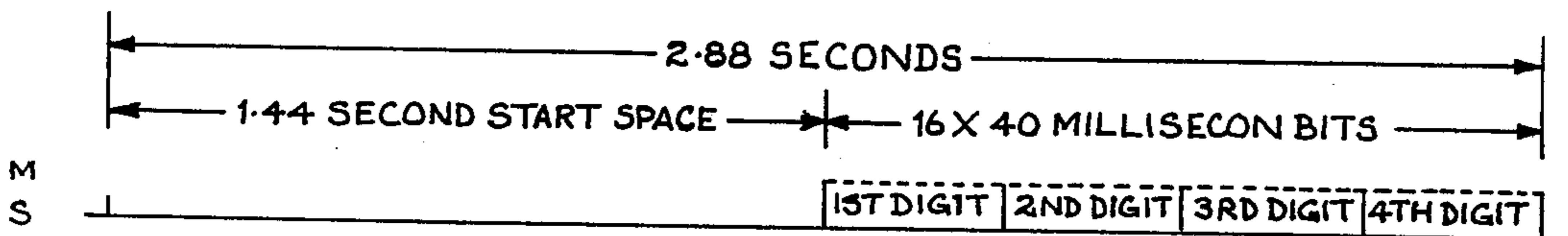
FIG. 2D. BASE STATION CALL SIGN
