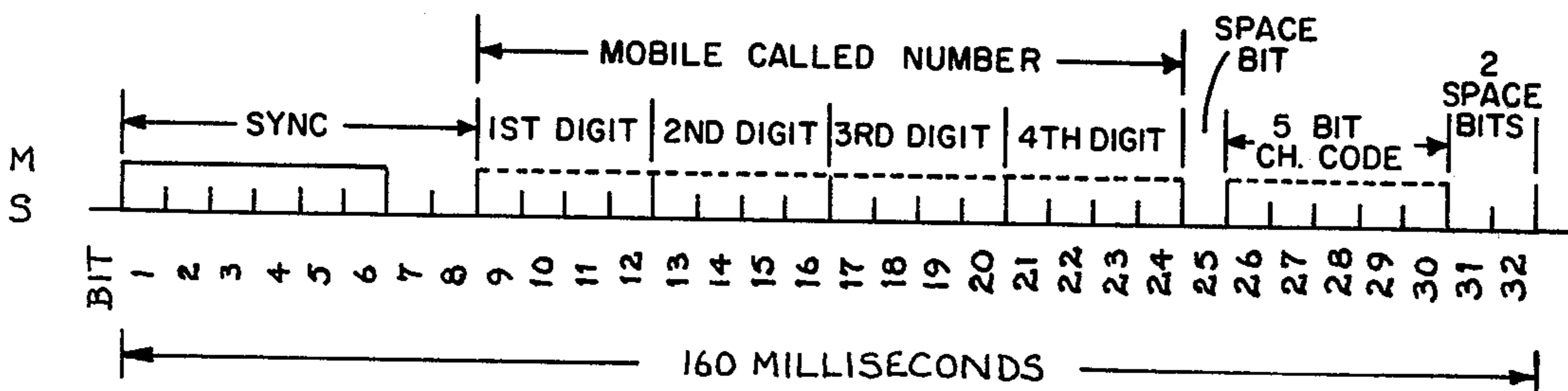
FIG. 2A. CALL SIGNALLING BASE-TO-MOBILE AT 200 BAUDS
