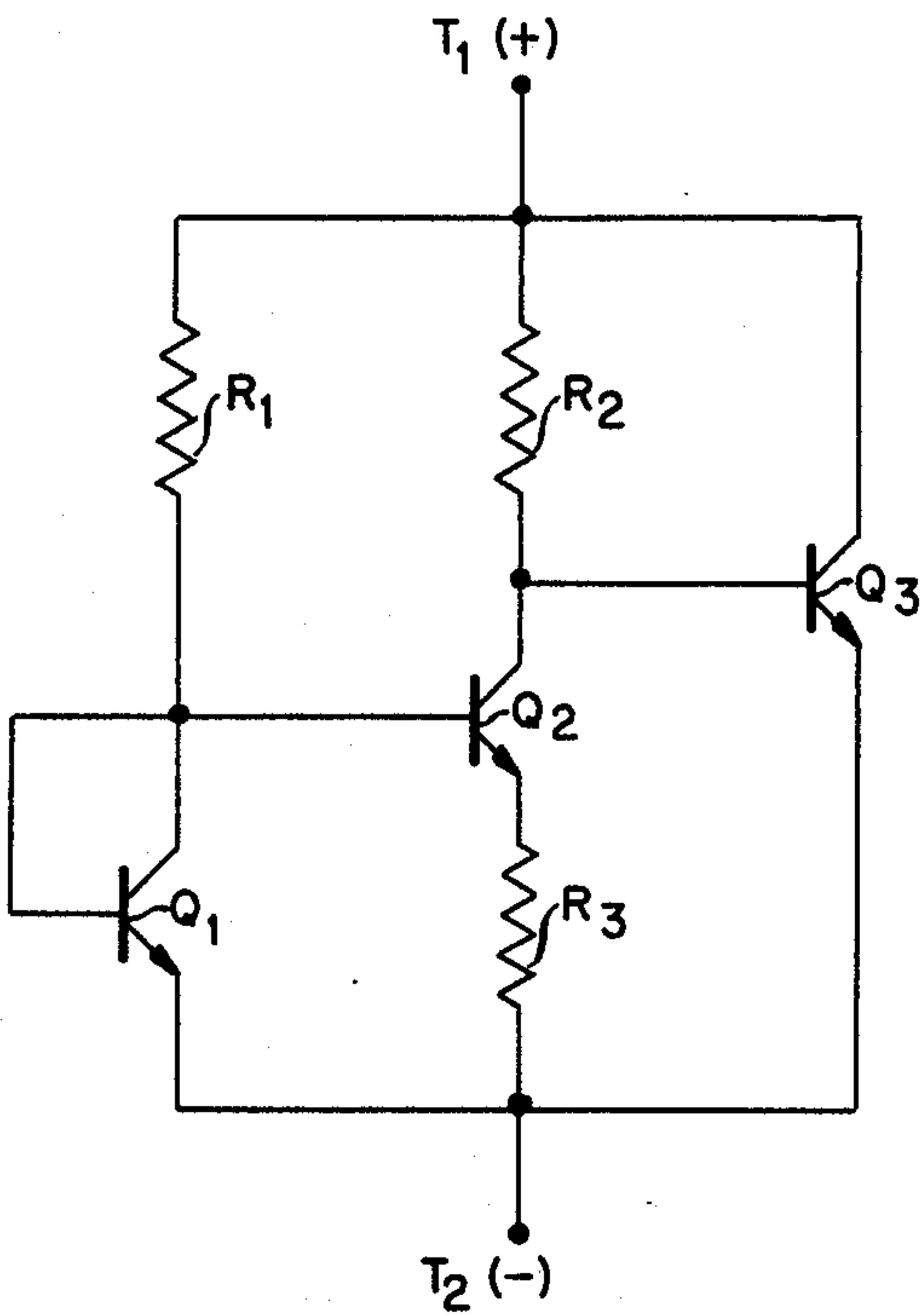
FIG. 1 (PRIOR ART)
